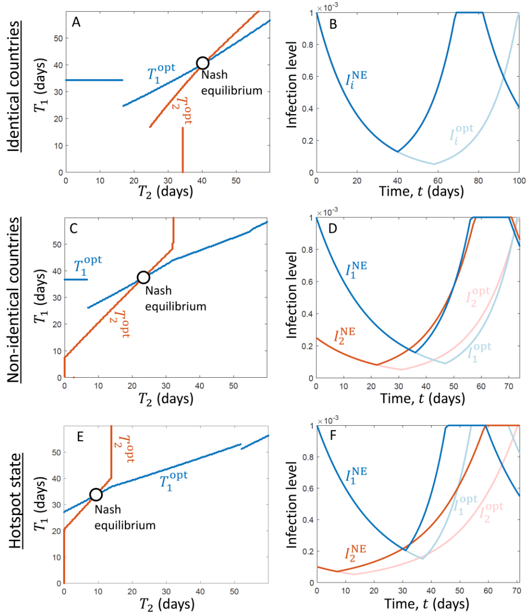
122 Figure 2: The equilibrium solution dictates that governments release the quarantines earlier 123 than optimal. We consider the three cases illustrated in Fig. 1: identical countries (A, B), non- 124 identical countries (C, D), and a state that initially has a much higher infection level than the rest 125 of the U.S. (E, F). The left column (A, C, E) shows the optimal time for country 1 to release the 126 quarantine, T_1^{\text{opt}} , as a function of the day when country 2 releases the quarantine, T_2 (blue line). 127 It also shows the optimal time for country 2 to release the quarantine, T_2^{\text{opt}} , as a function of the 128 day when country 1 releases the quarantine, T_1 , on a flipped axis (mirror image, red line). The 129 intersection of the blue and the red line indicates the open-loop Nash equilibrium. In turn, the 130 right column (B, D, E) shows the time evolution of the infection level in countries 1 and 2, 131 assuming that they adopt the Nash equilibrium strategies ( I_1^{\text{NE}} , blue line, and I_2^{\text{NE}} , red line), as
