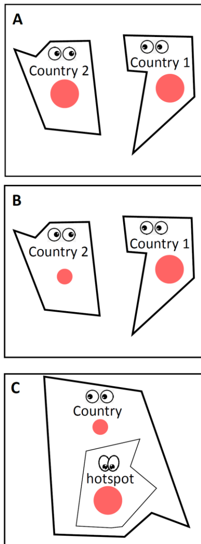
118 Figure 1: Illustration of the three cases that we consider. (A) Case 1: Both countries have the 119 same population size and infection level. (B) Case 2: Both countries have the same population 120 size, but country 1 has a more severe outbreak. (C) Case 3: One U.S. state is a “hotspot” and has 121 a more severe outbreak than the rest of the U.S.
