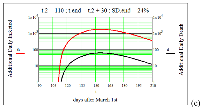
Figure 8. The sequence of figures demonstrates effects of releasing the 48% social distancing set constant from day - 22 nd . Selected values: t_2 - beginning progressive SD release; t_{end} - end SD release, final SD = 24%. The sequence forecasts additional daily numbers of symptomatic infected (red line), and additional deaths (black line).
