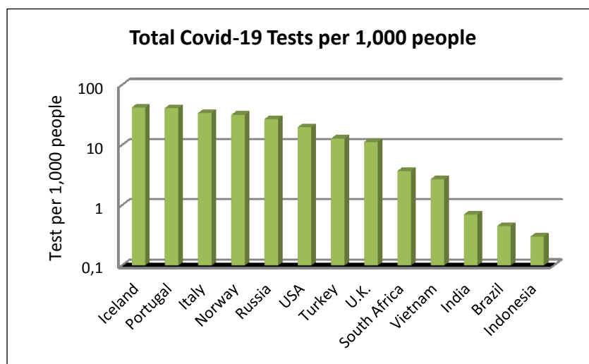
Figure 1. Data (relative to May, 1 st ) collected from www.ourworldindata.org [1].
