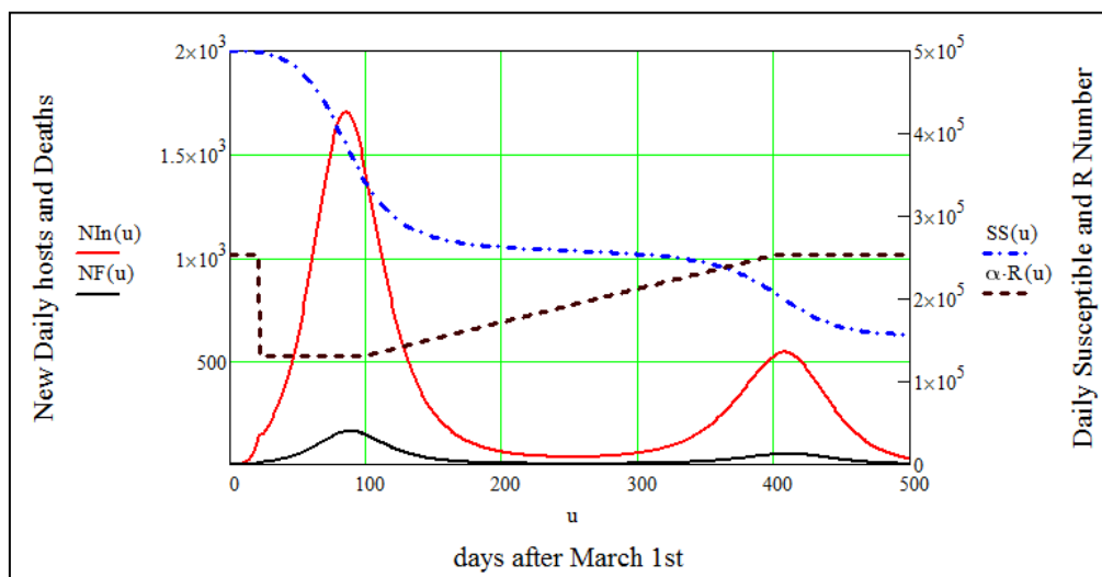
Figure 9. Result of the MP release over a longer period of time. Simulation by a progressive SD release, starting by the end of the third month, and ending ten months later, as shown by R(t) .
