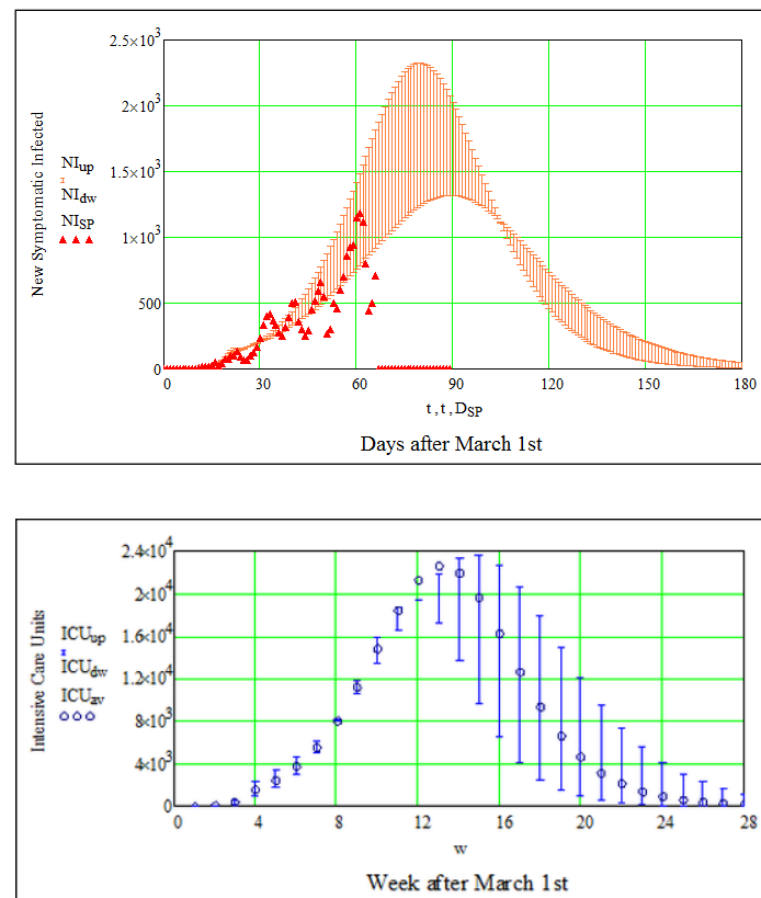
Figure 6. Data on the daily number of new symptomatic infected compared to predictions of the SEIRD model (a). The large data scattering on day to day-plus differences comes from the available reported cases. The number of Intensive Care Units (ICU) was estimated to be proportional to the weekly number of symptomatic infected (b). Permanence of SD after day 22 nd was assumed. Error bars account for the RMS values on the SEIRD parameters.
