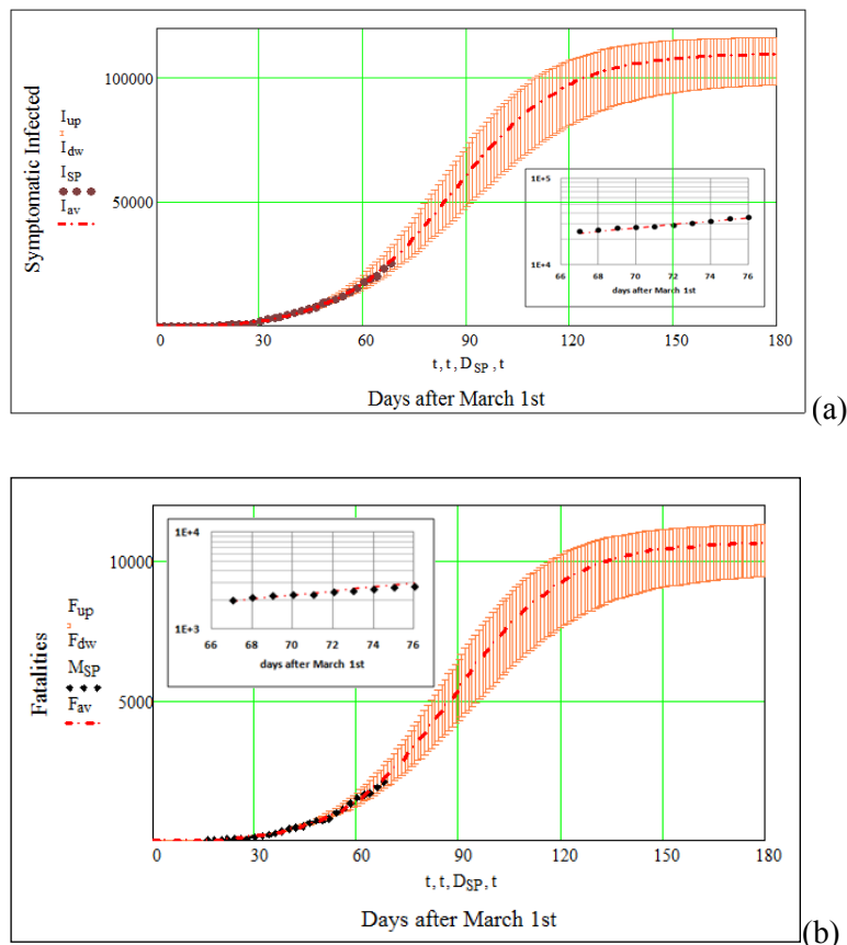
Figure 5. Official data on symptomatic infected individuals (a), and fatalities (b) are shown by black circles, and diamonds respectively. Error bars account for the RMS values on the SEIRD parameters. The fitting values to SEIRD model shown by red dashed line and error bars are: R_o = 2.53 \pm 0.09 , \beta_o = 0.913 \pm 0.018 , \gamma = 0.316 \pm 0.01 , \mu = 0.017 , \psi_o = 0.525 \pm 0.03 , \sigma_o = 0.50 \pm 0.02 , and t_{SD} = 22 days. The mean fitting to the infected individuals (logarithmic scale) presents standard deviation SD = 0.05 and root mean square RMS = 0.07 . Data points for the last 10 days (inserts) were added after the model was complete, granting confidence on outcomes.
