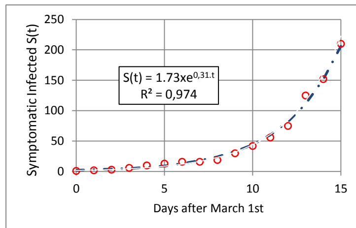
Figure 2. Exponential fitting of the initial growth of symptomatic infect people. The growth rate r = 0.31 \pm 0.02 was estimated applying the Levenberg-Marquardt method.
