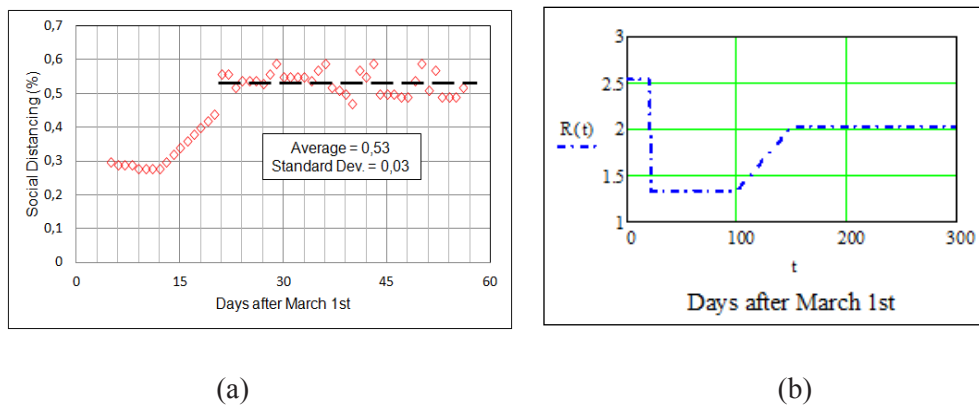
Figure 4. Quantification of the MP application on the city of S. Paulo by Social Distancing (SD) measures (a), Reproductive Basic Number R(t) modeling the Social Distancing effective change after March 22 nd (b). Blue point and dashed line represent the progressive return to R_o after day 100.
