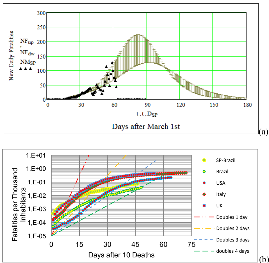
Figure 7. (a) Data on daily new fatalities is compared to model prediction. Keeping the MP as modeled after March 22 nd . The RMS values to SEIRD model are shown by black error bars. The maximum number of new daily fatalities is predicted to happen by the last week of May 2020. (b) Number of fatalities per thousand inhabitants reported from other countries. The fatality rise in the city of S. Paulo is shown for comparison.
