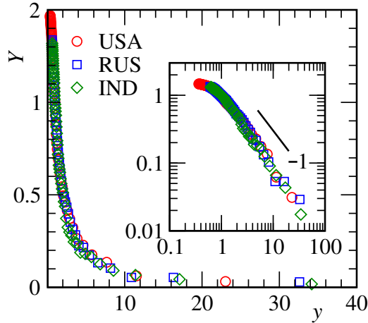
FIG. 2. Finite-size scaling analysis, i.e., Y versus y plots, to understand the spread of COVID-19. Data from all the considered countries have been included. See text for the values of m and n_d that were used to obtain the data collapse. The main frame and the inset show the same plots on linear and log scales. The solid line in the inset is a power-law. The value of the exponent has been mentioned next to it.
