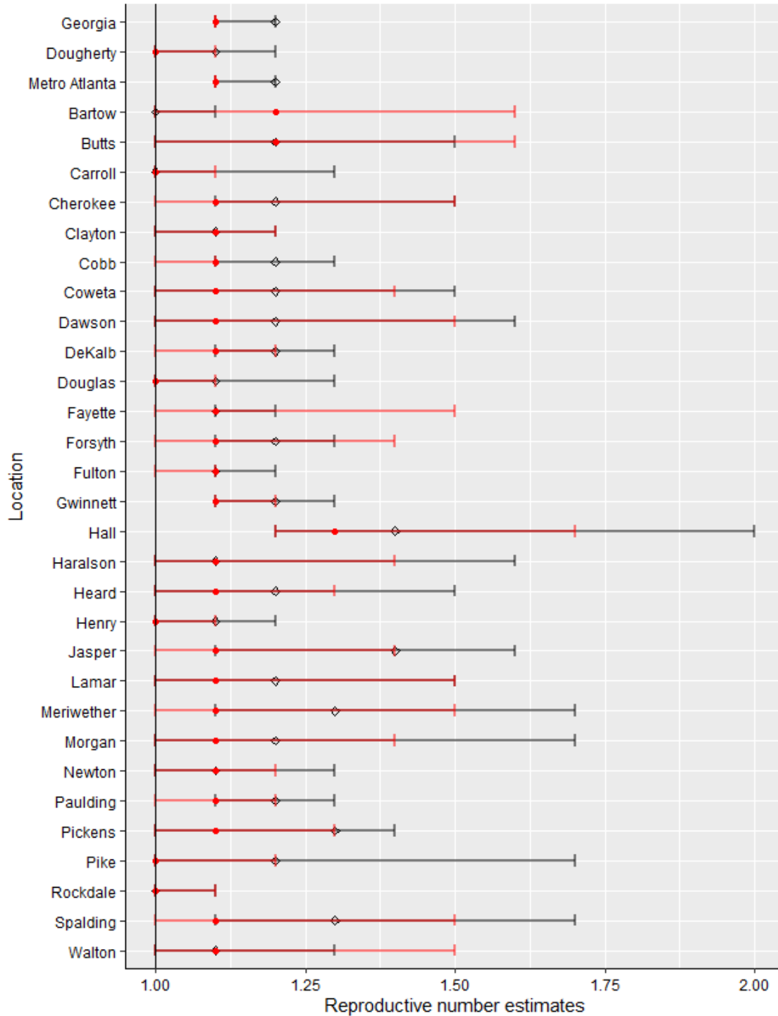
Figure 2. Effective reproductive number estimates calculated using the Generalized Growth Model method for Georgia, USA up to May 2, 2020. Estimates for the growth rate with data collected up to April 18, 2020 (black diamonds and black lines) and data analyzed up to May 2, 2020 (red circles and red lines). The vertical black line highlights where the Re = 1 .
