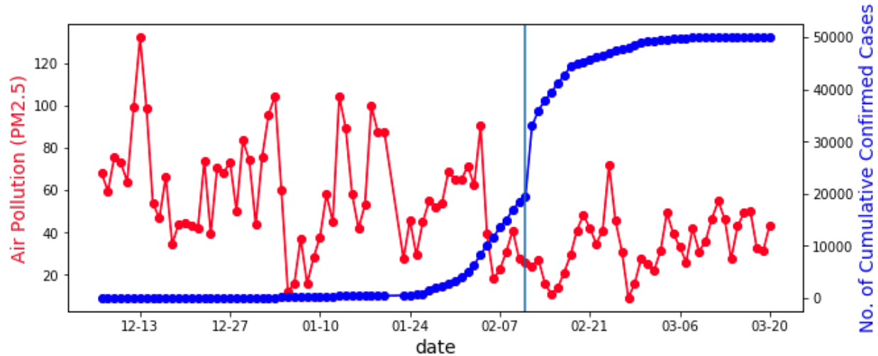
Figure 1. The cumulative number of confirmed cases vs. the air pollutant concentration (PM 2.5 ) in Wuhan, China
