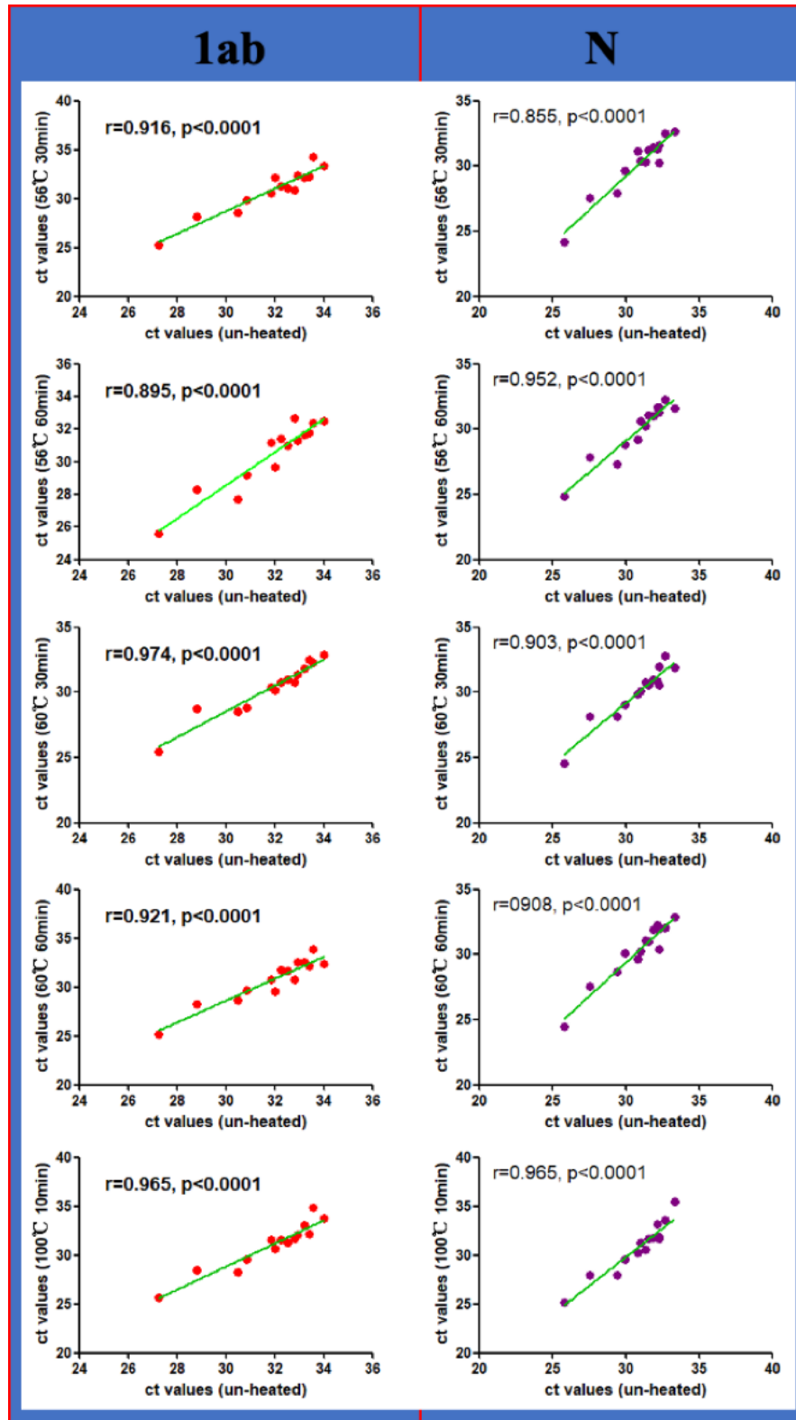
Fig 1. Spearman correlation analysis of The Ct values for ORF1a/b and N between Inactivated and non-Inactivated Samples
