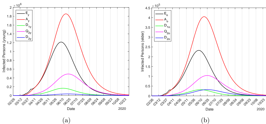
Figure 16: All persons harboring the new coronavirus ( E_j , A_j , D_{1j} , Q_{2j} and D_{2j} ), for young ( j = y ) (a) and elder ( j = o ) (b) persons.
