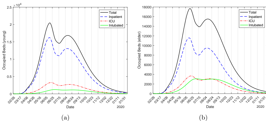
Figure 28: The number of occupied beds due to CoViD-19 by young ( j = y ) (a) and elder ( j = o ) (b) for inpatients ( B_{1j} ), ICU ( B_{2j} ) and ICU/intubated ( B_{3j} ) persons. Strategy B with \varepsilon = 0.2 , release beginning on June 15.
