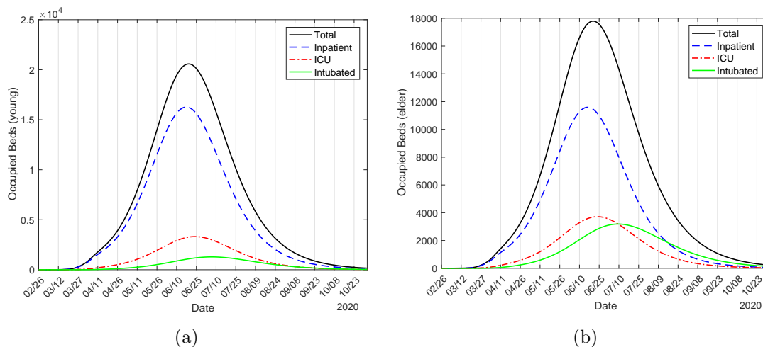
Figure 12: The number of beds occupied by young ( j = y ) (a) and elder ( j = o ) (b) persons in hospital ( B_{1j} ), ICU ( B_{2j} ) and ICU/intubated ( B_{3j} ).
