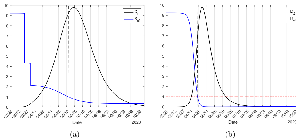
Figure 11: Illustration of the effective reproduction number R_{ef} when isolation and protection are adopted (a) and without adoption (b), with the actual value of curve D_2 must be multiplied by, respectively, 7,000 (a) and 40,000 (b).
