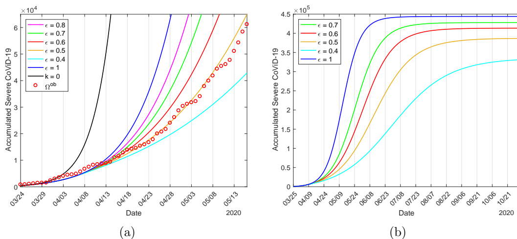
Figure 7: The curves of D_2 = D_{2y} + D_{2o} and observed data, where \beta'_y = 0.8\beta_y = 0.648 , 0.7\beta_y = 0.567 , 0.6\beta_y = 0.486 , 0.5\beta_y = 0.405 and 0.4\beta_y = 0.324 , plus \beta'_y = 1 and without isolation (a), and extended curves of D_2 for 4 different decreasing values of transmission rates plus \beta'_y = 1 (b).
