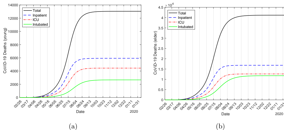
Figure 23: The number of deaths due to CoViD-19 by young ( j = y ) (a) and elder ( j = o ) (b) for inpatient ( \Pi_{1j} ), ICU ( \Pi_{2j} ) and ICU/intubated ( \Pi_{3j} ) persons. Strategy A with \varepsilon = 0.5 , release beginning on June 1.
