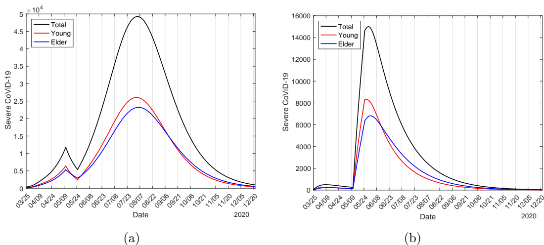
Figure 20: The curves of D_{2y} , D_{2o} , and D_2 among circulating (a) and isolated (b) persons, assuming that among isolated persons, \varpi = 10 (low transmission) and \varepsilon = 1.0 (without protection).
