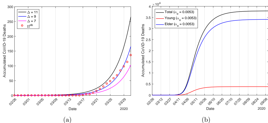
Figure 4: The estimated curve of \Pi and the observed data for R_0 = 9.239 (a), and the accumulated number of CoViD-19 deaths ( \Pi_y , \Pi_o , and \Pi = \Pi_y + \Pi_o ) (b).
