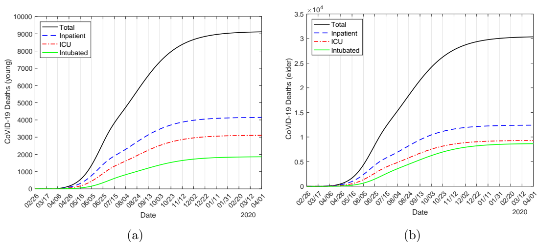
Figure 33: The number of deaths due to CoViD-19 by young ( j = y ) (a) and elder ( j = o ) (b) for inpatient ( \Pi_{1j} ), ICU ( \Pi_{2j} ) and ICU/intubated ( \Pi_{3j} ) persons. Strategy C with \varepsilon = 0.2 , release beginning on June 23.
