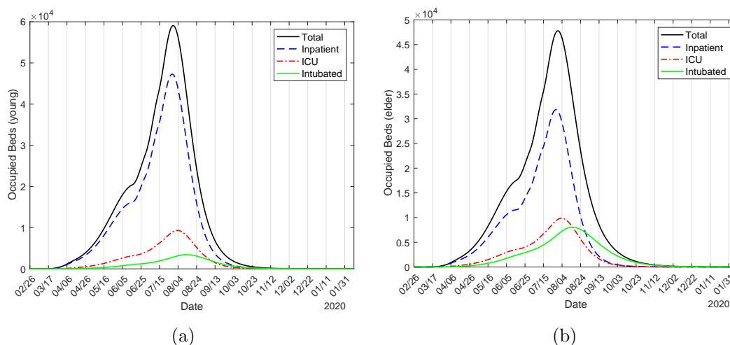
Figure 26: The number of occupied beds due to CoViD-19 by young ( j = y ) (a) and elder ( j = o ) (b) for inpatients ( B_{1j} ), ICU ( B_{2j} ) and ICU/intubated ( B_{3j} ) persons. Strategy B with \varepsilon = 0.5 , release beginning on June 15.
