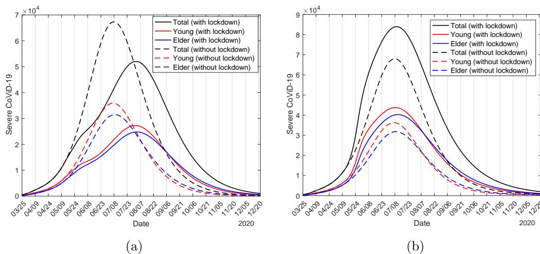
Figure 21: The curves of D_{2y} , D_{2o} and D_2 with (continuous) and without (dashed) lockdown for \varpi = 10 (low transmission) (a), and \varpi = 5 (medium transmission) and (b), using \varepsilon = 0.5 for circulating and \varepsilon = 1 for isolated persons.
