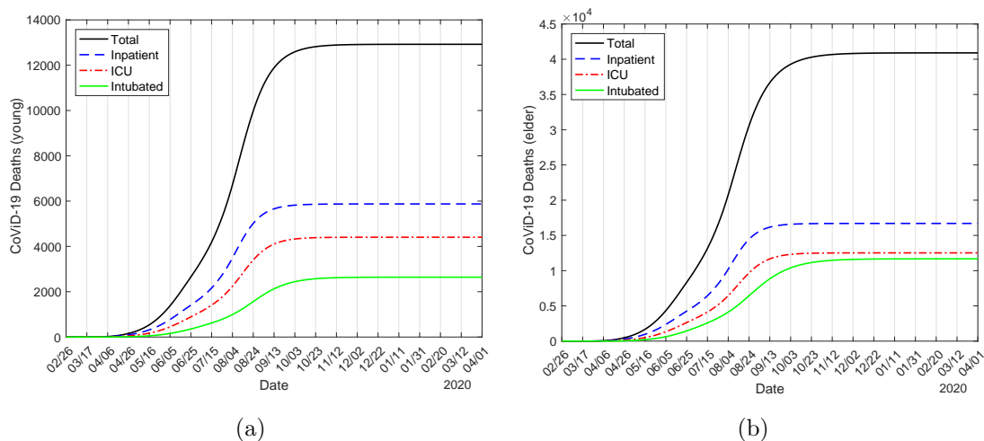
Figure 31: The number of deaths due to CoViD-19 by young ( j = y ) (a) and elder ( j = o ) (b) for inpatient ( \Pi_{1j} ), ICU ( \Pi_{2j} ) and ICU/intubated ( \Pi_{3j} ) persons. Strategy C with \varepsilon = 0.5 , release beginning on June 23.
