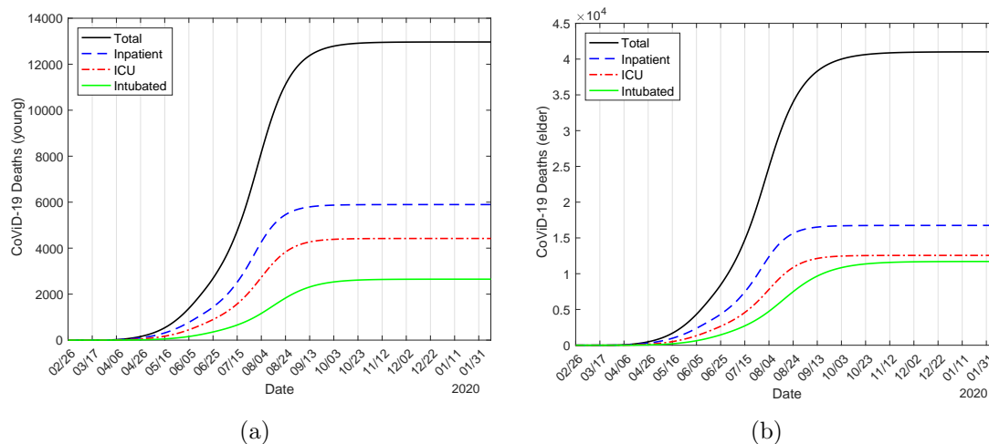
Figure 27: The number of deaths due to CoViD-19 by young ( j = y ) (a) and elder ( j = o ) (b) for inpatient ( \Pi_{1j} ), ICU ( \Pi_{2j} ) and ICU/intubated ( \Pi_{3j} ) persons. Strategy B with \varepsilon = 0.5 , release beginning on June 15.
