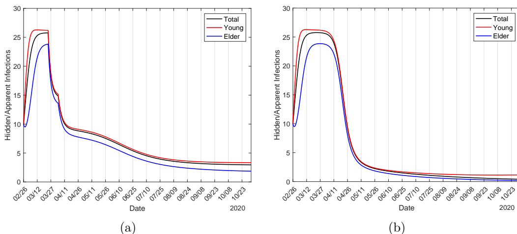
Figure 17: The ratio hidden:apparent based on Figure 16, calculated based on the ratio (E + A + D_1) : (Q_2 + D_2) . The ratio hidden:apparent when there is not any intervention is shown (b).
