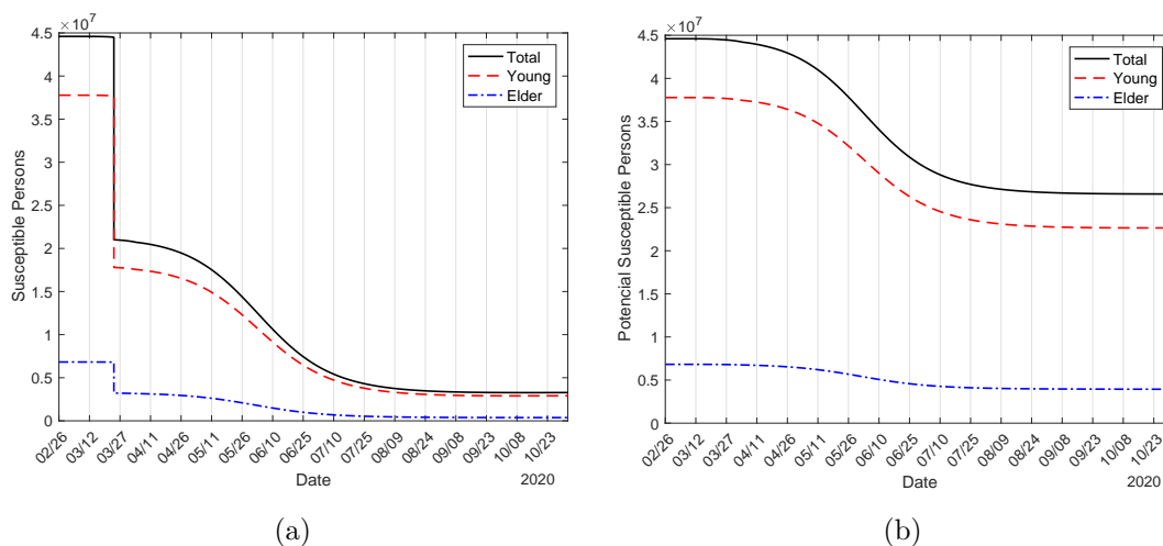
Figure 10: The circulating susceptible persons S_y , S_o and S = S_y + S_o (a), and potential susceptible persons to be infected S_y^{tot} , S_o^{tot} and S^{tot} = S_y^{tot} + S_o^{tot} (b).
