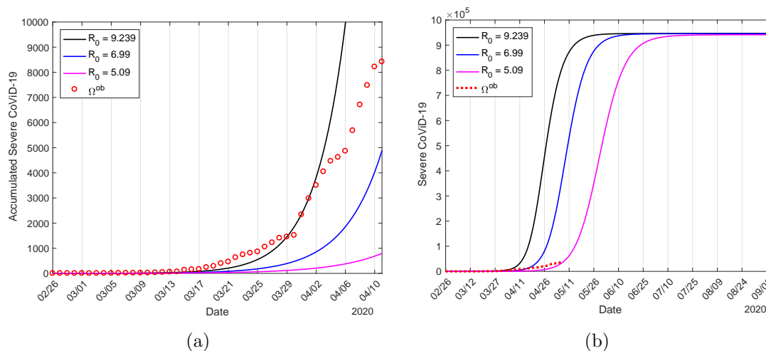
Figure 3: The estimated curve of D_2 and observed data, plus two curves with lower transmission rates: \beta_y = 0.59 and \beta_o = 0.679 ( days^{-1} ), with R_0 = 6.99 , and \beta_y = 0.43 and \beta_o = 0.495 ( days^{-1} ), with R_0 = 5.09 (a); and extended curves of accumulated number of severe CoViD-19 \Omega (b).
