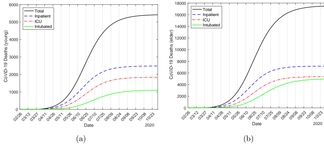
Figure 13: The number of deaths due to CoViD-19 by young ( j = y ) (a) and elder ( j = o ) (b) persons in hospital ( \Pi_{1j} ), ICU ( \Pi_{2j} ) and ICU/intubated ( \Pi_{3j} ).
