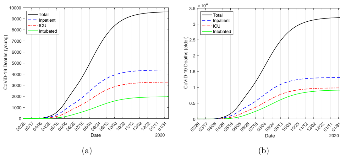
Figure 25: The number of deaths due to CoViD-19 by young ( j = y ) (a) and elder ( j = o ) (b) for inpatient ( \Pi_{1j} ), ICU ( \Pi_{2j} ) and ICU/intubated ( \Pi_{3j} ) persons. Strategy A with \varepsilon = 0.2 , release beginning on June 1.
