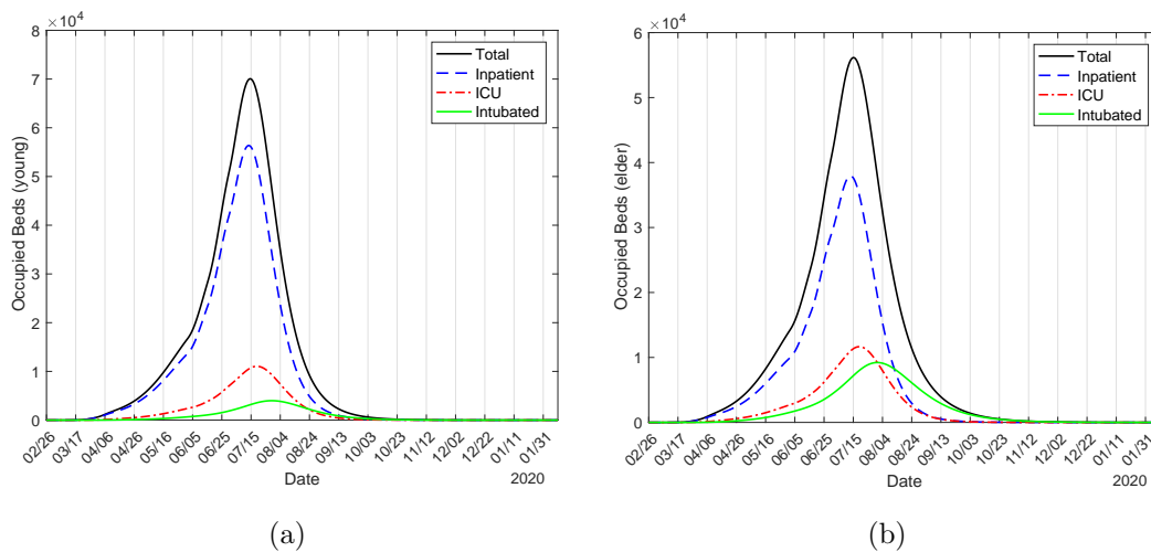
Figure 22: The number of occupied beds due to CoViD-19 by young ( j = y ) (a) and elder ( j = o ) (b) for inpatients ( B_{1j} ), ICU ( B_{2j} ) and ICU/intubated ( B_{3j} ) persons. Strategy A with \varepsilon = 0.5 , release beginning on June 1.
