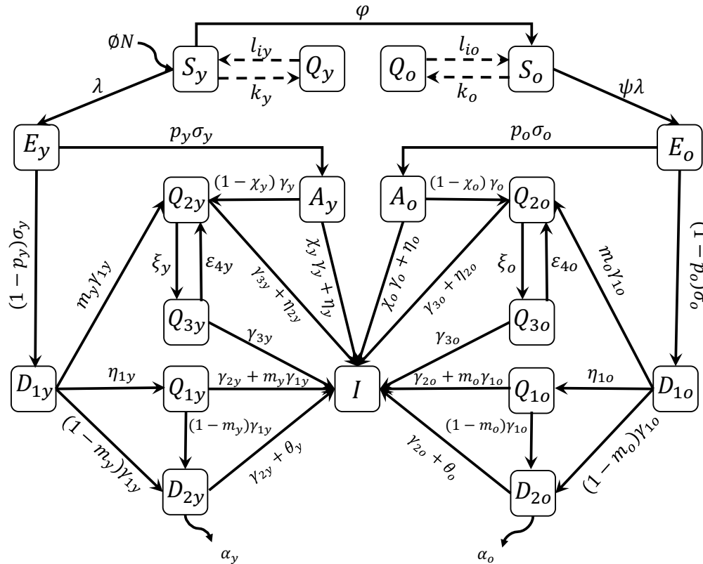
Figure 1: The flowchart of new coronavirus transmission model with variables and parameters.
