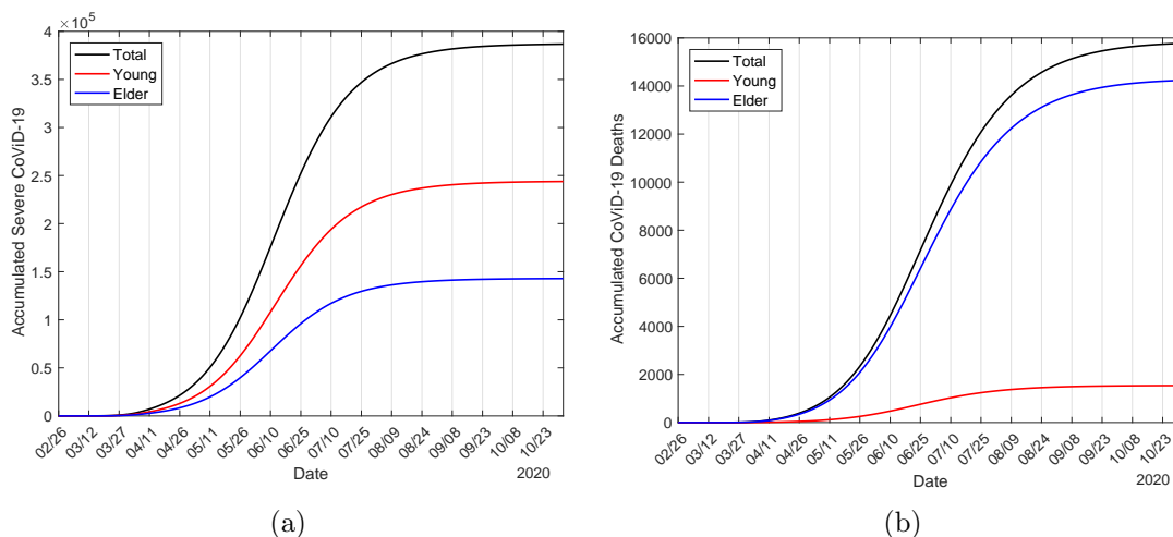
Figure 8: The estimated curves of \Omega_y , \Omega_o , and \Omega = \Omega_y + \Omega_o (a) and \Pi_y , \Pi_o , and \Pi = \Pi_y + \Pi_o (b), for k = 0.528 and \varepsilon = 0.6 . The reduced transmission rates are \beta'_y = 0.486 and \beta'_o = 0.559 , with R_0 = 5.76 .
