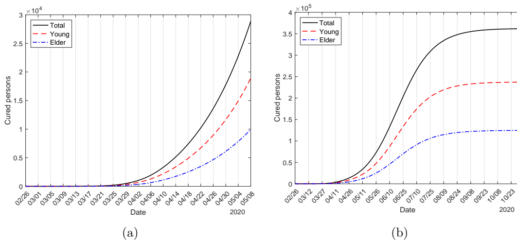
Figure 14: The numbers of cured young, elder and total persons from CoViD-19 (a), and extended curves (b).
