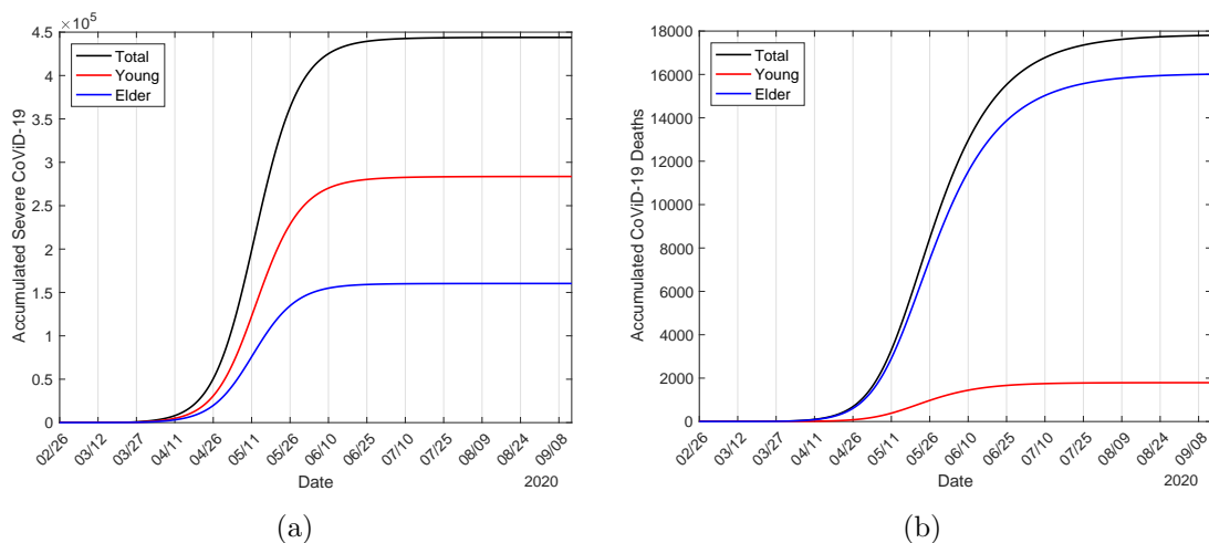
Figure 6: The estimated curves of \Omega_y , \Omega_o , and \Omega = \Omega_y + \Omega_o (a), and \Pi_y , \Pi_o , and \Pi = \Pi_y + \Pi_o (b), for k = 0.528 .
