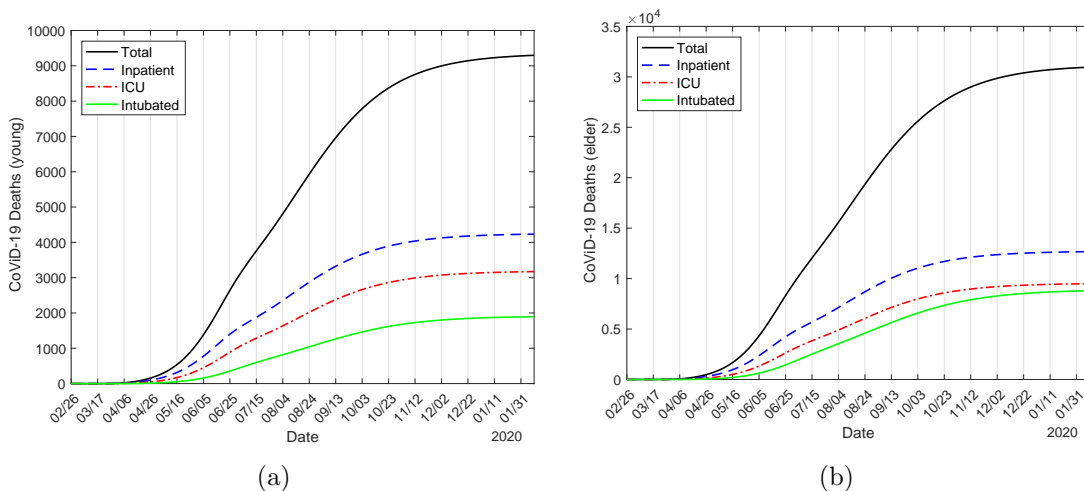
Figure 29: The number of deaths due to CoViD-19 by young ( j = y ) (a) and elder ( j = o ) (b) for inpatient ( \Pi_{1j} ), ICU ( \Pi_{2j} ) and ICU/intubated ( \Pi_{3j} ) persons. Strategy B with \varepsilon = 0.2 , release beginning on June 15.
