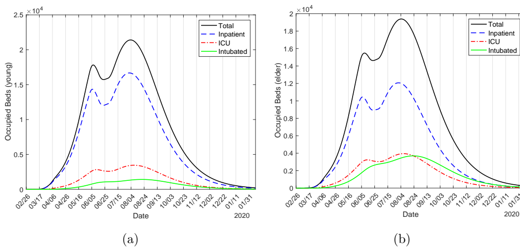
Figure 24: The number of occupied beds due to CoViD-19 by young ( j = y ) (a) and elder ( j = o ) (b) for inpatients ( B_{1j} ), ICU ( B_{2j} ) and ICU/intubated ( B_{3j} ) persons. Strategy A with \varepsilon = 0.2 , release beginning on June 1.
