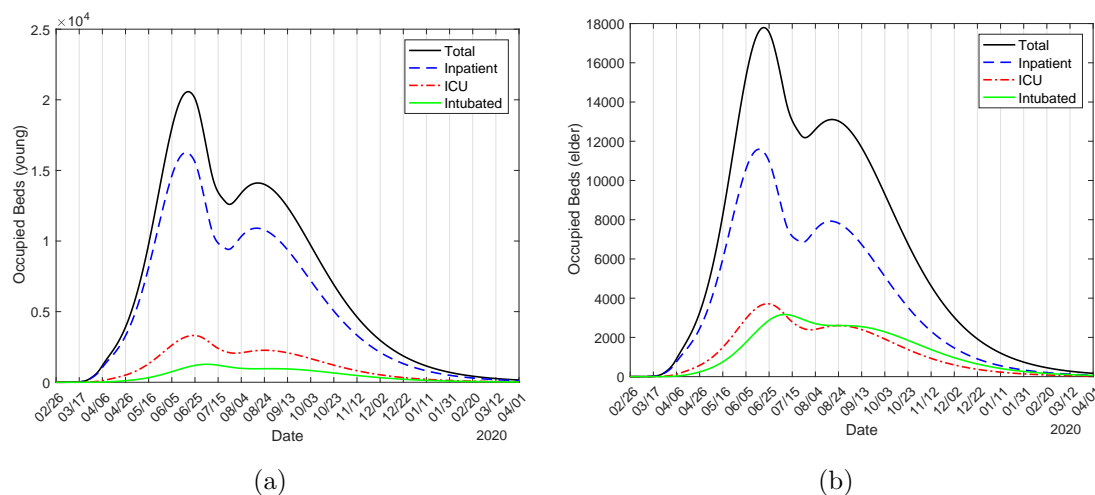
Figure 32: The number of occupied beds due to CoViD-19 by young ( j = y ) (a) and elder ( j = o ) (b) for inpatients ( B_{1j} ), ICU ( B_{2j} ) and ICU/intubated ( B_{3j} ) persons. Strategy C with \varepsilon = 0.2 , release beginning on June 23.
