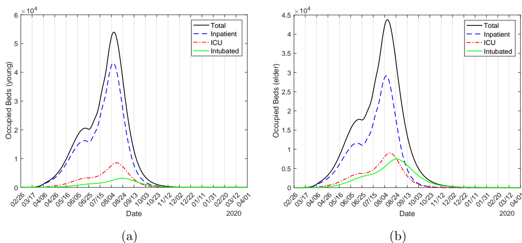
Figure 30: The number of occupied beds due to CoViD-19 by young ( j = y ) (a) and elder ( j = o ) (b) for inpatients ( B_{1j} ), ICU ( B_{2j} ) and ICU/intubated ( B_{3j} ) persons. Strategy C with \varepsilon = 0.5 , release beginning on June 23.
