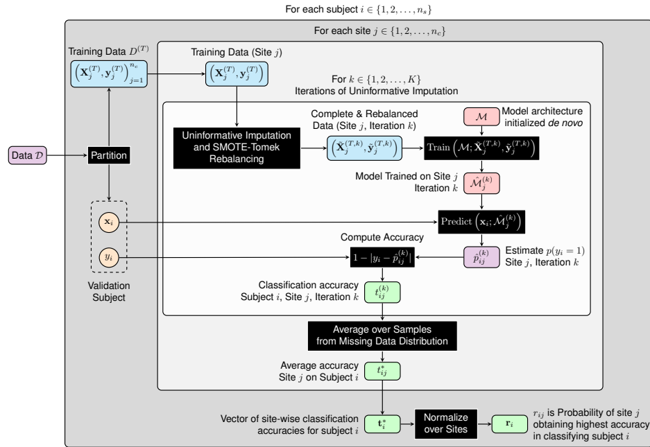
Figure 3. Illustration of the algorithm for the predict every subject out protocol.
