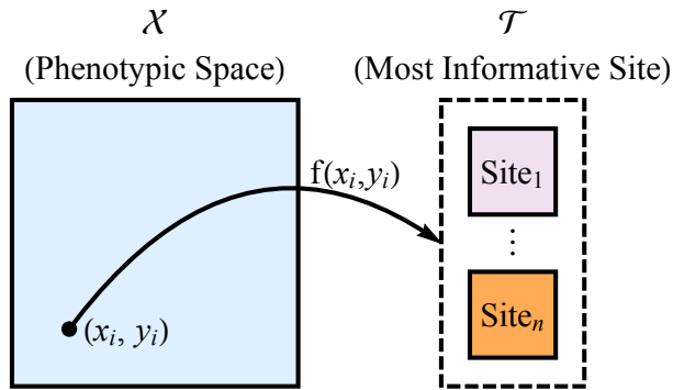
Figure 2. Representation of the mapping from phenotypic space \mathcal{X} onto the representation of “most informative site-level model” ( \mathcal{T} ). The transformation function is the normalized accuracy score for a classification model trained on each site’s data individually (Equation 2).
