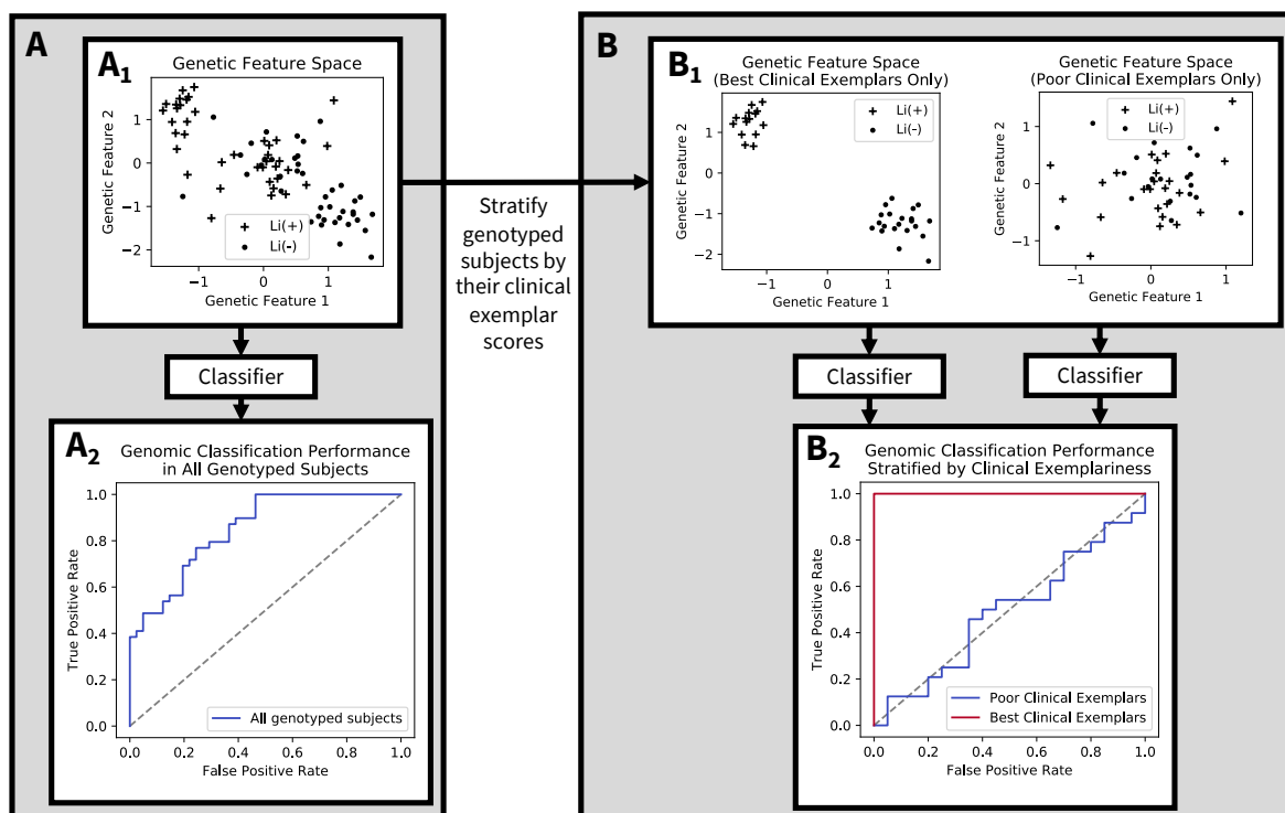
Figure 4. Hypothetical illustration of Part 2 of this study’s analysis, which evaluates the degree to which stratification of genomic data by corresponding subjects’ clinical exemplar scores can improve genomic classification performance. Panel A: Subjects’ genotypes lie on a genotypic feature space (shown in Panel A 1 as a simplified 2 dimensional plane). Panel A 2 shows a hypothetical ROC curve for these aggregated data. Panel B: Each genotyped subject has an exemplar score computed from Part 1 of the present study. Recall that the exemplar score merely identifies the degree to which a subject’s clinical profile (i.e. symptoms, family history, comorbidities, etc.) is reliably predictive of lithium responsiveness. Panel B 1 shows that the aggregated genotyped sample can then be stratified into the “Best” clinical exemplars (subjects with top 25% of clinical exemplar scores within each of the responder and non-responder groups, respectively), and the “Poor” clinical exemplars (those with the lowest 25% of clinical exemplar scores in each responsiveness class). We then apply classifiers to the genomic data in each of these “Best Exemplar” and “Poor Exemplar” strata, respectively, and compare classification performance (Panel B 2 ). The hypothetical receiver operating characteristic curve in Panel B 2 reflects our hypothesis, that genetic classification of lithium response will be superior among the subgroup of Best clinical exemplars.
