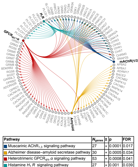
Figure 7. Gene enrichment in the best exemplars. Results of the statistical enrichment test using the logistic regression coefficients from the classifier trained on the best exemplar. Individual genes are shown in gray, with pathway nodes (and edges) colored according to the pathway identity. Pathway names are shown in bold along the perimeter of the graph. Abbreviations: acetylcholine receptor (AChR), G-protein coupled receptor (GPCR), histamine H 1 receptor (H 1 R), false discovery rate (FDR).
