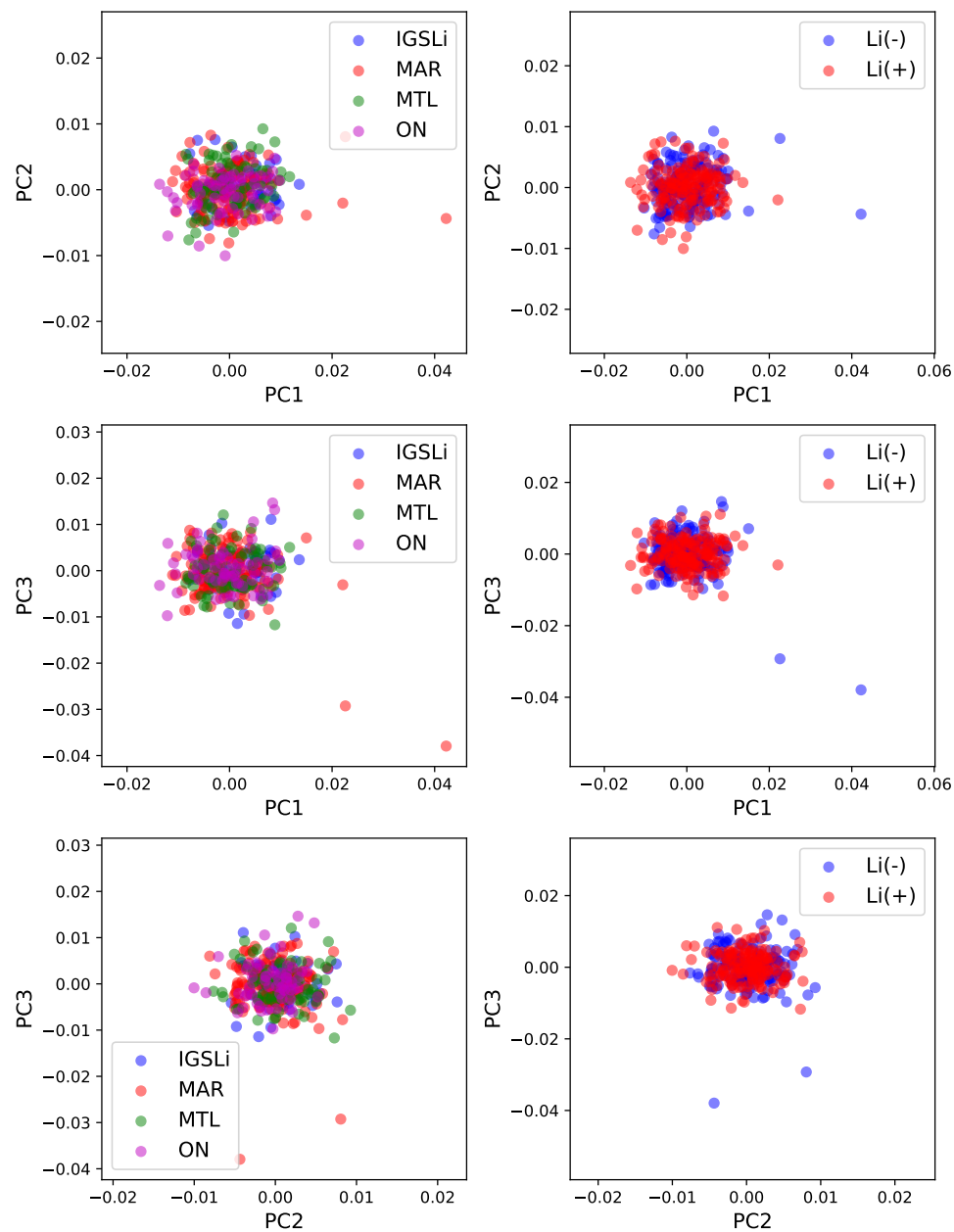
Figure C.1. Principal components analysis of the genomic dataset from Halifax (as coded in the ConLiGen studies [6]). The left column is coloured by the site of origin, whereas the right column of plots is coloured by lithium responsiveness. Abbreviations: International Group for the Study of Lithium (IGSLi), Maritimes (MAR), Montreal (MTL), Ontario (ON; also known as Ottawa/Hamilton).
