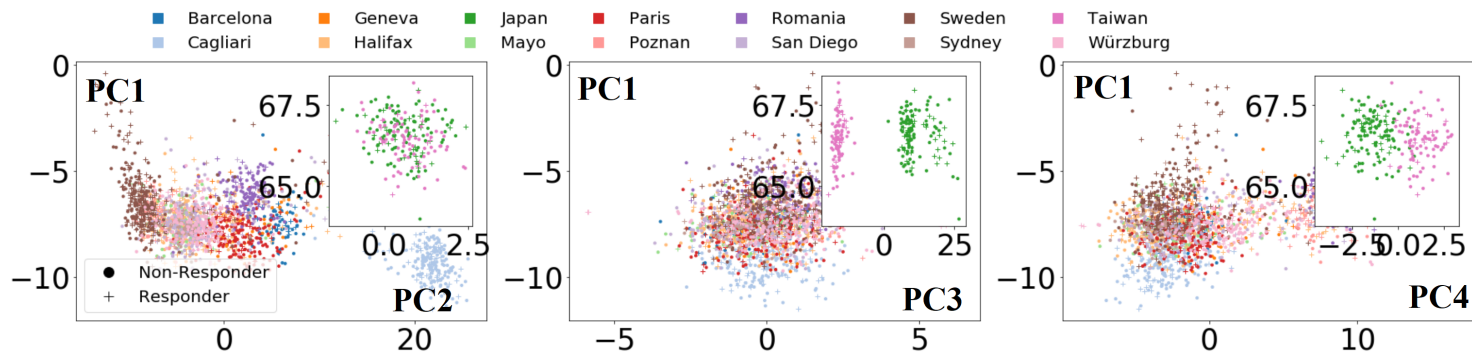
Figure C.2. Principal components analysis of the genomic dataset from the Consortium on Lithium Genetics sample [6] (Figure used with permission from Stone et al., submitted manuscript)
