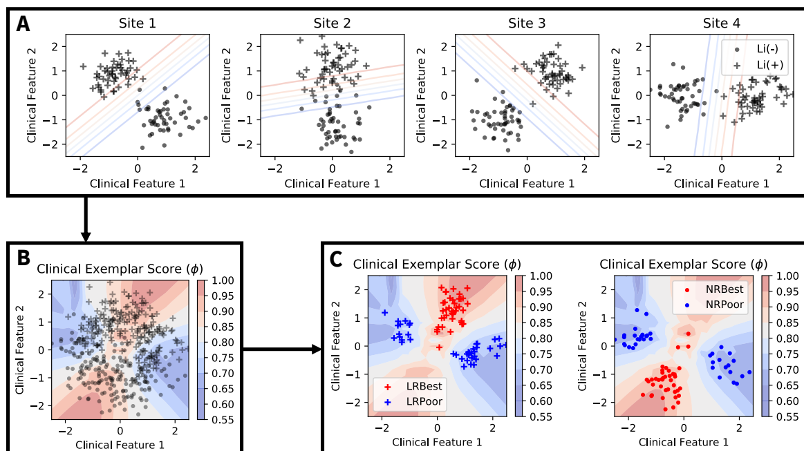
Figure 1. Hypothetical illustration of the clinical exemplar scoring analysis. Note that this part of the analysis is performed using the clinical feature dataset alone. Panel A: Demonstration of heterogeneity in the relationship between lithium responsiveness (depicted as “Li(+)” for responders and “Li(-)” for non-responders) and clinical features across four hypothetical sites. A classifier trained on data from each individual site may yield different discriminative functions. Panel B: Points demonstrate the aggregated dataset (“+” and “-” are responders and non-responders, respectively). Contours demonstrate regions of clinical feature space in which site-level classifiers (from Panel A) agree with high accuracy on the predicted class. An exemplar score can be computed for each subject in the clinical dataset by (1) holding his data out of the training set, (2) predicting his lithium responsiveness using site-level classifiers trained on the remaining subjects, then (3) using the site-wise prediction results to compute the exemplar score. Panel C: Stratification of the clinical dataset according to lithium responsiveness and exemplar score quartile. The “LRBest” and “NRBest” exemplars are those responders and non-responders with exemplar scores above the 75th percentile, respectively. The “LRPoor” and “NRPoor” exemplars are those responders and non-responders with exemplar scores below the 25th percentile, respectively. This stratification can be used to evaluate the clinical features that differentiate good from poor exemplars of lithium response and non-response, respectively.
