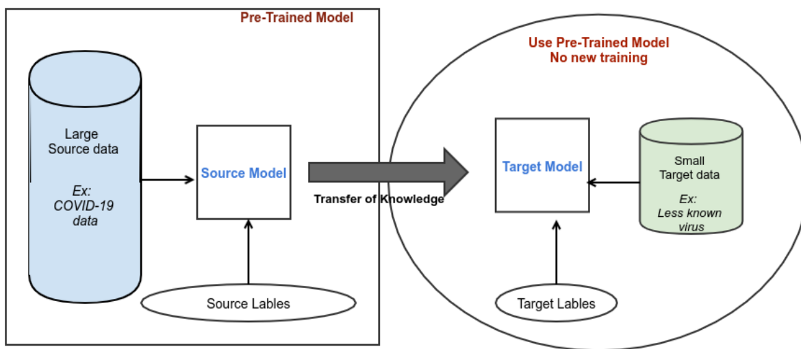
Figure 4a: Typical transfer learning model for future pandemic predictions
