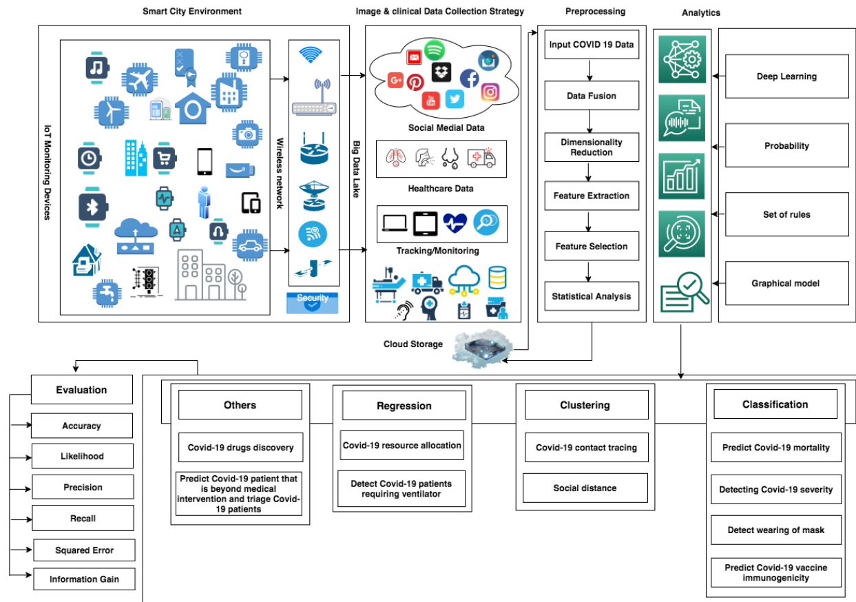
Figure 4: Propose smart city framework integrated with machine learning for fighting COVID-19
