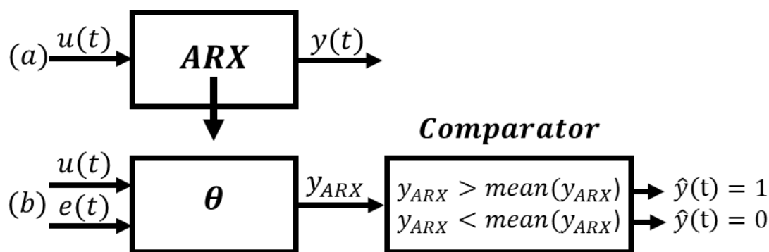
Figure 2. The process of obtaining final output of system: (a) ARX model parameter by training data (b) Output estimation by obtained parameters
