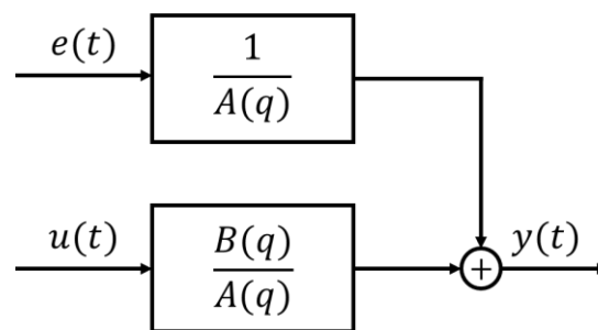
Figure 1. Block diagram of ARX model
