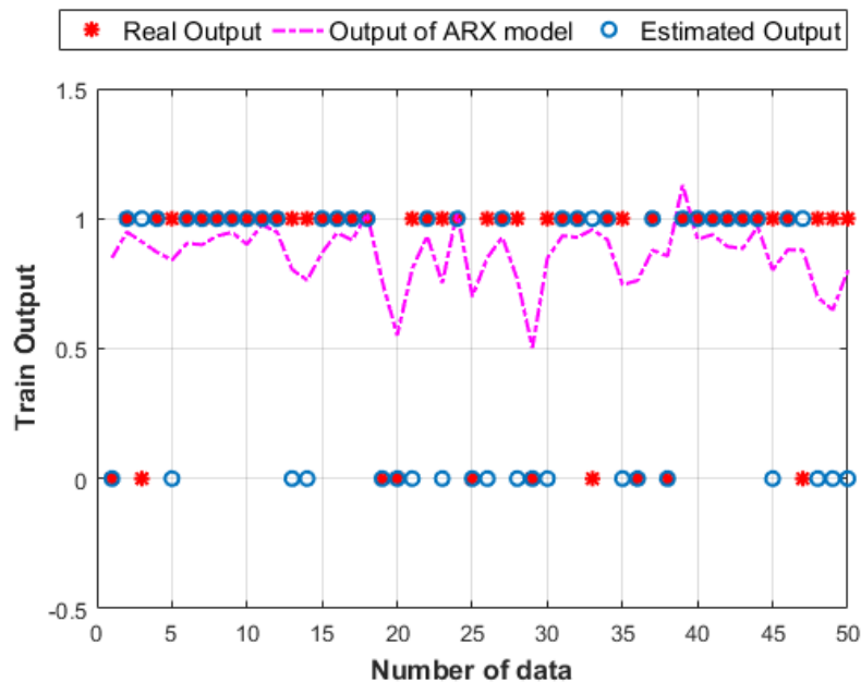
Figure 3. ARX model's output, estimated and actual output of 50 training data
