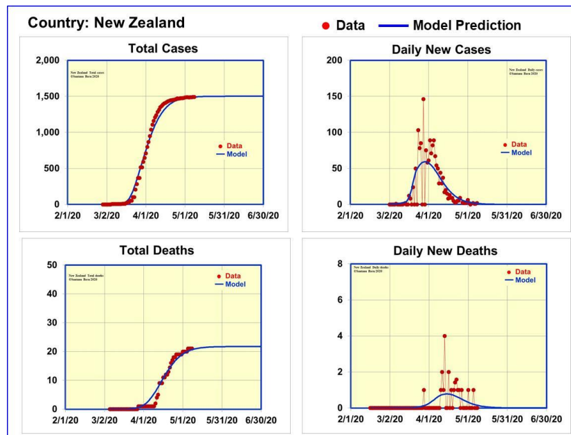
Figure 7. Data and model predictions for Covid-19 cases in New Zealand
