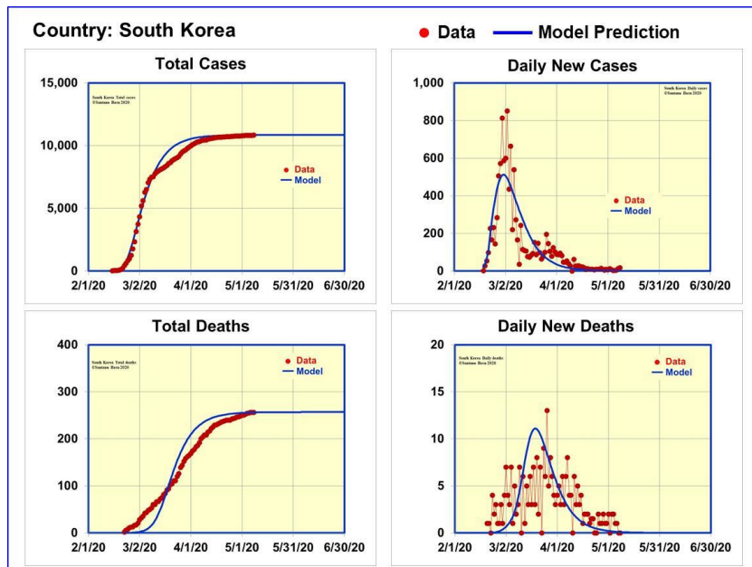
Figure 6. Data and model predictions for Covid-19 cases in South Korea
