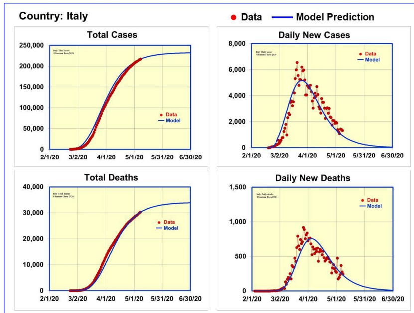
Figure 5. Data and model predictions for Covid-19 cases in Italy
