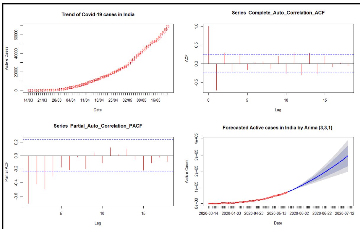
Fig. 1(b) Correlogram and ARIMA Forecast for the Active COVID-19 Cases in India
