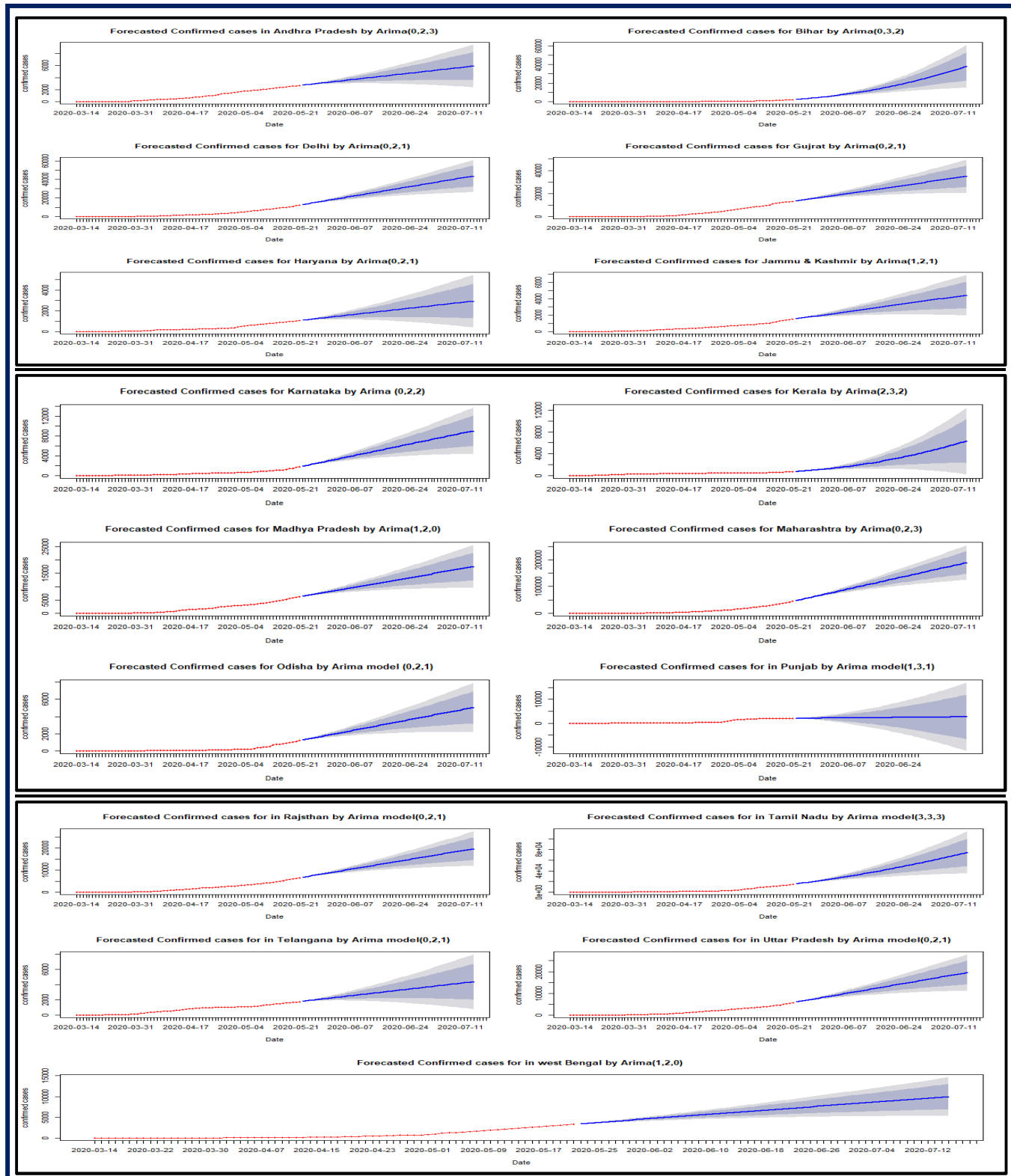
Fig.4 Forecast trend of Confirmed cases of COVID-19 for Indian States
