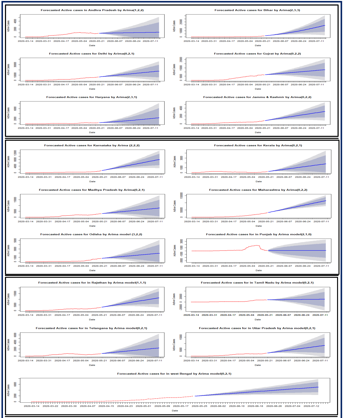
Fig.4 Forecast trend of Active cases of COVID-19 for Indian States
