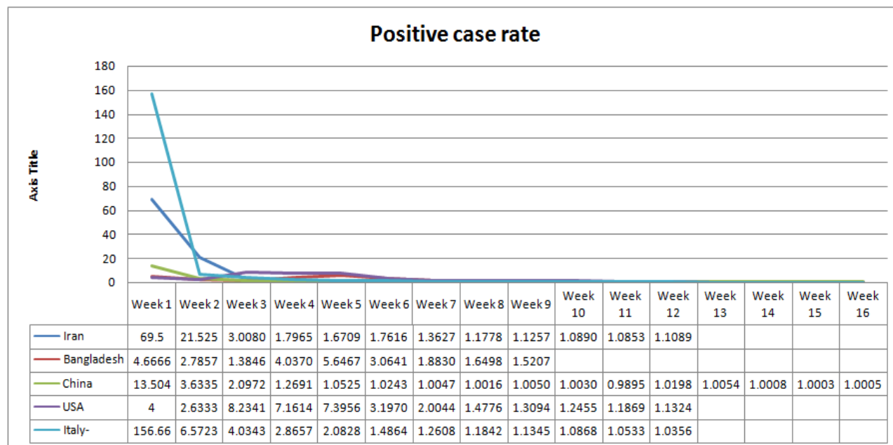
Figure 3: Rate of positive case of Italy, Iran, China, Bangladesh and the USA
