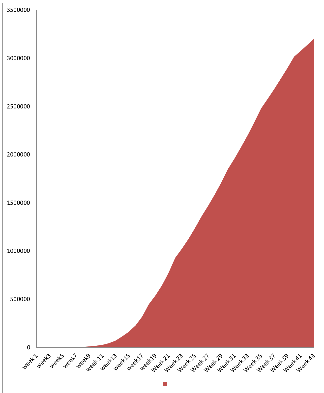
Diagram: Series of COVID 19 positive case
