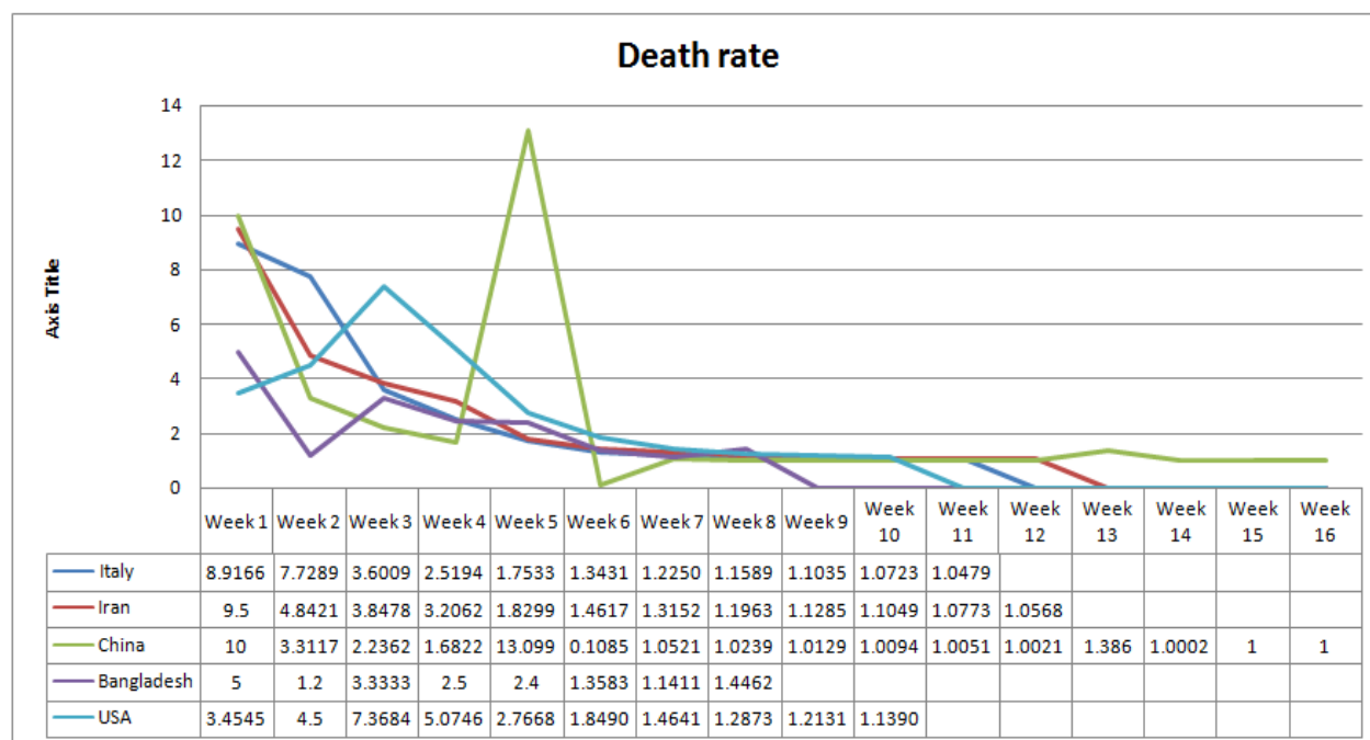
Figure 3: Death rate of Italy, Iran, China, Bangladesh and the USA
