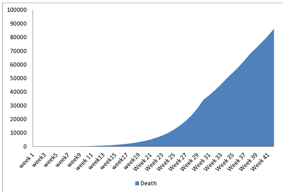
Diagram 2: Series of Death of COVID 19
