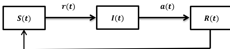
Figure 2: Description of SIR model considering COVID-2019 outbreak virus evolution
