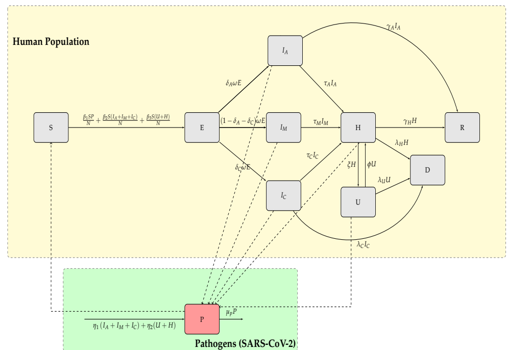
Fig 1. Compartmental model of the SEIR model of transmission of COVID-19
