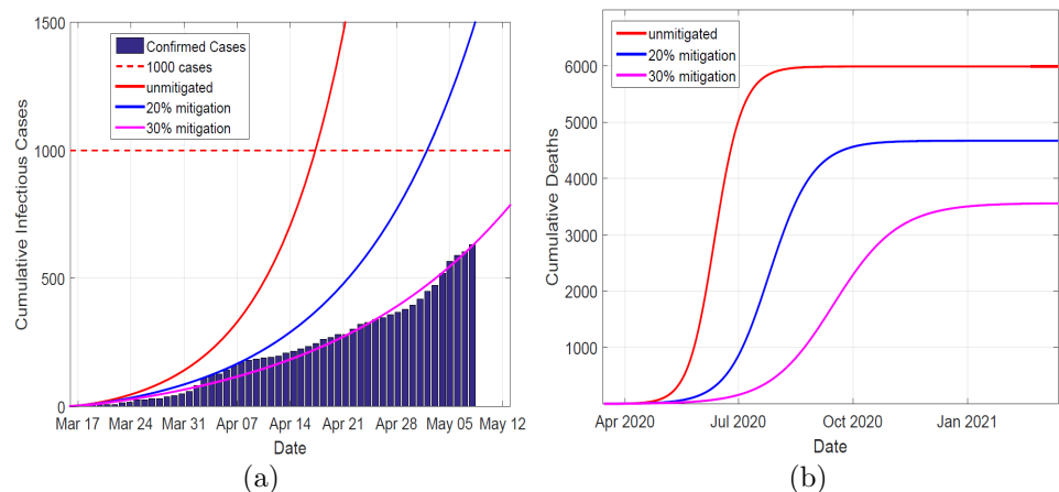
Fig 3. Left panel depicts the data of the confirmed cases in Kenya against the simulated infectious cases for the first 60 days, in unmitigated and mitigated situations. The simulated results of a 30% NPIs effectiveness coincides with the data. Right panel show the cumulative deaths, which decline significantly as the NPIs take effect.
