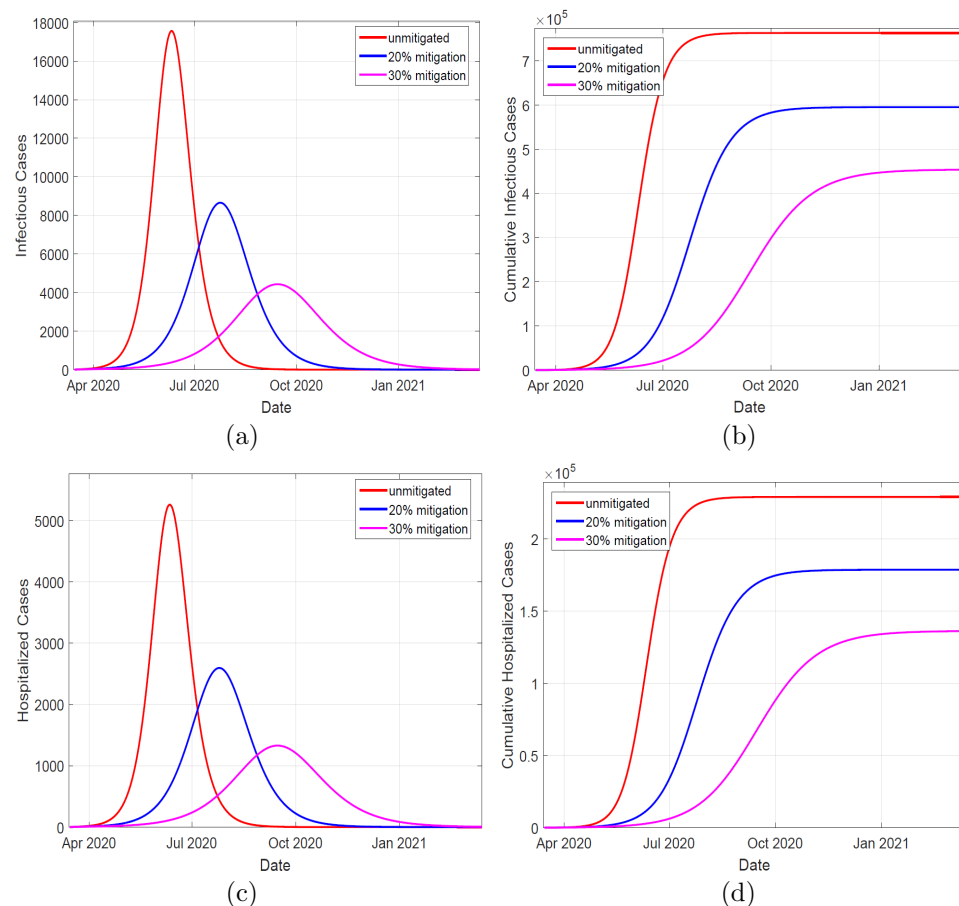
Fig 2. Left panels depicts simulation of infectious and hospitalized cases, in unmitigated and mitigated situations. The implementation of NPIs results to a delay and significant reduction in the cases, as shown by the varying peaks. Right panels show the simulated cumulative cases for both infectious and hospitalized individuals. The infectious cases comprise of individuals in compartments I_A , I_M , and I_C cases. The hospitalized cases comprise of individuals in compartments H and U .
