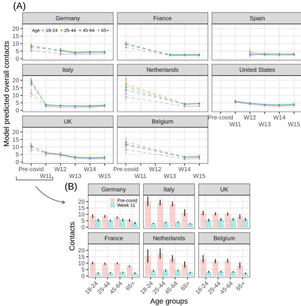
Fig. 3. Weekly overall social contacts by age (90% outlier scenario): trends for the model that predicts overall social contact numbers by age group and by week ( A ), and comparison of the model that predicts overall social contact numbers between the pre-COVID period and the first week of available data for each country ( B ). Pre-COVID model predictions adjusted for age, sex, education, and household size. CHBS model predictions adjusted for age, gender, region of residence, education, day of the week, being foreign-born, and household size. All social contact numbers exclude the top 10% of the distribution.
