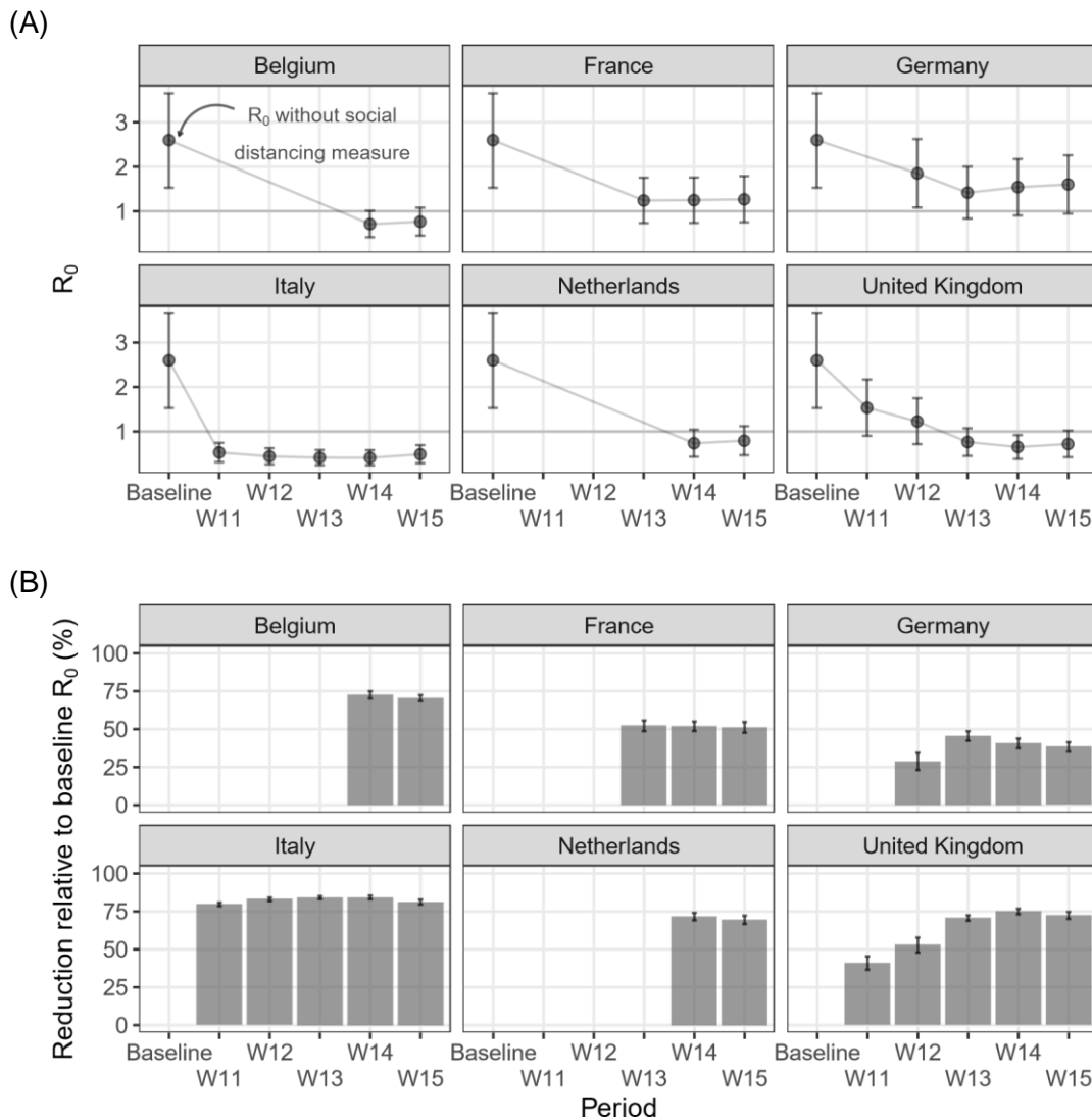
Fig. 4. Weekly changes in the basic reproduction number (90% outlier scenario): Expected change in R_0^b of COVID-19 by calendar week following the reduction in the number of overall social contacts due to the physical distancing measures. Panel (A) shows the reduction in the R_0^b and panel (B) shows the reduction as a percentage. The 95% CIs are based on 10,000 replicates. The CHBS social contacts exclude the top 10% of the distribution.
