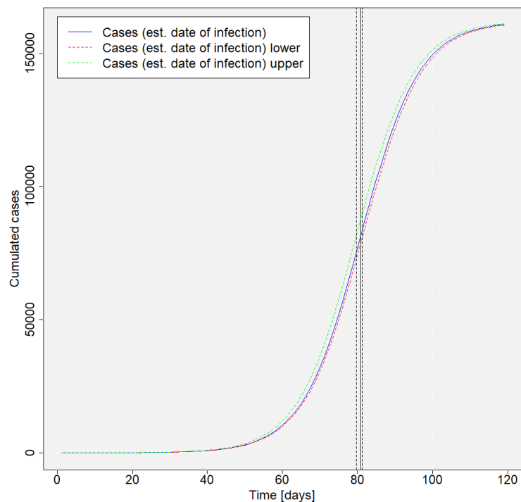
Figure 4: Estimated logistic growth model (including inflection point) for cumulative SARS-CoV-2 infections in Germany (based on estimated dates of infection) incorporating upper and lower bounds (95%-CI)
