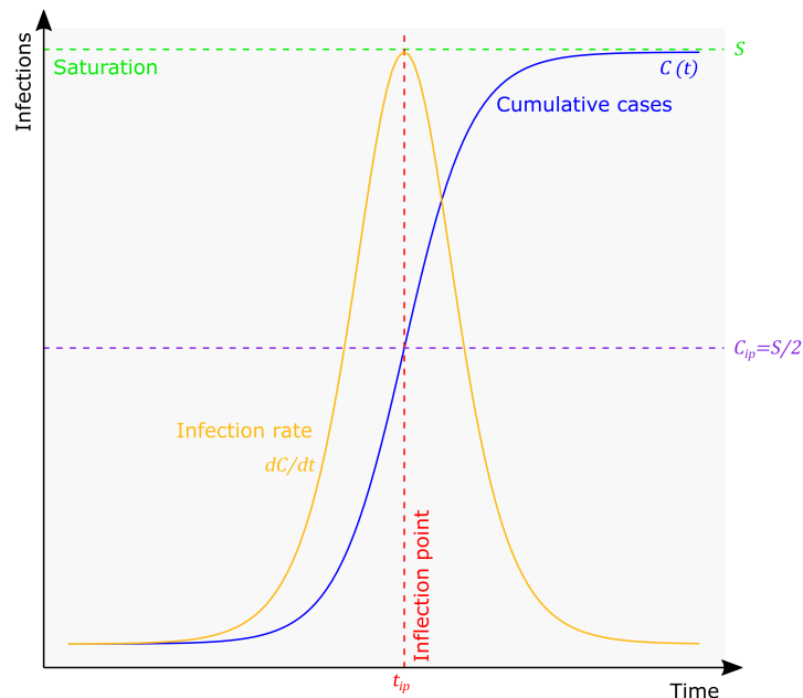
Figure 1: Logistic growth of an epidemic
