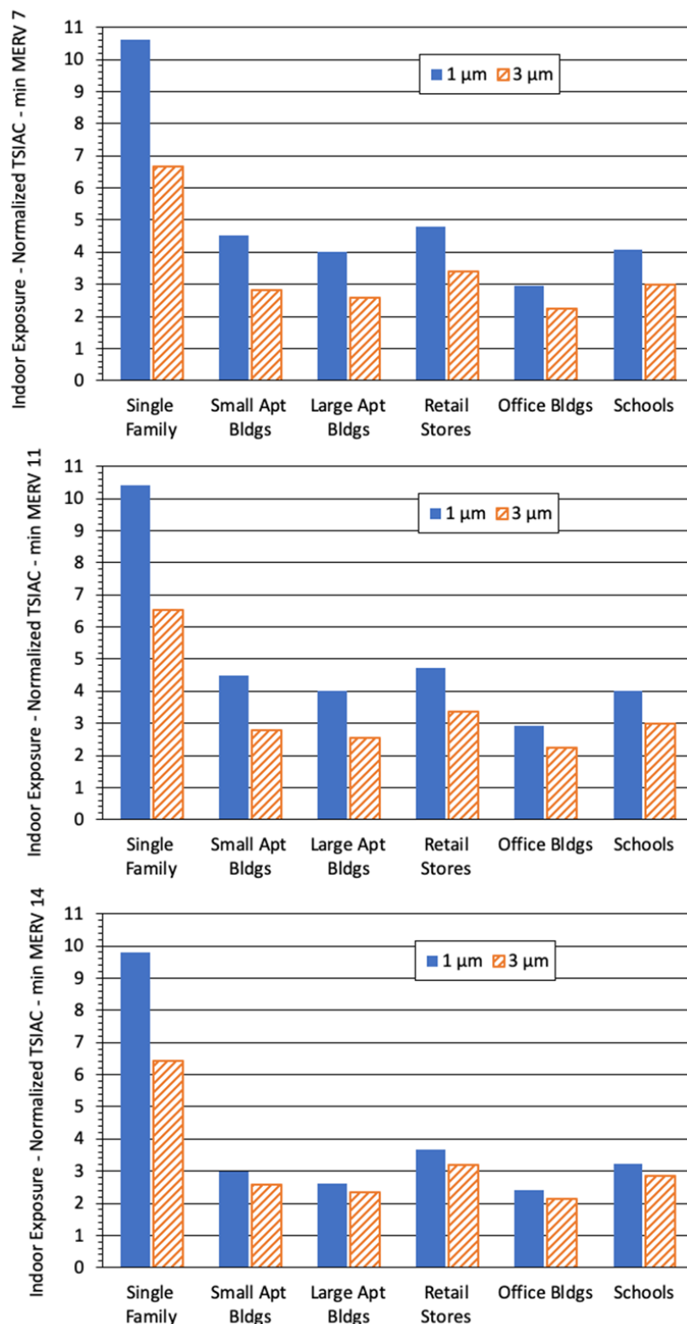
1116 1117 Figure C2. Improved filtration scenario results for the US Indoor Normalized Time and Space 1118 Integrated Air Concentration (Indoor Normalized TSIAC in s\ m^{-1} ) – indoor exposures to indoor- 1119 origin airborne particles – for selected building types; two aerosol sizes: 1 \mu m (solid bar) and 3 1120 \mu m diameter (diagonal striped bar); and a 0\ h^{-1} airborne loss rate. Higher Indoor Normalized 1121 TSIAC values correspond to greater exposures. Note the change in vertical scale from Figure 3 .
