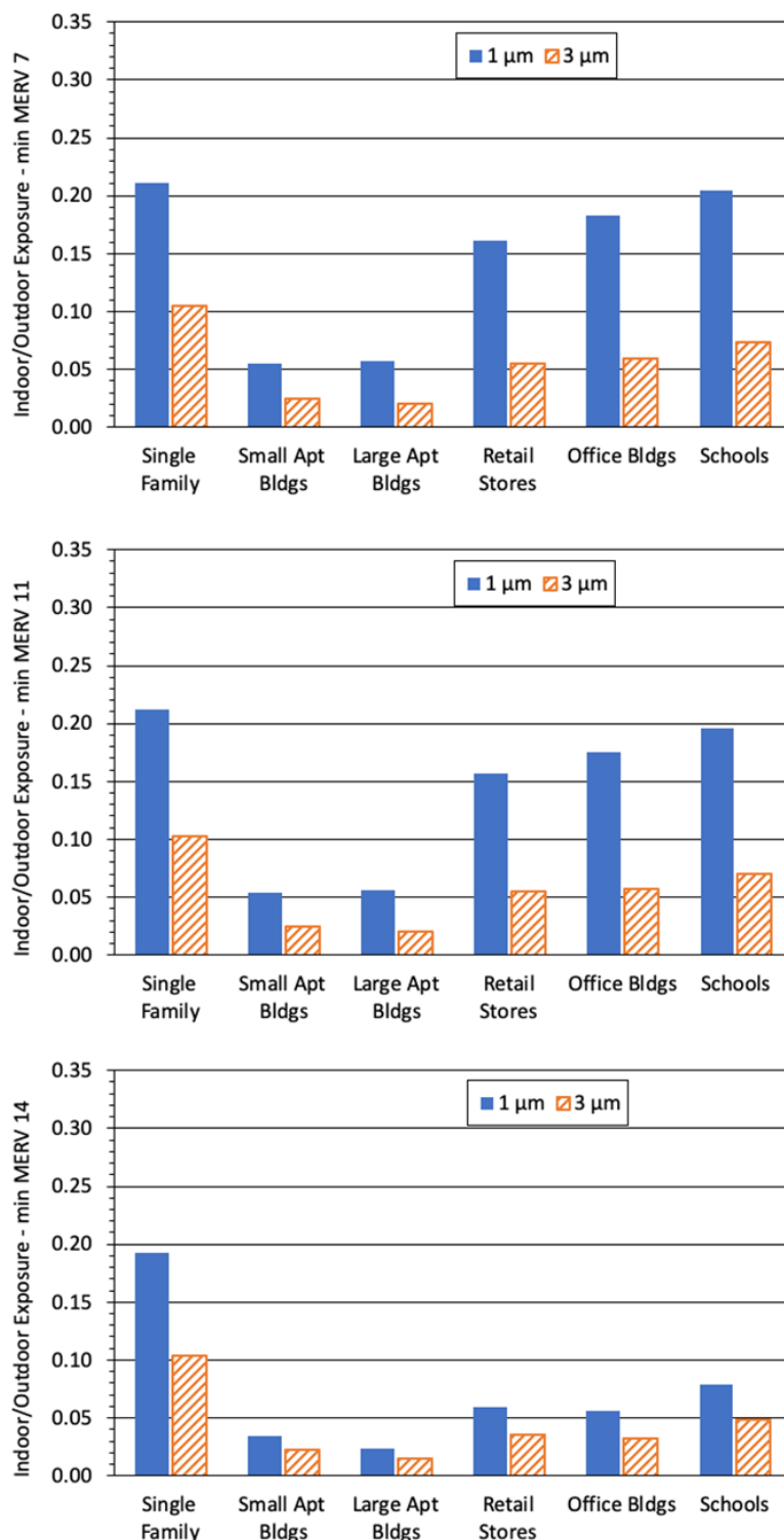
1110 1111 Figure C1. Improved filtration scenario results for the US Building Transmission Factor 1112 (dimensionless) – the ratio of the indoor exposures to the corresponding outdoor exposure – 1113 for selected building types; two aerosol sizes: 1 μm (solid bar) and 3 μm diameter (diagonal 1114 striped bar); and a 0 h -1 airborne loss rate. Higher Building Transmission Factor values 1115 correspond to greater exposures.
