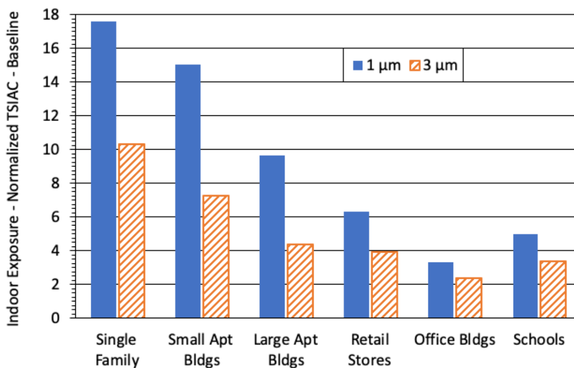
593 Figure 3. Baseline scenario results for the US Indoor Normalized Time and Space Integrated Air 594 Concentration (Indoor Normalized TSIAC in \text{s m}^{-1} ) – indoor exposures to indoor-origin airborne 595 particles – for selected building types; and two aerosol sizes: 1 \mu\text{m} (solid bar) and 3 \mu\text{m} 596 diameter (diagonal striped bar). Higher Indoor Normalized TSIAC values indicate more 597 exposure. 598 599
