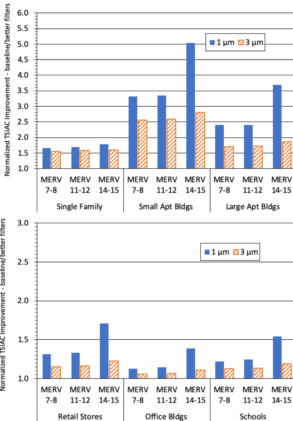
630 Figure 4. Improvement in the US Indoor Normalized TSIAC for selected residential (top panel) 631 and non-residential (bottom panel) building types; two aerosol sizes: 1 \mu\text{m} (solid bar) and 3 \mu\text{m} 632 diameter (diagonal striped bar); and 3 minimum MERV ratings. The vertical axis shows the ratio 633 of the Indoor Normalized TSIAC for the baseline scenario to the specified improved filtration 634 scenario (a value of 1 indicates no improvement, larger numbers indicate greater 635 improvement). Note the factor of 2 difference in vertical scales between the top and bottom 636 panels.
