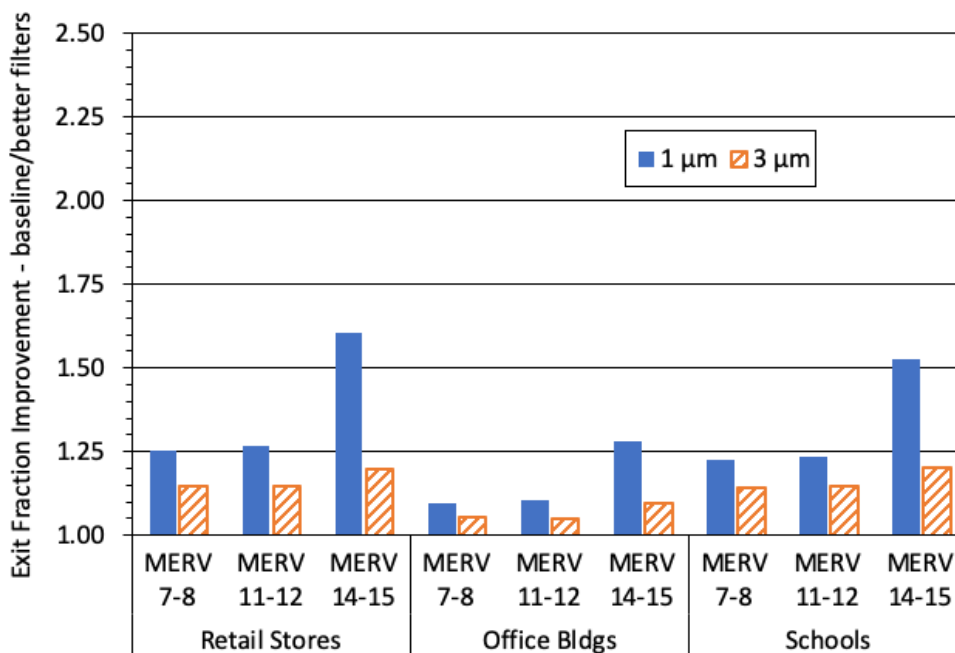
Figure 6. Improvement in the US Building Exit Fraction for selected residential (top panel) and non-residential (bottom panel) building types; two aerosol sizes: 1 μm (solid bar) and 3 μm diameter (diagonal striped bar); and 3 minimum MERV ratings. The vertical axis shows the ratio of Building Exit Fraction for the baseline scenario to the specified improved filtration scenario (a value of 1 indicates no improvement, larger numbers indicate greater improvement). Note the factor of 2 difference in vertical scales between the top and bottom panels.
