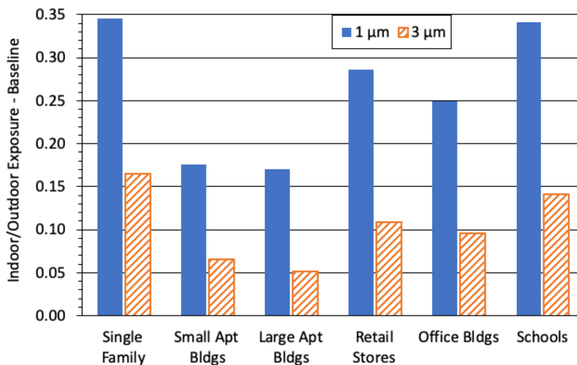
535 Figure 1. Baseline scenario results for the US Building Transmission Factors (dimensionless) – 536 the ratio of the indoor exposures to the corresponding outdoor exposure – for selected building 537 types; and two aerosol sizes: 1 \mu\text{m} (solid bar) and 3 \mu\text{m} diameter (diagonal striped bar). Higher 538 Building Transmission Factor values indicate more exposure. 539
