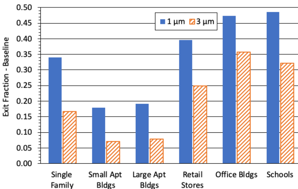
657 658 Figure 5. Baseline scenario results for the US Building Exit Fraction (dimensionless) – the 659 fraction of indoor airborne particles that are released to the outdoor atmosphere – for selected 660 building types; and two aerosol sizes: 1 μm (solid bar) and 3 μm diameter (diagonal striped bar). 661 Higher Exit Fraction values correspond to more particles released to the outdoor atmosphere.
