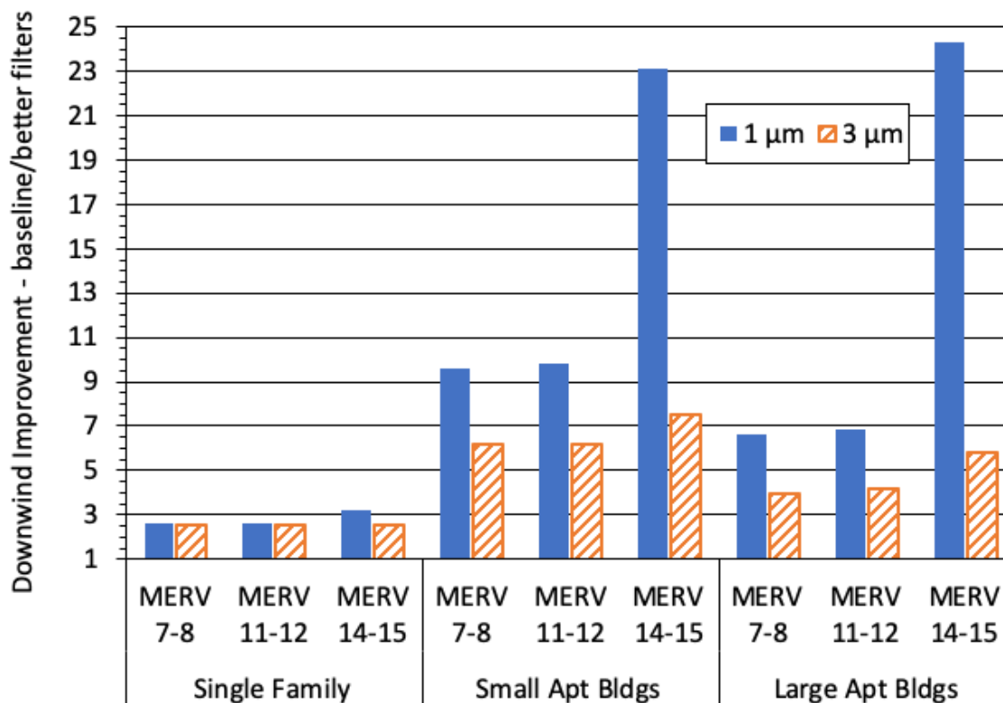
698 699 700 Figure 7. Improvement in the US Downwind Indoor Exposure for homogenous residential 701 neighborhoods comprised of the selected building use types; two aerosol sizes: 1 μm (solid bar) 702 and 3 μm diameter (diagonal striped bar); and 3 minimum MERV ratings. The vertical axis 703 shows the ratio of the Downwind Indoor Exposure for the baseline scenario to the specified 704 improved filtration scenario (a value of 1 indicates no improvement, larger numbers indicate 705 greater improvement). 706
