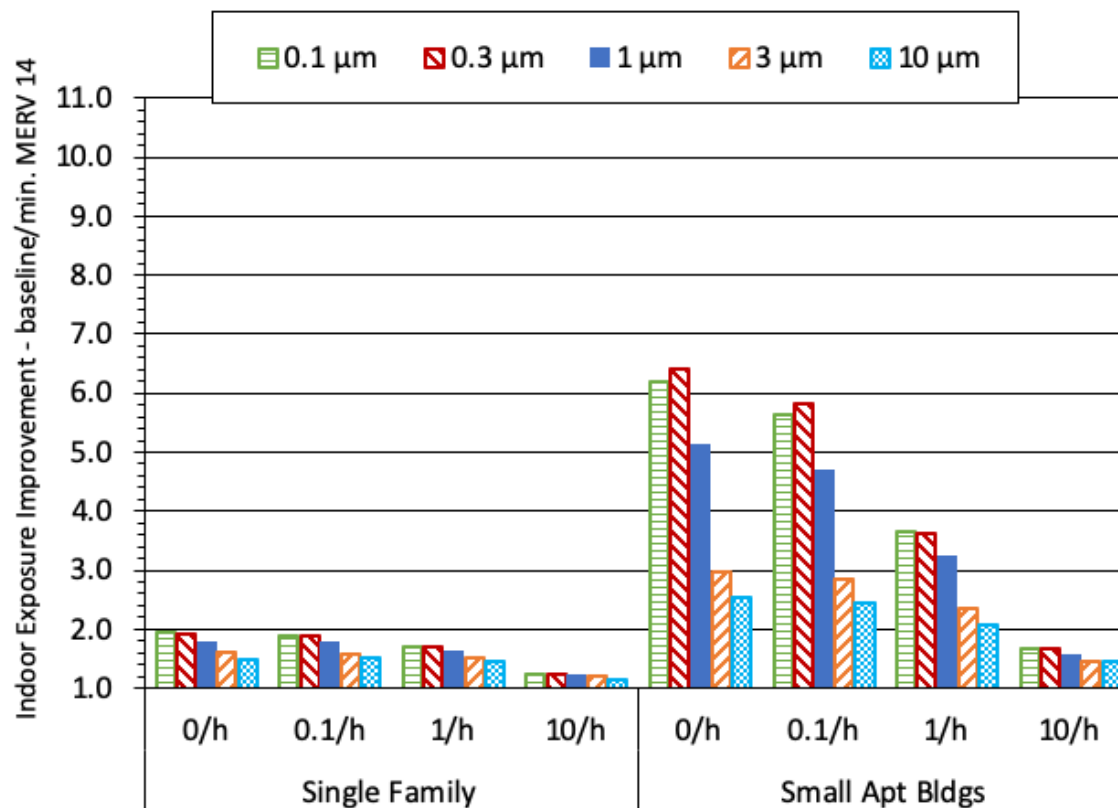
1139 1140 Figure D1. Improvement in the US Building Transmission Factor for two residential building 1141 types; five aerosol sizes: 0.1 μm (horizontal striped bar), 0.3 μm (downward diagonal striped 1142 bar, 1 μm (solid bar), 3 μm diameter (upward diagonal striped bar), and 10 μm diameter 1143 particles (cross-hatched bar); and four airborne loss rates: 0, 0.1, 1, and 10 h -1 . The vertical axis 1144 is the ratio of the Building Transmission Factors for the baseline to the Minimum MERV 14 1145 filtration scenario (a value of 1 indicates no improvement, larger numbers indicate greater 1146 improvement). 1147
