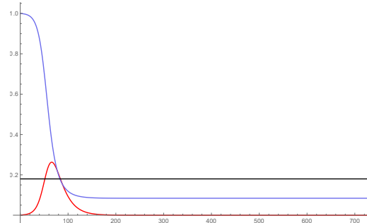
Figure 1: On the left, I(t) (red), S(t) (blue), and b(t) (black) for u(t) = 0 \forall t and T = 1,000 .
