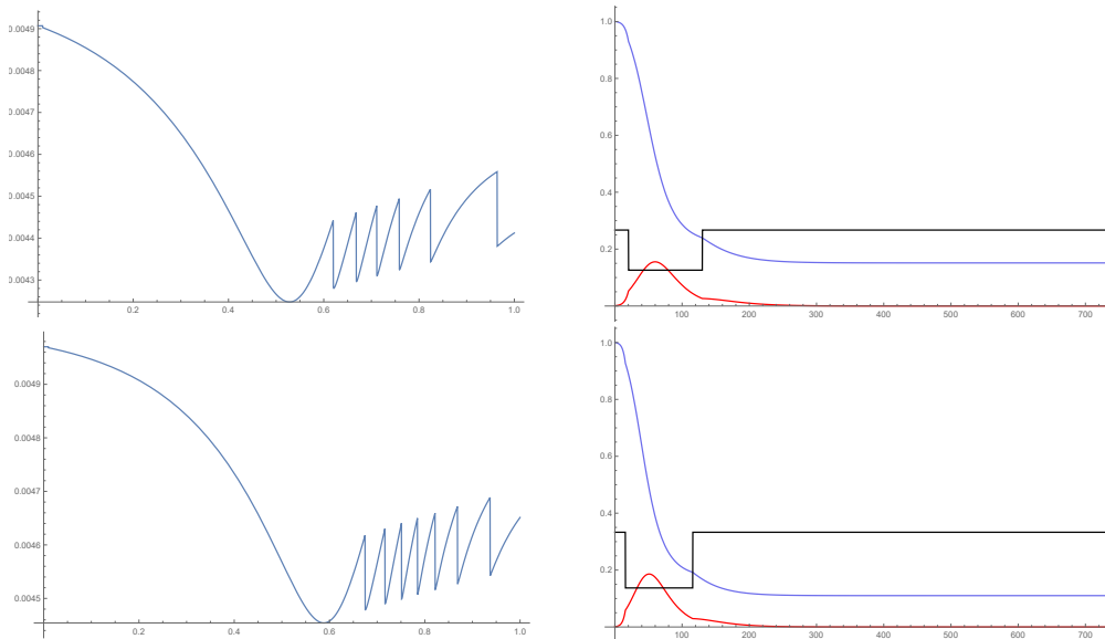
Figure 6: On the left, D(T) as a function of u_1 for u_1 \in [0, 1] and T = 1,000 . On the right, I(t) (red), S(t) (blue), and b(t) (black) for the level u_1^* of u_1 that minimizes the overall fatality rate. On both rows, \alpha_n = 10 and \alpha_c = 20 . On the first row, R_0 = 4 , which gives u_1^* = 52.8\% , and D(T) = 0.425\% . On the second row, R_0 = 5 , which gives u_1^* = 58.8\% , and D(T) = 0.445\% .
