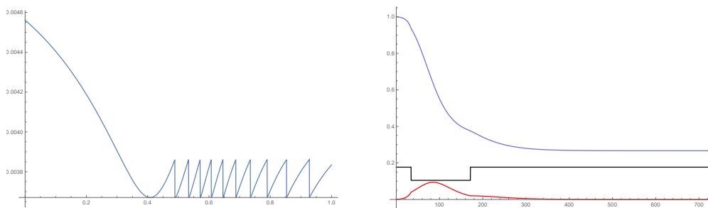
Figure 9: The mitigation threshold is 4% and the opening threshold is 2%. On the left, D(T) as a function of u_1 for u_1 \in [0, 1] and T = 1,000 . On the right, I(t) (red), S(t) (blue), and b(t) (black) for u_1^* = 40.8\% , which gives D(T) = 0.367\% .
