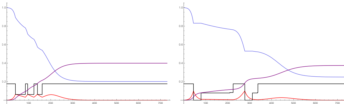
Figure 8: I(t) (red), S(t) (blue), b(t) (black), and 100 \times D(t) (purple), for T = 1,000 . On the left, \alpha_n = 20 and \alpha_c = 40 ; u_1 is set at 65.0%, which gives D(T) = 0.399\% . On the right, \alpha_n = 10 and \alpha_c = 100 ; u_1 = 99.9\% , u_2 = 55.8\% , and u_3 = 53.3\% , which gives D(T) = 0.376\% .
