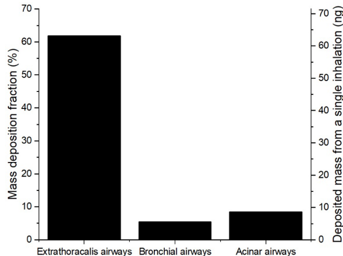
Figure 2. Mass deposition fraction of inhaled particles (left axis) and deposited mass from a single inhalation (right axis) in the extrathoracic, bronchial and acinar regions of the lungs.
