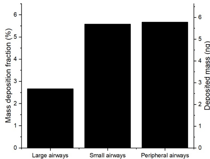
Figure 3. Mass deposition fraction of inhaled particles (left axis) and deposited mass from a single inhalation (right axis) in the large, small, and peripheral airways.
