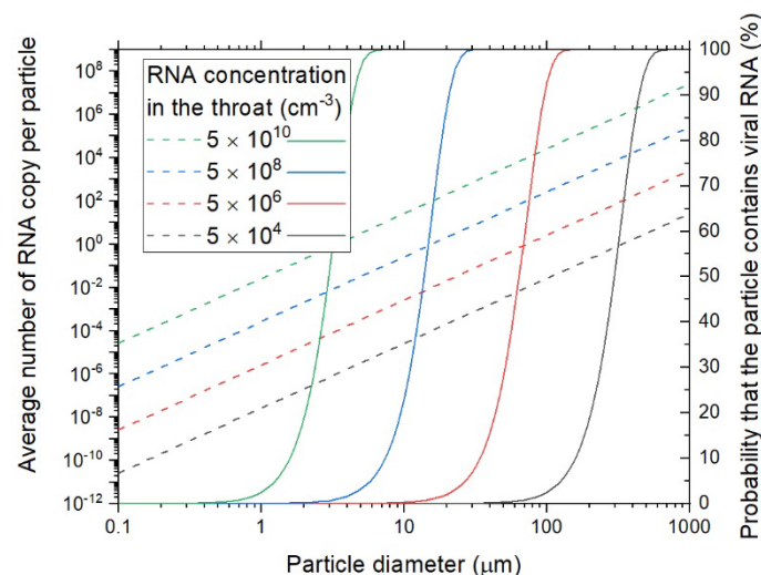
Figure 5. The average number of RNA copies of the virus in one particle (dash lines) and the probability that a particle contains at least one virus copy (solid lines) as the function of particle size in case of different initial virus concentrations in the throat (different colours).
