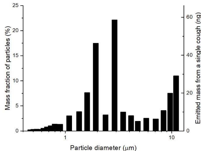
Figure 1. Mass size distribution of particles emitted by coughing of patients with influenza (18). This mass size distribution was used as input in the Monte-Carlo simulations.
