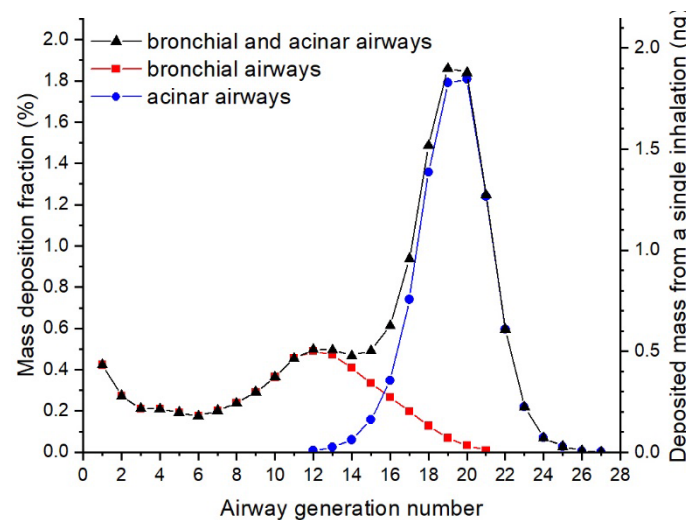
Figure 4. Mass deposition fraction of inhaled particles (left axis) and deposited mass from a single inhalation (right axis) as the function of airway generation number.
