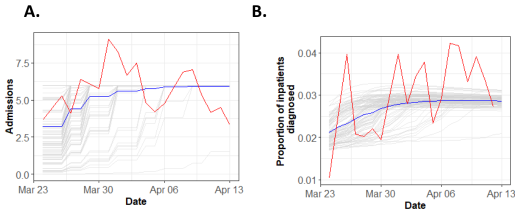
Figure A2: Comparison to NHS Situation Report data: Simulated (blue) and NHS situation report (red) daily admissions data (A) and daily proportion of inpatients developing an infection (B). Grey lines are 100 realisations of simulation.
