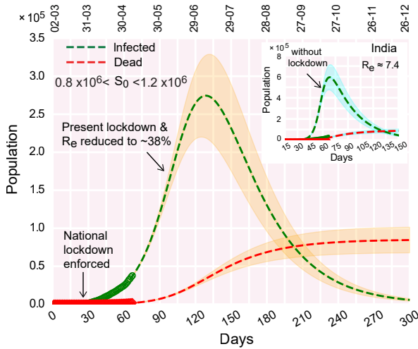
FIG. 4. Best fit of the infection and death curves with the real data freely varying the effective \mathcal{R}_e which appears to be \sim 7.4 in the early stage. The color shades enveloping the curves denote variation in susceptible population within a range of \sim 0.8 - 1.2 \times 10^6 . The real data considered for fitting are from March 2, 2020. Relevant parameters for the analysis are \beta = 0.257 \text{ day}^{-1} , \gamma = 0.0315 \text{ day}^{-1} , \delta = 0.0032 \text{ day}^{-1} , \tau = 29 \text{ days} , T = 7 \text{ days} , \zeta = 0.375 .
