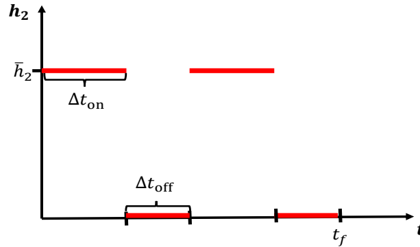
Figure 12: Pulsing of socially distancing protocol. Social distancing is enacted for a time length of \Delta t_{\text{on}} days, followed by a full relaxation for \Delta t_{\text{off}} days. This schedule is then repeated until a time window t_f has been reached.
