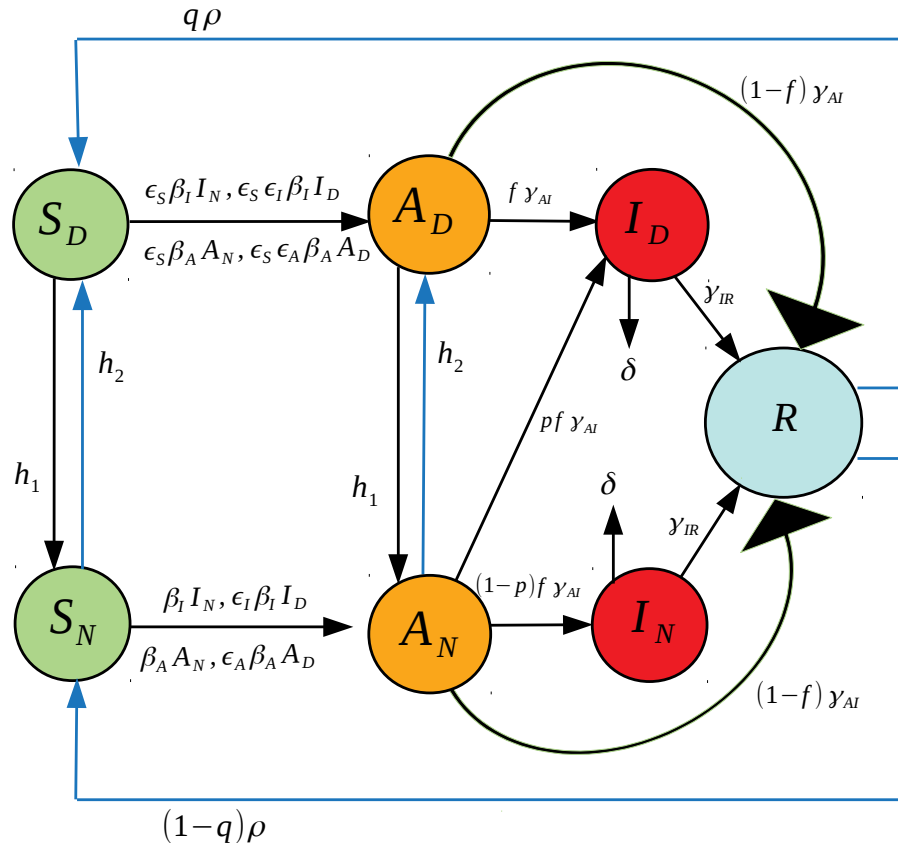
Figure 1: Illustration of the seven compartment SIR model in equations (1)-(7).
