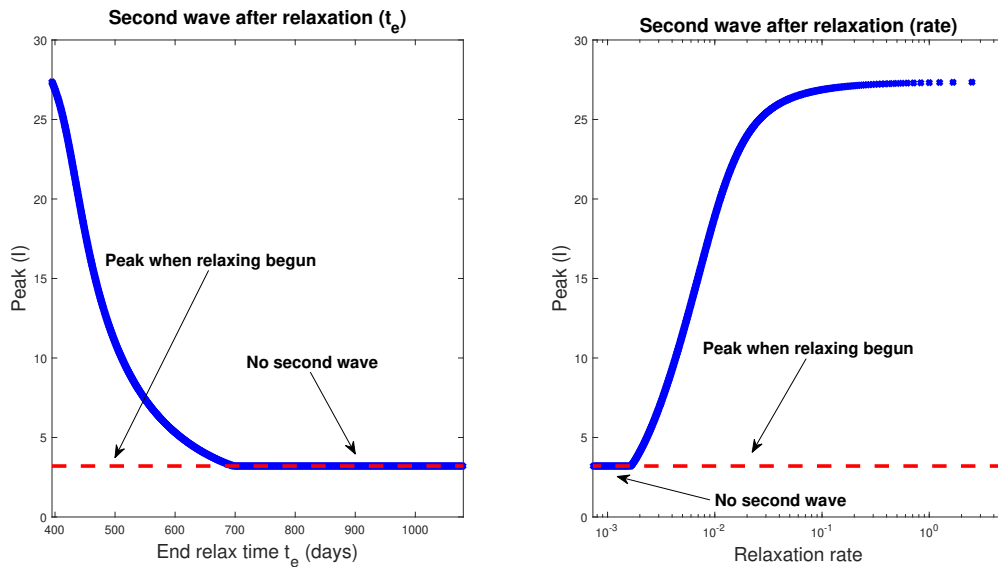
Figure 21: Magnitudes of peak of symptomatic individuals (percentage of total population) as a function of end time t_e (left) and rate (right). Note that t_e and relaxation rate are inversely proportional; see equation (64). Relaxation is begun when the symptomatic population first “flattens,” which is indicated by the dashed red line in the figure, and occurs for all schedules at day t_d = 395 . A peak equal to the dashed red line thus indicates that no second wave of infections occurs, i.e. there was never a day when the number of infected individuals was greater than the peak when relaxation was commenced. All simulations are taken over 1080 days.
