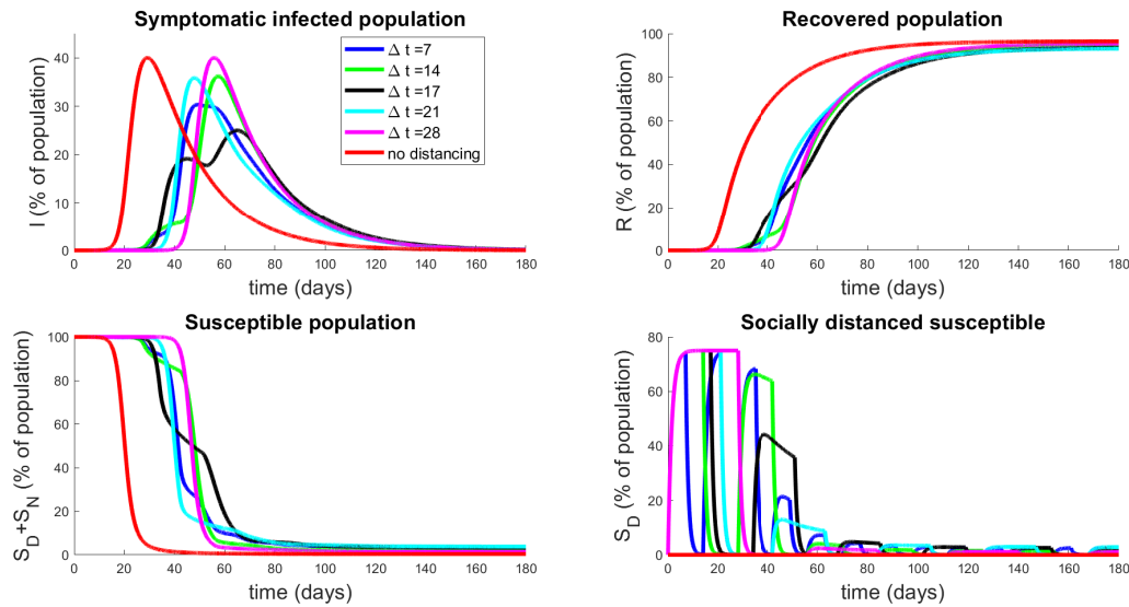
Figure 13: Population response to strategies based on periodic relaxation of social distancing; see Fig. 12. Top left panel denotes temporal dynamics of symptomatic population ( I ) for pulsing strategies with \Delta t_{\text{on}} = \Delta t_{\text{off}} = \Delta t . Non-socially distanced dynamics (red curves) are provided for comparison. Top right panel is recovered population in time, and bottom panels are total susceptible individuals (left) and socially-distanced susceptible individuals (right). Initial conditions are described in Section 3.2.1.
