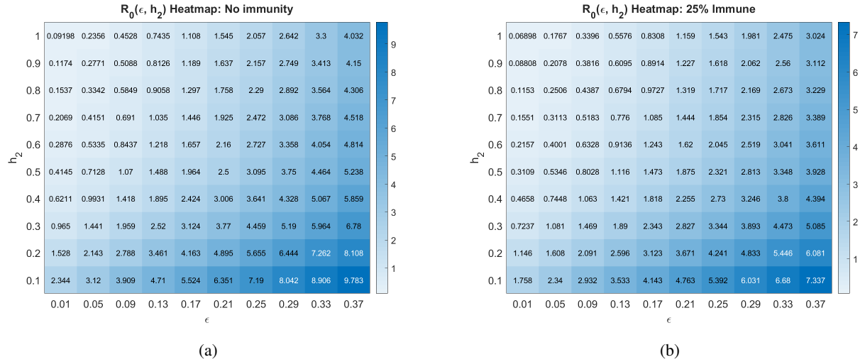
Figure 24: Basic reproduction number as a function of the social distancing rate parameter h_2 and the contact rescaling factor (CoRF) \epsilon at different pandemic stages. CoRF measures the impact of social distancing on infectivity rate. All other parameters as in Table 2.
