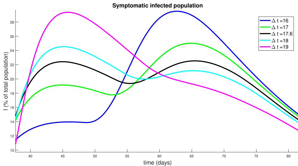
Figure 14: Symptomatic population response to strategies based on periodic relaxation of social distancing (similar to Fig. 13), but for policies with \Delta t near 17 days.
