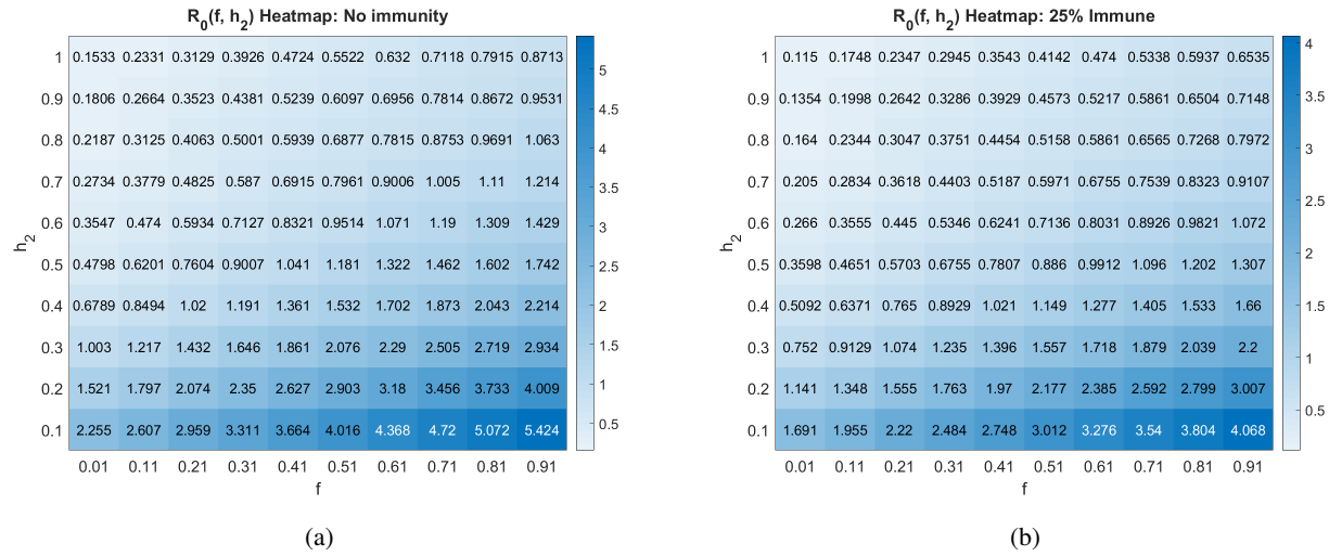
Figure 22: Basic reproduction number as a function of the social distancing rate parameter h_2 and fraction of individuals who become symptomatic ( f ) at different pandemic stages. All other parameters as in Table 2.
