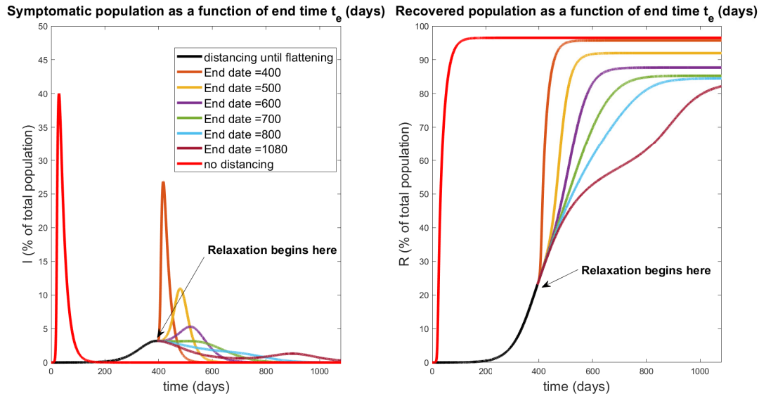
Figure 20: Relaxation that was started during flattening. Symptomatic (left) and recovered (right) populations for policies which relax social distancing at a rate determined (inversely) by t_e , the day at which distancing policies are completely removed. The response for no social distancing implemented is included for reference (red curves). All curves besides the red curve are identical for the first t_d = 395 days of treatment, when social distancing is implemented with h_2(t) \equiv \bar{h}_2 = 0.5 per day for t \in [0, t_d] . Note that a second wave occurs for relaxation protocols that end too quickly ( t_e = 400, 500, 600 days). However, if relaxation is slow enough (larger t_e ), a second wave of infection is completely mitigated. All simulations are taken over 1080 days.
