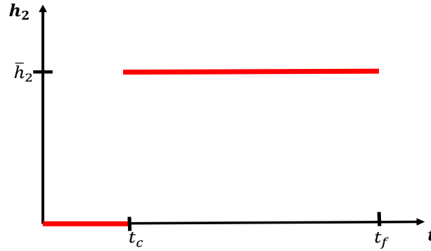
Figure 9: Social distancing control as a function of the delay t_c . Functional form for h_2 used in Figs. 10, 11. See also equation (55).
