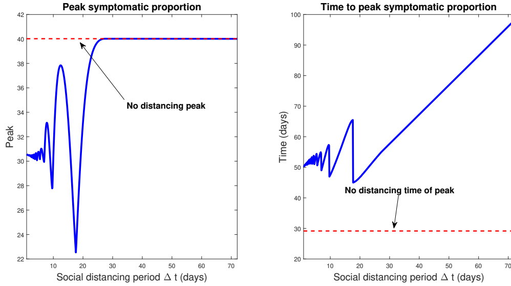
Figure 15: Response of infection dynamics to periodic relaxation for a range of frequencies. Policy period is assumed for 360 days. Left panel denotes peak symptomatic population (percentage) at any one time. Right panel is the corresponding time (in days) when this peak occurs. Initial conditions are described in Section 3.2.1.
