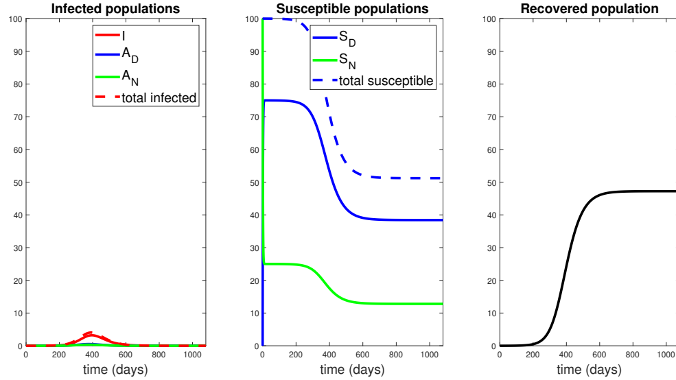
Figure 19: Response to 1080 days of social distancing, with h_2 as in equation (60) for t \in [0, 1080] days. Note the peak of the symptomatic population is approximately 3.2% of the population, occurring at around day 395. As suggested by the right panel, the population is still largely susceptible, and one may suspect that a second epidemic will occur if social distancing protocols are immediately abandoned.
