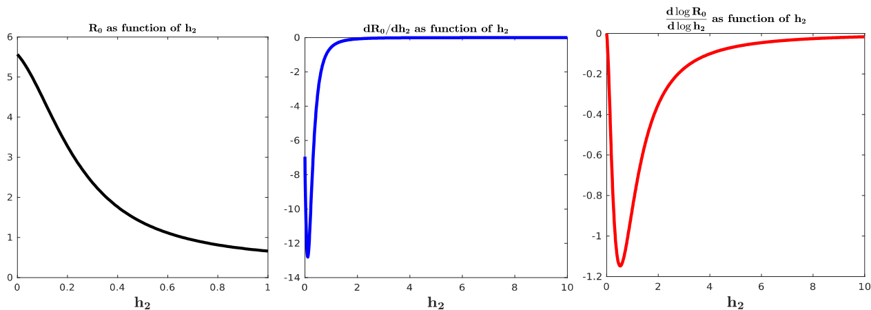
Figure 4: Plots of R_0 , derivative dR_0/dh_2 , and differential sensitivity \frac{d \log R_0}{d \log h_2} = \frac{dR_0}{dh_2} \cdot \frac{h_2}{R_0} , all as functions of h_2 at R^* = 0 . Different ranges picked for clarity. dR_0/dh_2 and differential sensitivity converge to zero.
