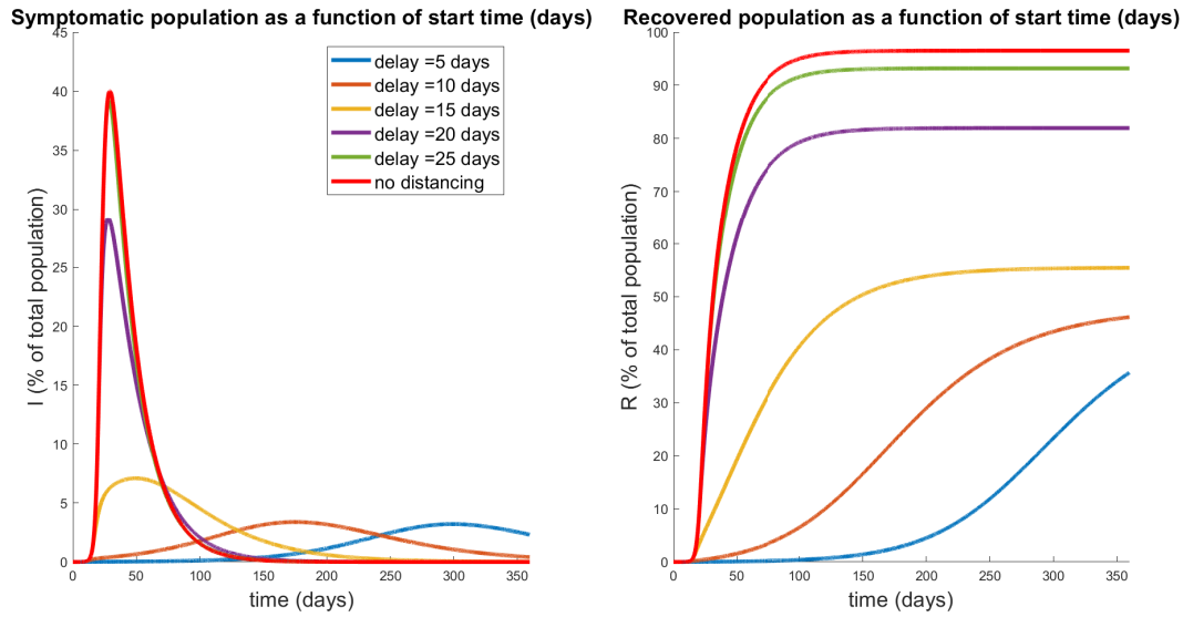
Figure 10: Population response for a treatment window of 360 days with varying start time t_c of social-distancing protocol (see Fig. 9). Left panel denotes the symptomatic ( I ) temporal response; right indicates the recovered percentages for each policy. Red curves correspond to no social distancing (see Fig. 8). Note that a delay of 25 days is hardly discernible from no social distancing, while a significant response transition occurs for delays shorter than 15 days.
