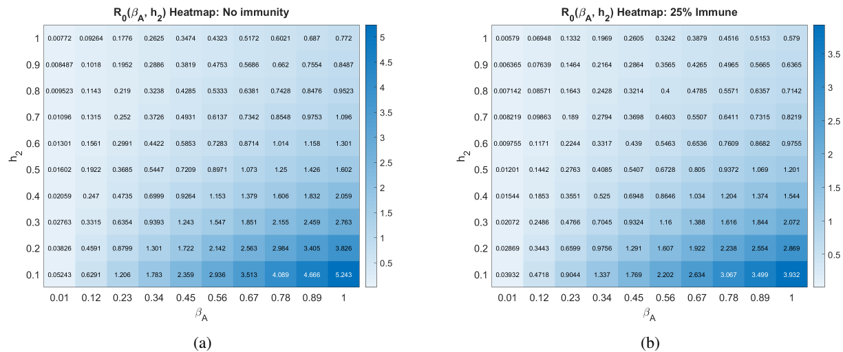
Figure 23: Basic reproduction number as a function of the social distancing rate parameter h_2 and infectivity rate of asymptomatics \beta_A at different pandemic stages. All other parameters as in Table 2.
