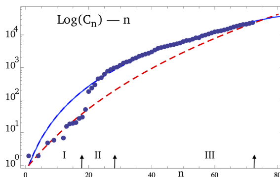
Figure 2: In the log-plot number of confirmed COVID-19 cases in Pakistan, \log(C_n) are plotted versus the number of days n , from February 26, 2020. The real time data is presented by blue dots. The number of confirmed cases in the first twenty days follows DG 2 M curve for r = 0.3 and p = 0.875 (red dashed line). The real time data follows DG 2 M curve for r = 0.74 and p = 0.74 (blue line).
