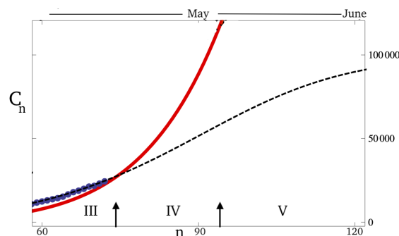
Figure 3: Evolution of confirmed COVID-19 patients ( C_n ) in Pakistan plotted versus number of days, n . The real time data is presented by blue dots, the DG^2M result is plotted (by red line) for r = 0.3 and p = 0.875 . DGRM results is plotted (in black dashed line) for r = 0.74 and p = 0.74 , \alpha = 2 and K = 100000 .
