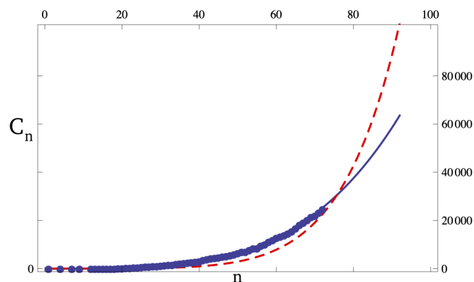
Figure 1: Evolution of confirmed COVID-19 patients ( C_n ) in Pakistan plotted versus number of days, n . The real time data is presented by blue dots. The number of confirmed cases in the first twenty days follows DG 2 M curve for r = 0.3 and p = 0.875 (red dashed line). The real time data in stage III follows DG 2 M curve for r = 0.74 and p = 0.74 (blue line).
