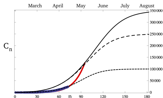
Figure 4: Evolution of Confirmed COVID-19 patients ( C_n ) plotted versus number of days, n . The real time data is presented by blue dots, the DG^2M result is plotted (by red line) for r = 0.3 and p = 0.875 . DGRM results is plotted (in black dashed line) for r = 0.74 and p = 0.74 , \alpha = 2 and K = 100000 . DGRM results plotted in black big-dashed line and black line for K = 250000 and K = 350000 .
