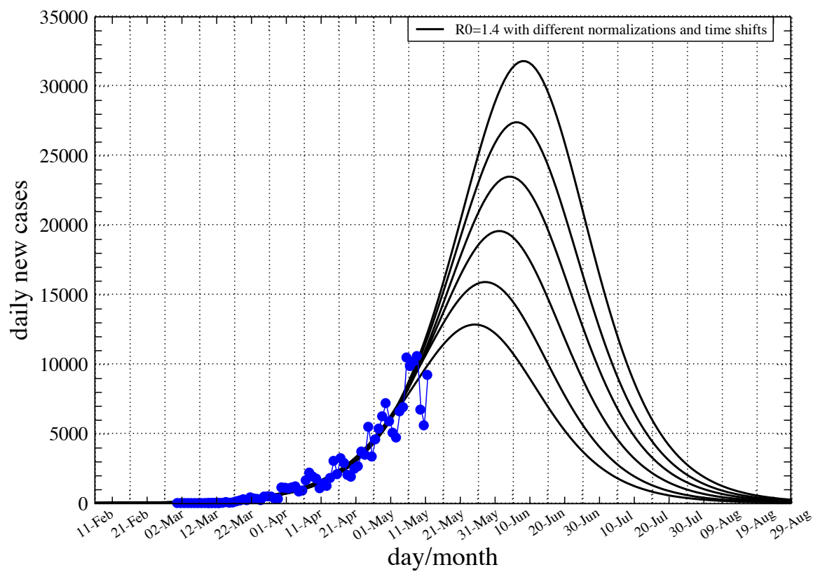
Figure 2: Reported daily number of new cases in Brazil (blue dots), solid line is the result of the simulation with the same parameters as in Figure 1 (blue curve) with different normalizations and time shift factors.
