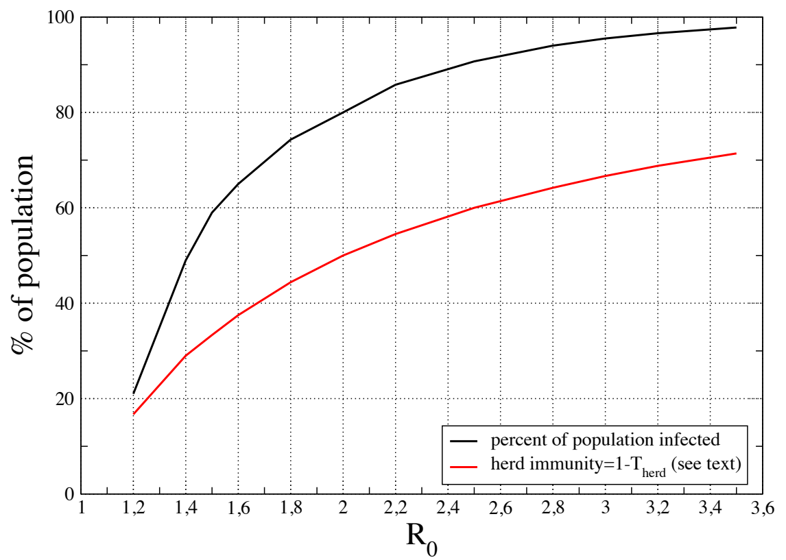
Percent of population contaminated and herd immunity as a function of R_0 .
