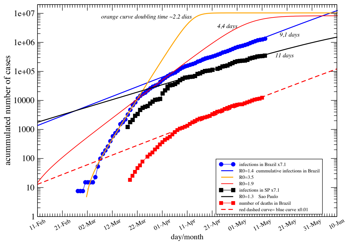
Figure 1: Contamination curves (solid lines). Number of cases in Brazil (blue circles). Number of cases in São Paulo (black squares), number of deaths in Brazil (red squares).
