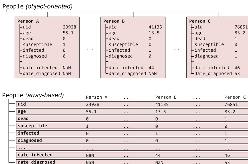
Fig. 5: Illustration of the standard object-oriented approach for implementing agent-based models (top), where each agent is a separate object, compared with the approach used in Covasim (bottom), where agents are represented as slices through a set of state arrays. Dots (...) represent omitted entries. In practice, each agent has 40 states, and there are typically hundreds of thousands of agents.
