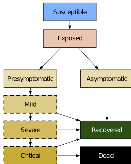
Fig. 1: Covasim model structure, including infection (exposure), disease progression, and final outcomes. Yellow shading indicates that an individual is infectious and can transmit the disease to other susceptible agents. States with a dashed border are considered symptomatic with respect to symptomatic versus asymptomatic testing.
