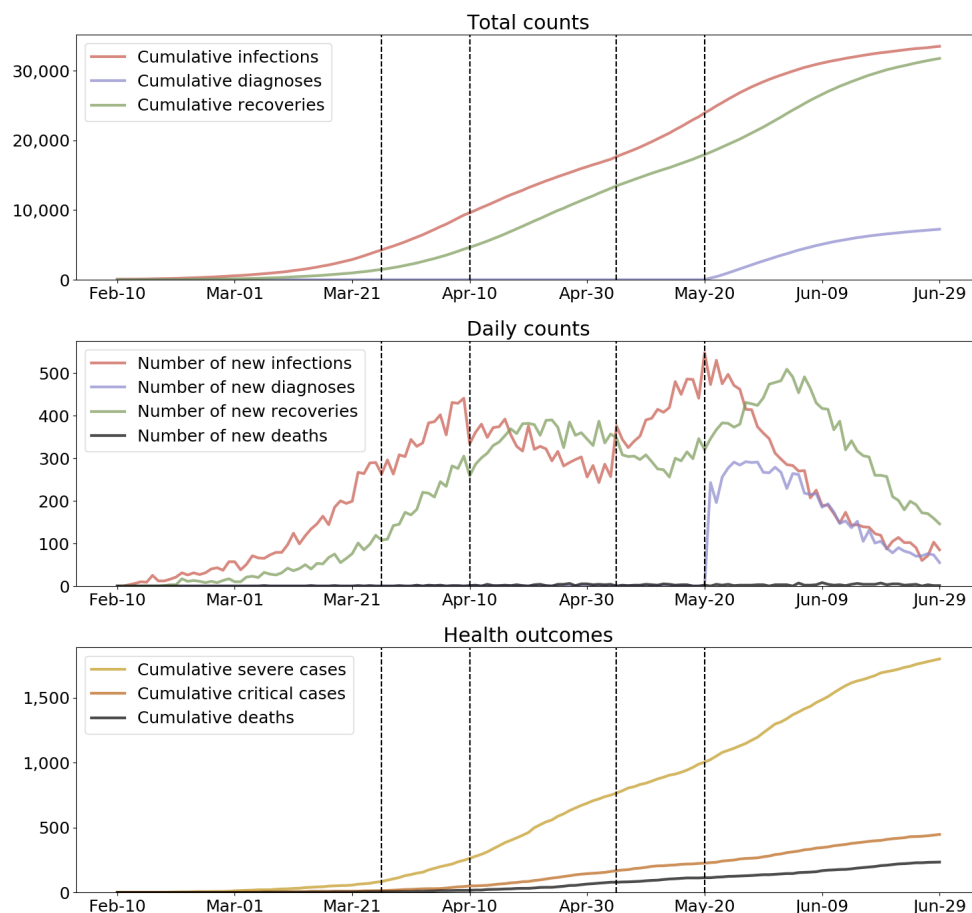
Fig. 8: Illustrative example of a single run of a Covasim simulation. Interventions (described in the text) are shown as dashed vertical lines.
