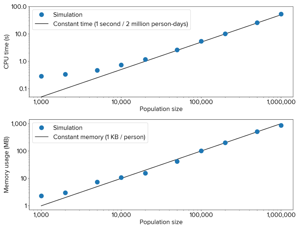
Fig. 6: Covasim performance in terms of processor usage (top) and memory usage (bottom), showing nearly linear scaling over three orders of magnitude of population size.
