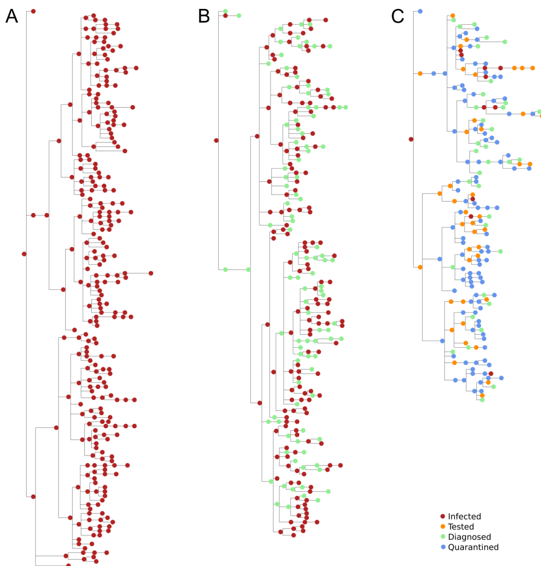
Fig. 10: Example transmission trees for a hypothetical population of 300 individuals with a single seed infection on day 1, with (A) no interventions, (B) testing only, and (C) testing plus contact tracing. Time is shown on the horizontal axis, with each tree representing approximately 90 days. The vertical size of each tree is proportional to the total number of infections.
