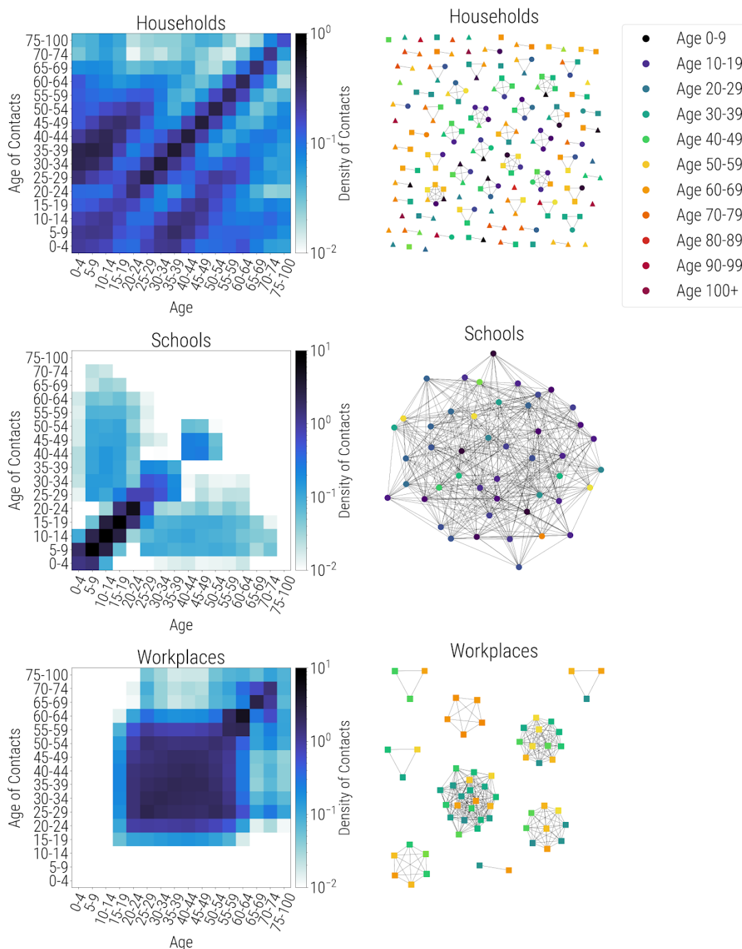
Fig. 4: Synthetic population networks for households (top), schools (middle), and workplaces (bottom). Age-specific contact matrices are shown on the left, while actual connectivity patterns for a 127-person subsample of a population of 10,000 individuals are shown on the right. All individuals are present in the household network, including some with no household connections. A subset of these individuals, including teachers, are present in the school network (circles); another subset is present in workplace networks (squares); some individuals are in neither school nor work networks (triangles).
