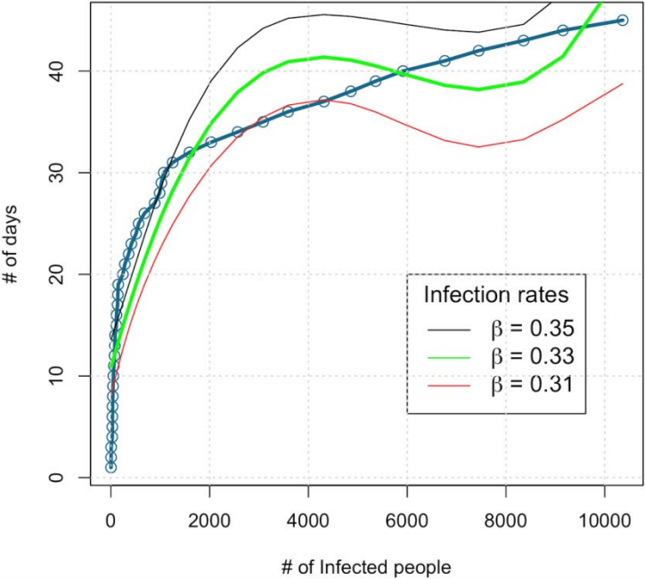
170 171 Fig 2: The comparison of Y(t_s) with the estimated infection rate \beta and the number of daily reported 172 cases of COVID-19 in India from 1st March ( t_s = 0 ) to 14th April ( t_s = 45 )
