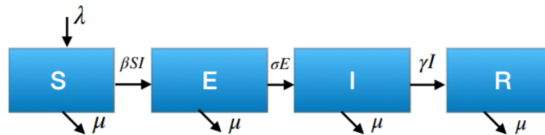
Fig 1: State Diagram for the SEIR epidemic model
