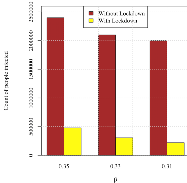
Fig 5: Comparison of the number of predicted infected cases without and with lockdown
