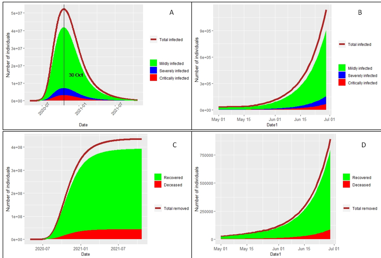
Graph 2: Predictions from Case 3 of step-function modifier- (at \hat{\gamma} = 0.042 )
