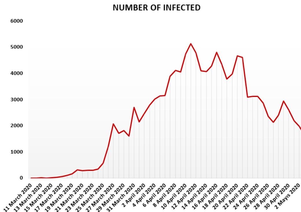
Figure 1. Number of infected people in Turkey from 11 March 2020 to 3 May 2020.
