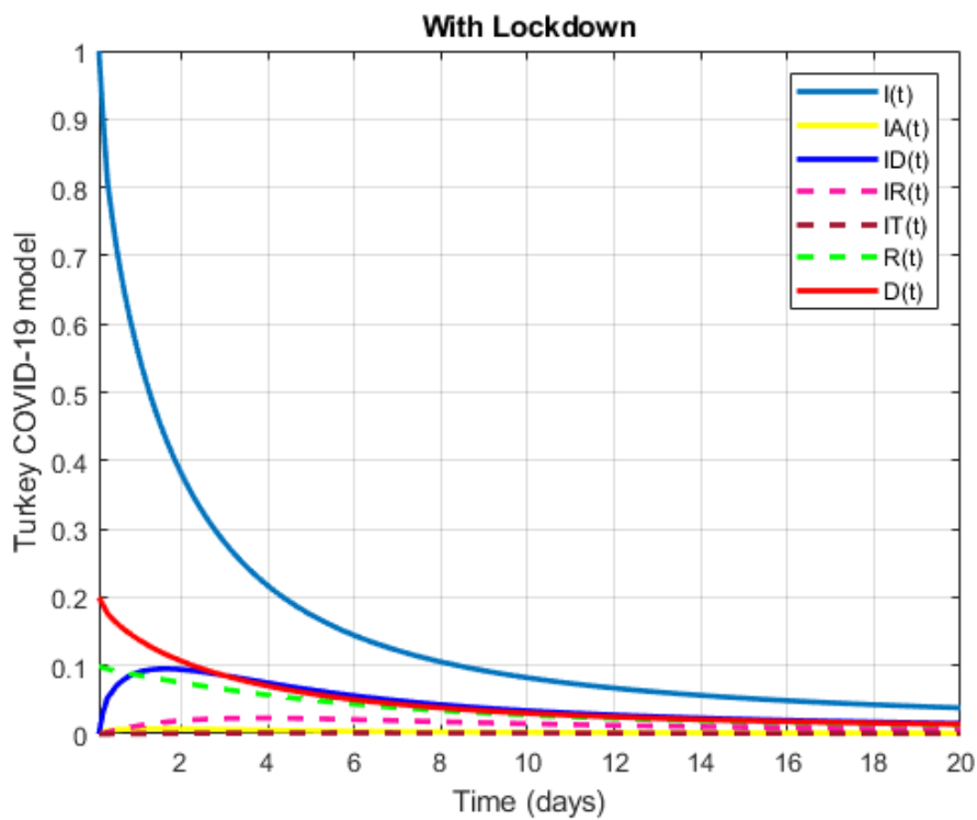
Figure 44. Numerical visualization for COVID-19 model in Turkey for \alpha = 0.7, \beta = 0.75 .
