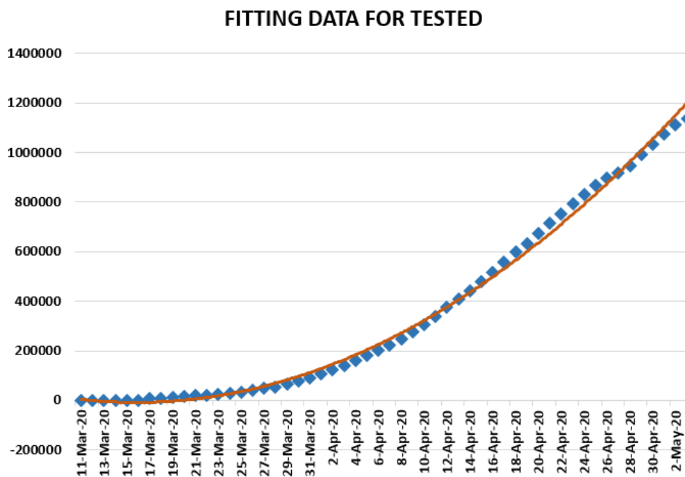
Figure 16. Polynomial fitting data for tested people in Turkey from 11 March 2020 to 3 May 2020.
