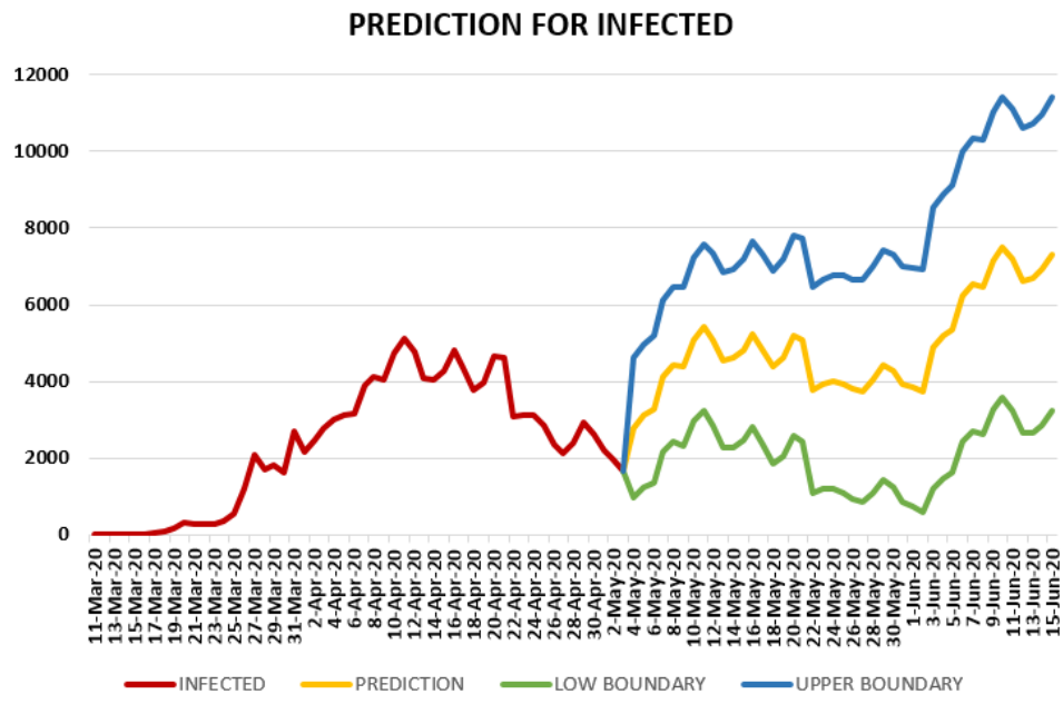
Figure 18. Prediction of daily number of infected in Turkey using Forecast Sheet.
