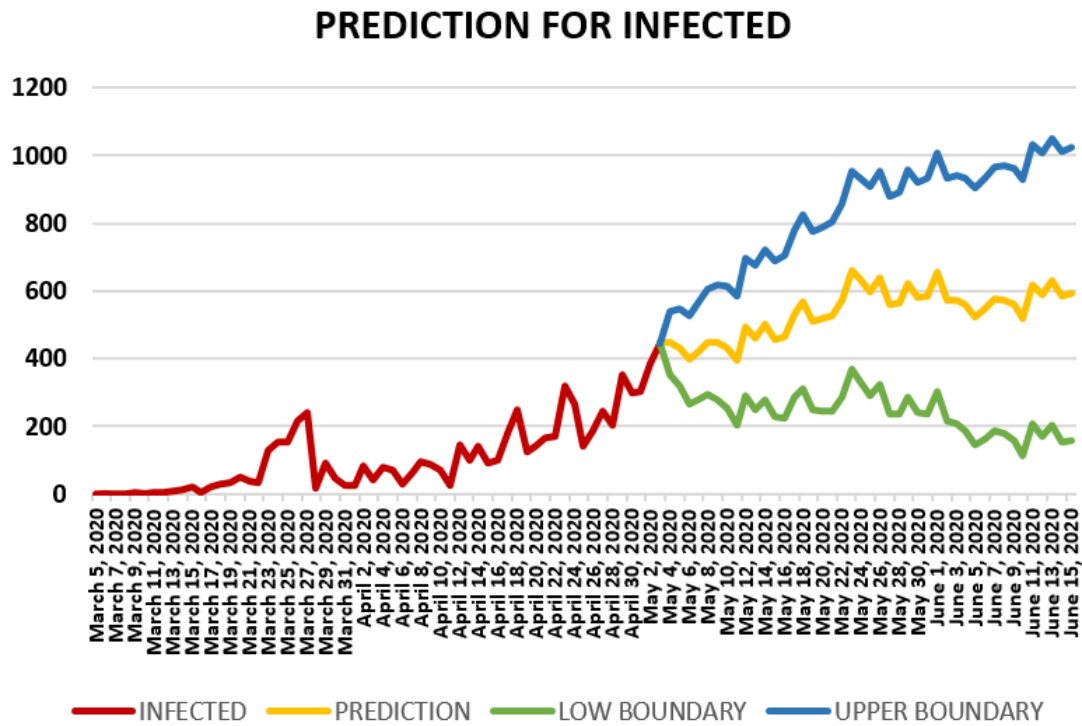
Figure 29. Prediction of daily number of infected in South Africa using Forecast Sheet.
