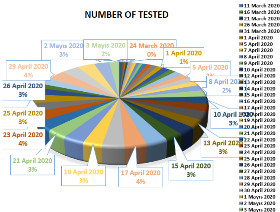
Figure 12. Number of tested people in Turkey from 11 March 2020 to 3 May 2020.
