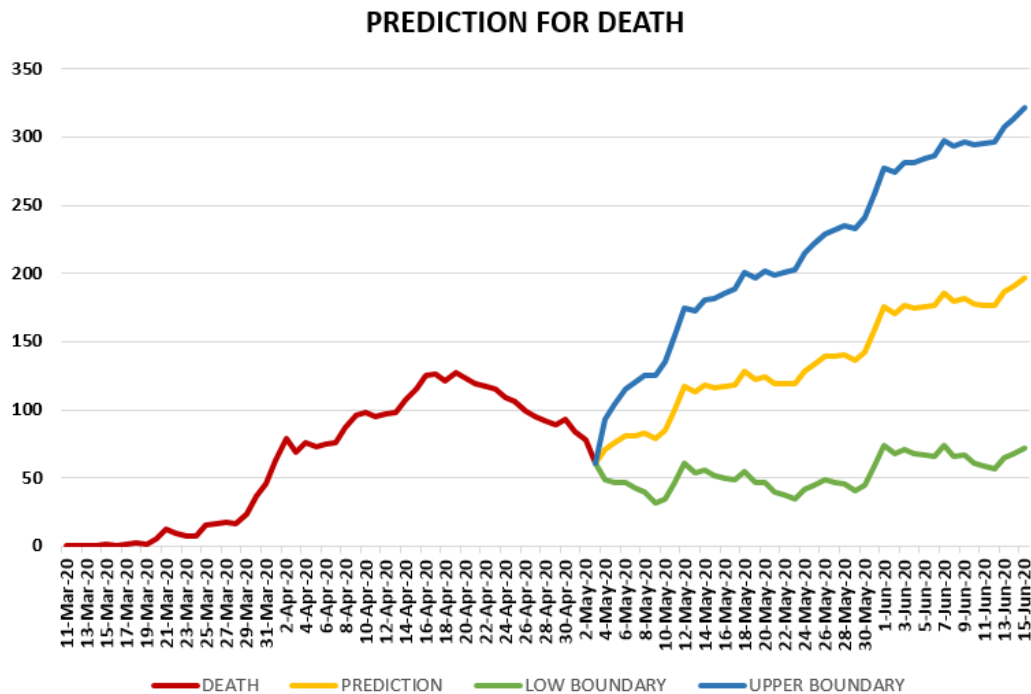
Figure 20. Prediction of daily number of deaths in Turkey using Forecast Sheet.
