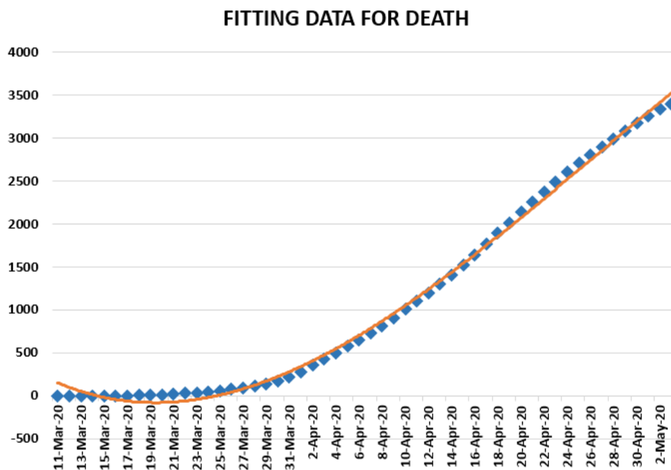
Figure 15. Polynomial fitting data for died people in Turkey from 11 March 2020 to 3 May 2020.
