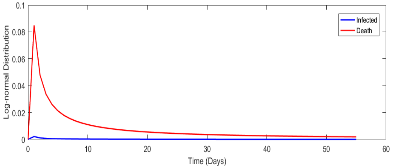
Figure 31. Lognormal distribution for all cases in South Africa.
