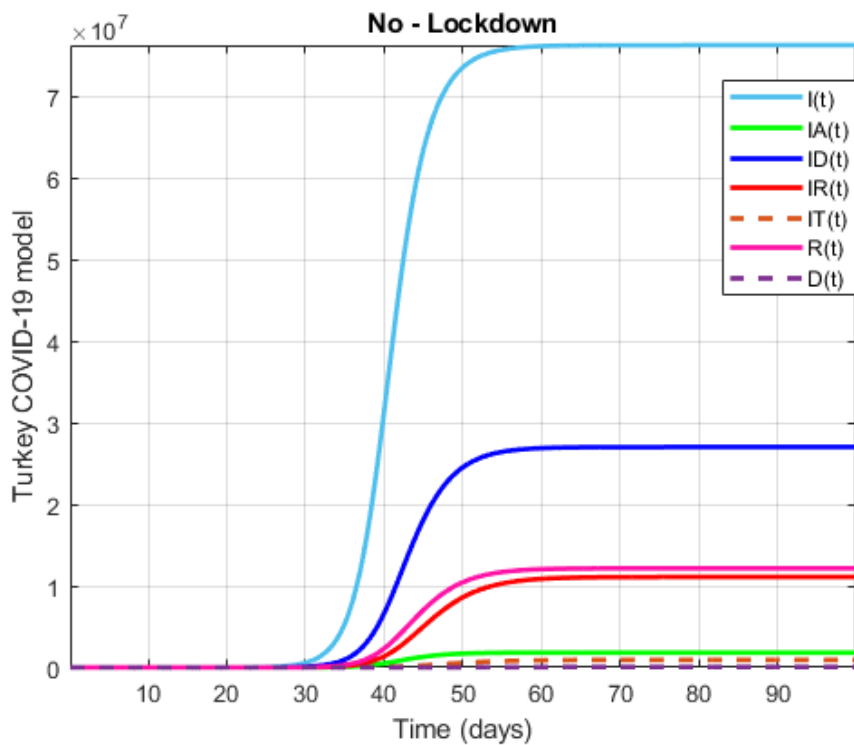
Figure 35. Numerical visualization for COVID-19 model in Turkey.
