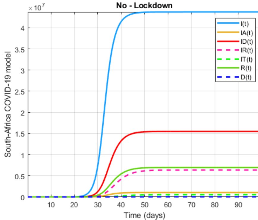
Figure 33. Numerical visualization for COVID-19 model in South Africa.
