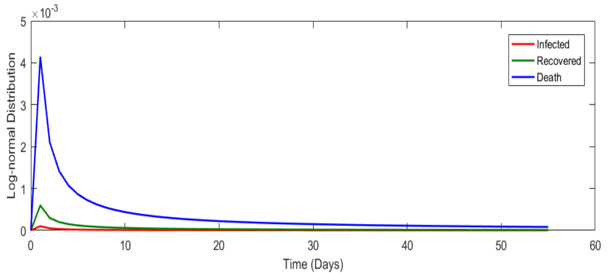
Figure 17. Lognormal distribution for all cases in Turkey from 11 March 2020 to 3 May 2020.
