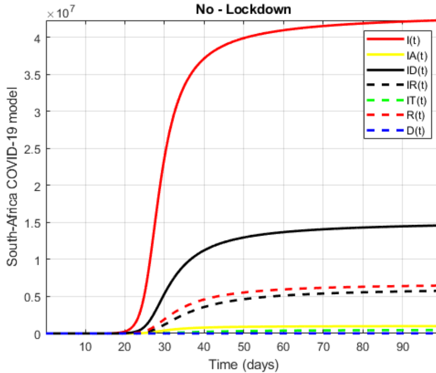
Figure 37. Numerical visualization for COVID-19 model in South Africa for \alpha = 0.75 .
