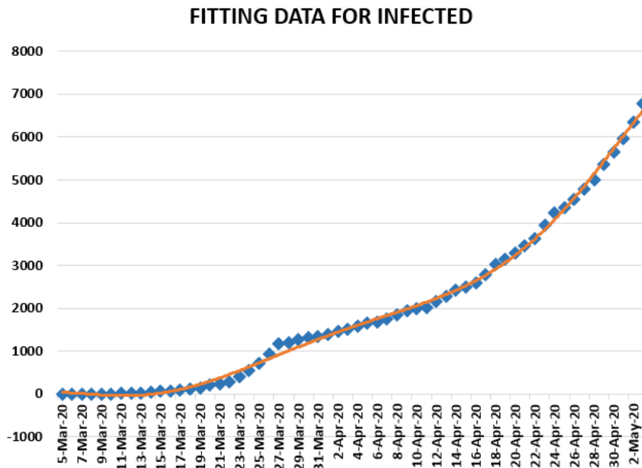
Figure 27. Polynomial fitting data for infected in South Africa from 5 March 2020 to 3 May 2020.
