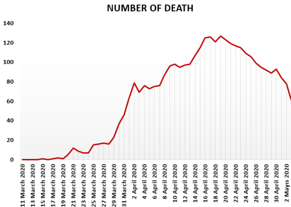
Figure 7. Number of death people in Turkey from 11 March 2020 to 3 May 2020.
