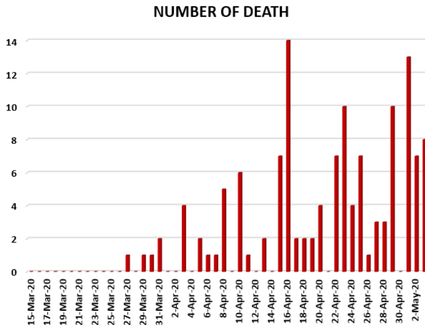
Figure 25. Number of death in South Africa from 15 March 2020 to 3 May 2020.
