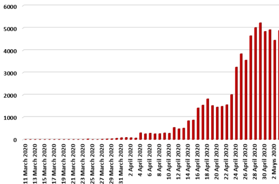
Figure 5. Number of recovered people in Turkey from 11 March 2020 to 3 May 2020.
