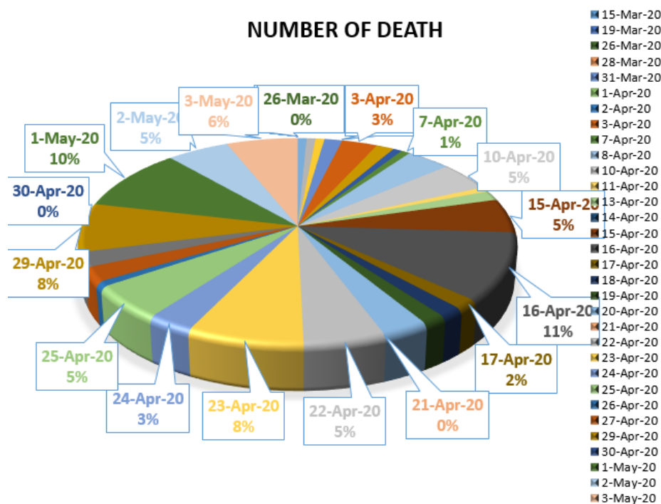
Figure 26. Number of death in South Africa from 15 March 2020 to 3 May 2020.
