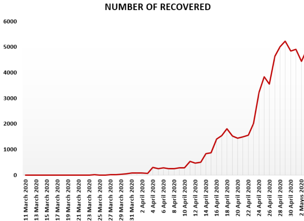
Figure 4. Number of recovered people in Turkey from 11 March 2020 to 3 May 2020.
