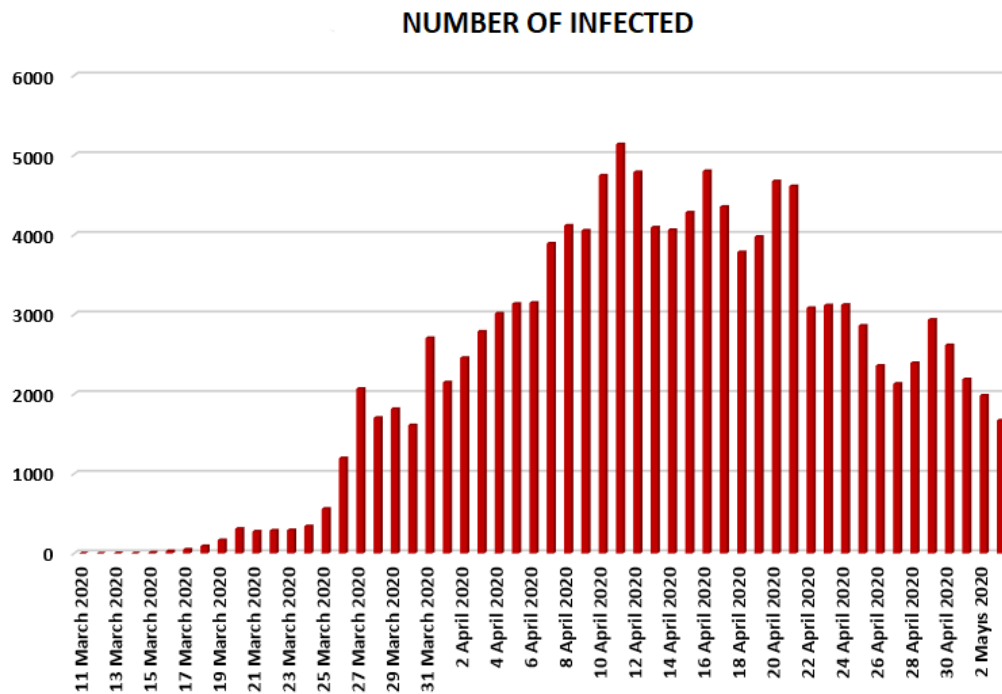
Figure 2. Number of infected people in Turkey from 11 March 2020 to 3 May 2020.
