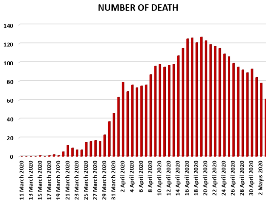
Figure 8. Number of death people in Turkey from 11 March 2020 to 3 May 2020.
