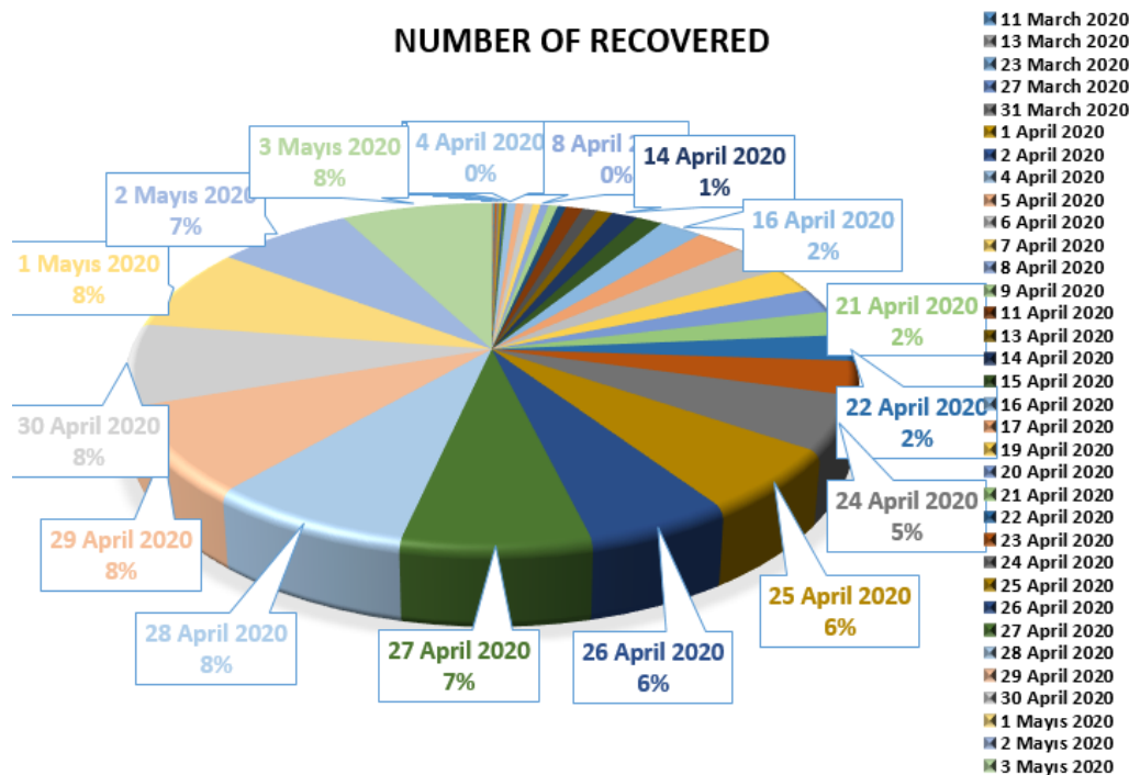
Figure 6. Number of recovered people in Turkey from 11 March 2020 to 3 May 2020.
