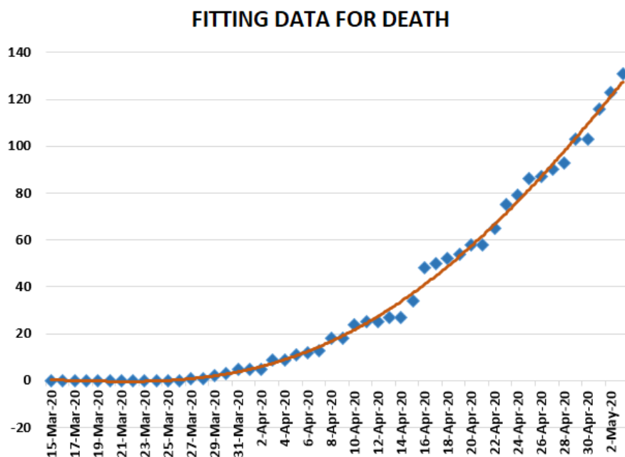
Figure 28. Polynomial fitting data for death in South Africa from 15 March 2020 to 3 May 2020.
