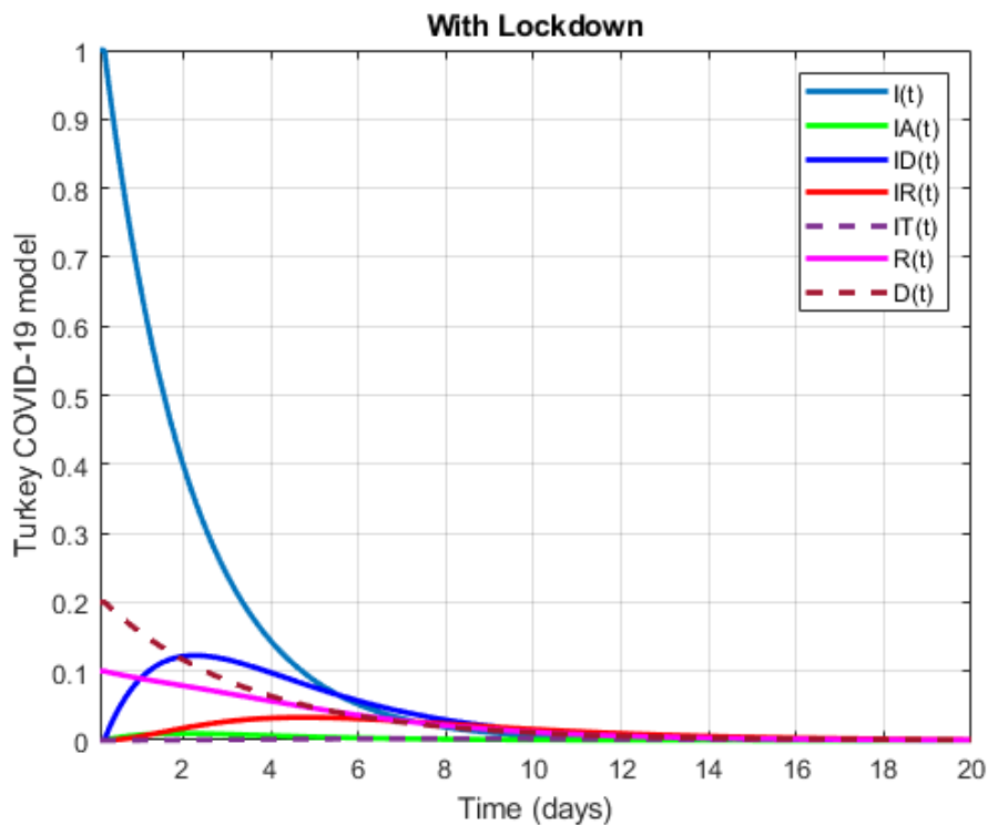
Figure 36. Numerical visualization for COVID-19 model in Turkey.
