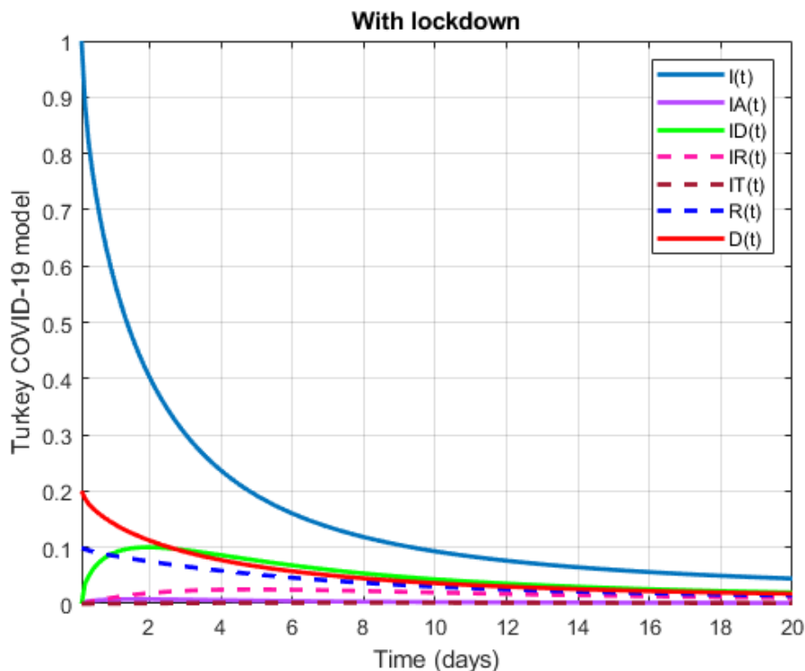
Figure 40. Numerical visualization for COVID-19 model in Turkey for \alpha = 0.8 .
