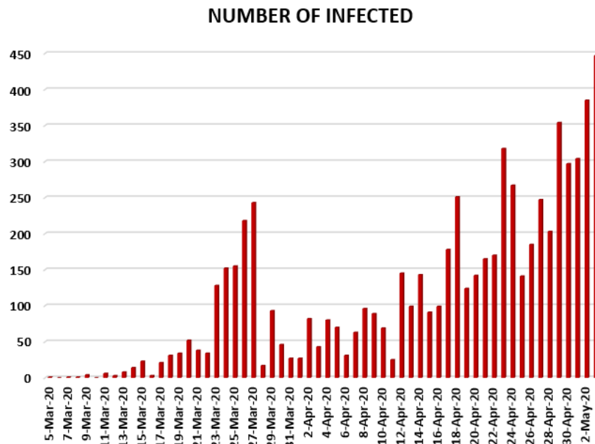
Figure 22. Number of infected people in South Africa from 5 March 2020 to 3 May 2020.
