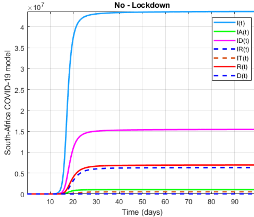
Figure 41. Numerical visualization for COVID-19 model in South Africa for \alpha = 0.9, \beta = 0.75 .
