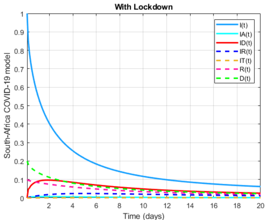
Figure 38. Numerical visualization for COVID-19 model in South Africa for \alpha = 0.75 .
