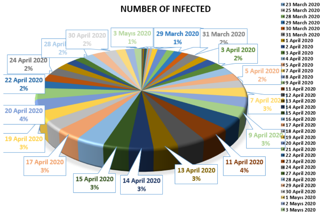
Figure 3. Number of infected people in Turkey from 11 March 2020 to 3 May 2020.
