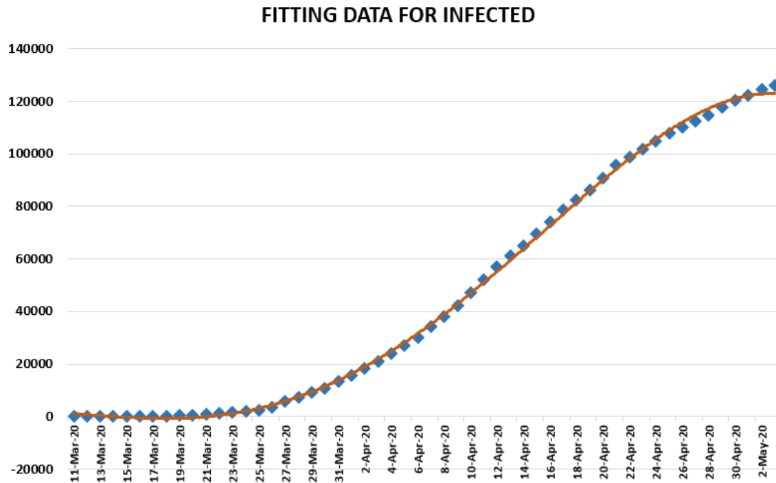
Figure 13. Polynomial fitting data for infected people in Turkey from 11 March 2020 to 3 May 2020.
