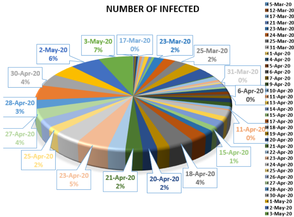
Figure 23. Number of infected people in South Africa from 5 March 2020 to 3 May 2020.
