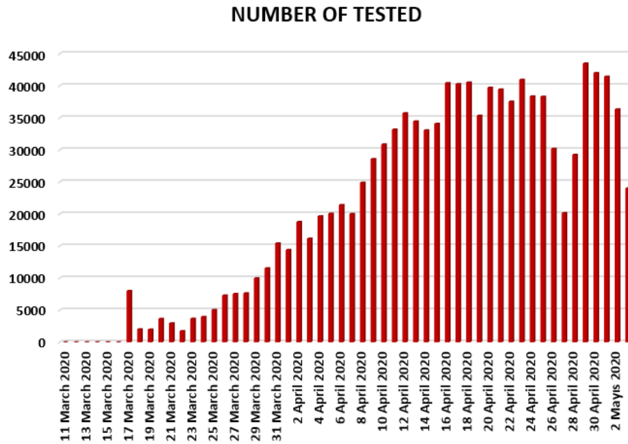
Figure 11. Number of tested people in Turkey from 11 March 2020 to 3 May 2020.
