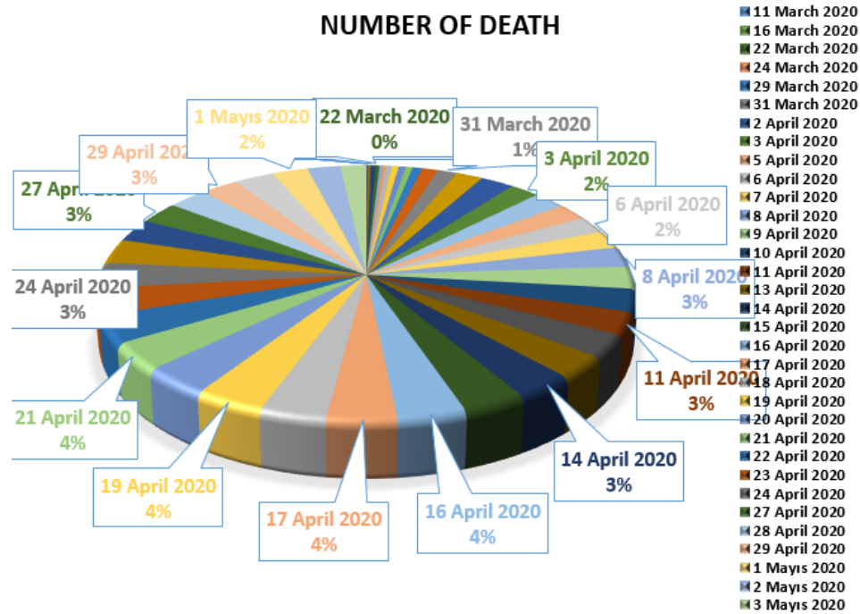
Figure 9. Number of death people in Turkey from 11 March 2020 to 3 May 2020.
