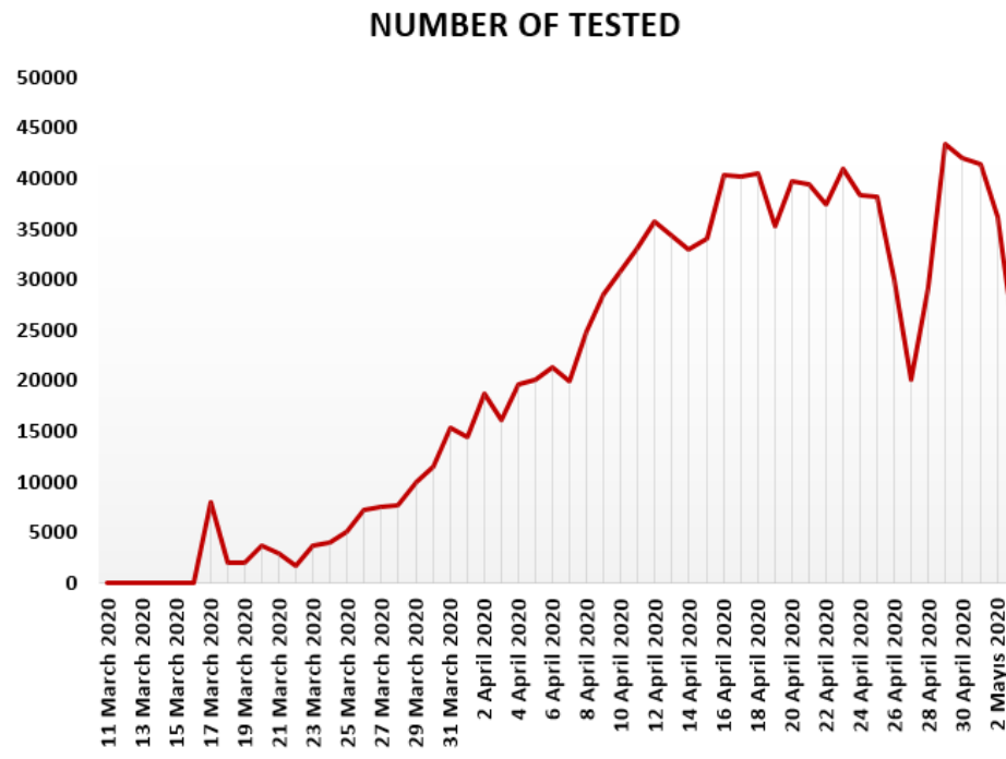
Figure 10. Number of tested people in Turkey from 11 March 2020 to 3 May 2020.
