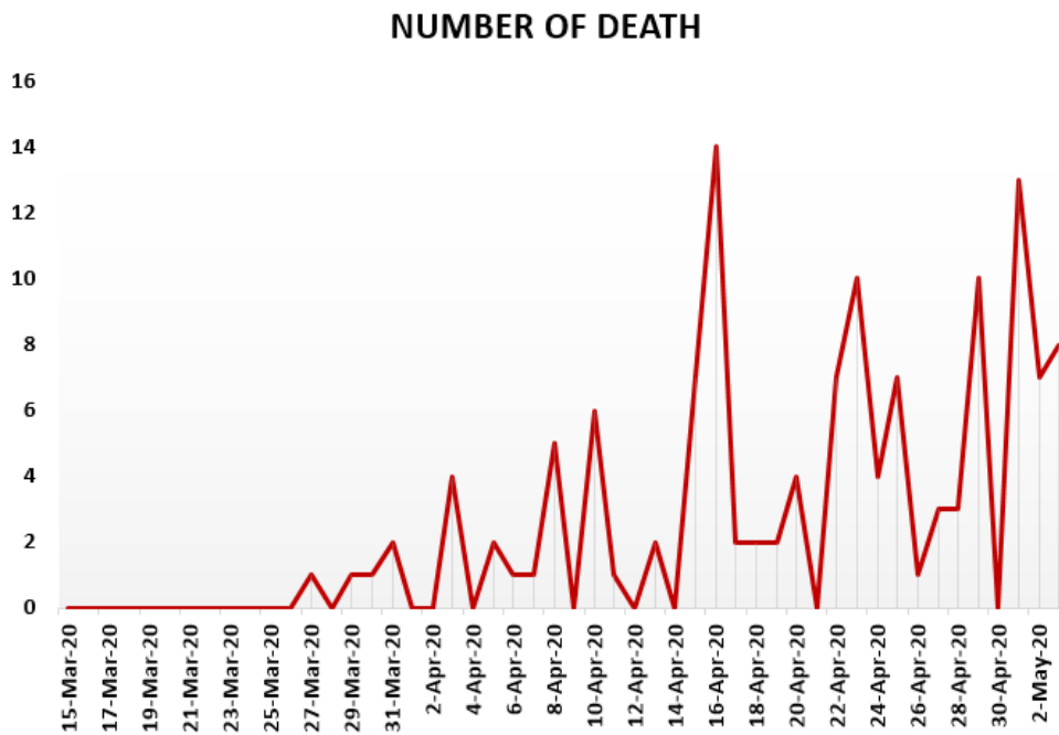
Figure 24. Number of death in South Africa from 15 March 2020 to 3 May 2020.
