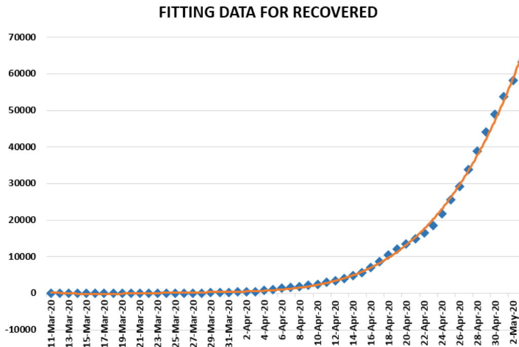
Figure 14. Polynomial fitting data for recovered people in Turkey from 11 March 2020 to 3 May 2020.
