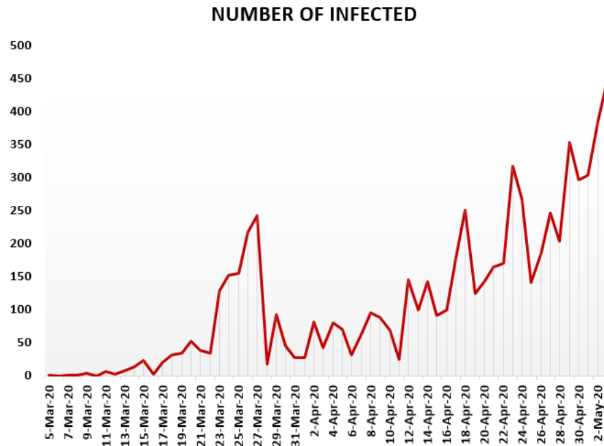
Figure 21. Number of infected people in South Africa from 5 March 2020 to 3 May 2020.
