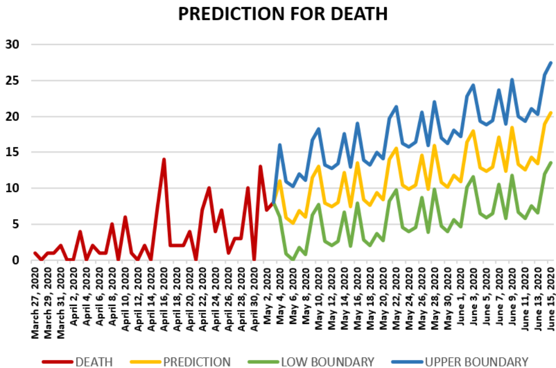
Figure 30. Prediction of daily number of deaths in South Africa using Forecast Sheet.
