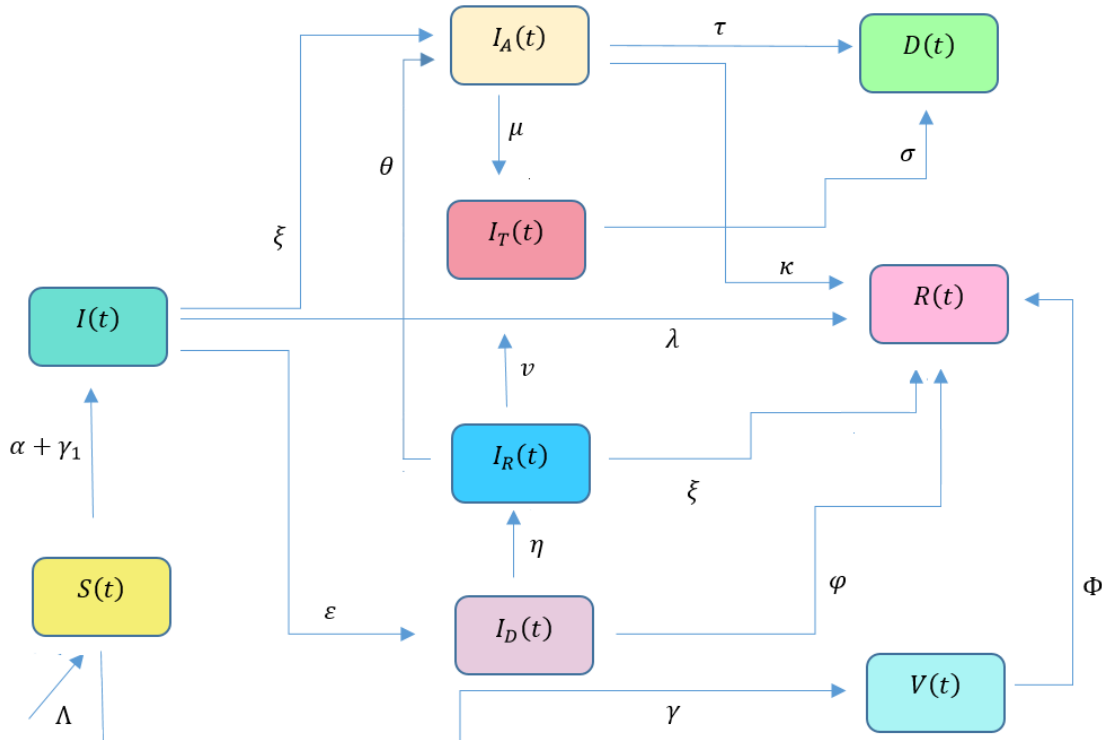
Figure 32. Diagram summarizing COVID-19 model given by the system (3.1).
