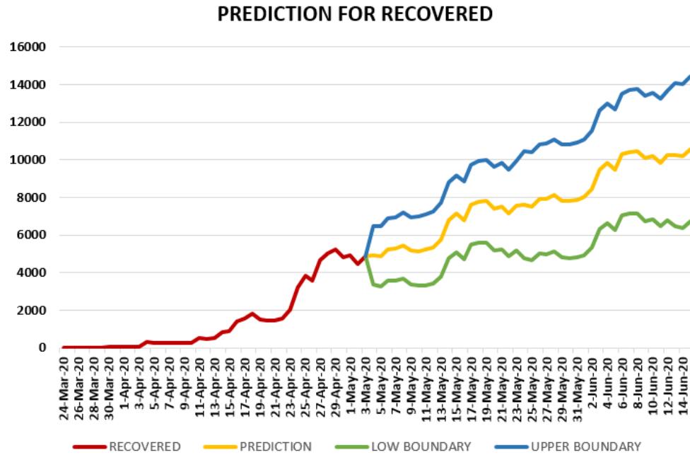
Figure 19. Prediction of daily number of recovered in Turkey using Forecast Sheet.
