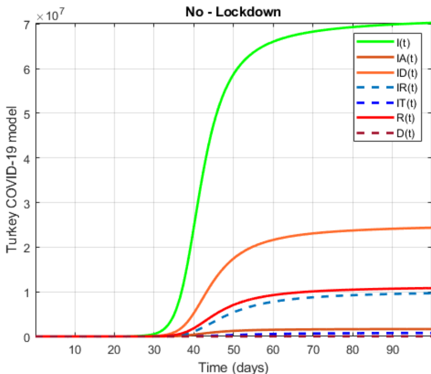
Figure 39. Numerical visualization for COVID-19 model in Turkey for \alpha = 0.8 .
