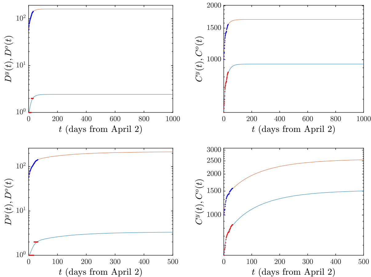
FIG. 3: Again the Deaths D(t) and the cumulative infections C(t) are given for the case where the c factor (characterizing the number of contacts) amongst young individuals is doubled, but those of the older individuals (and of the young-older interaction) are kept fixed. This is shown in the top panels. In the bottom panels, the c 's of both young and old individuals are doubled.
