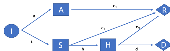
FIG. 1: Flowchart of the populations considered in the model and the rates of transformation between them. The corresponding dynamical equations are Eqs. (1)–(6).
