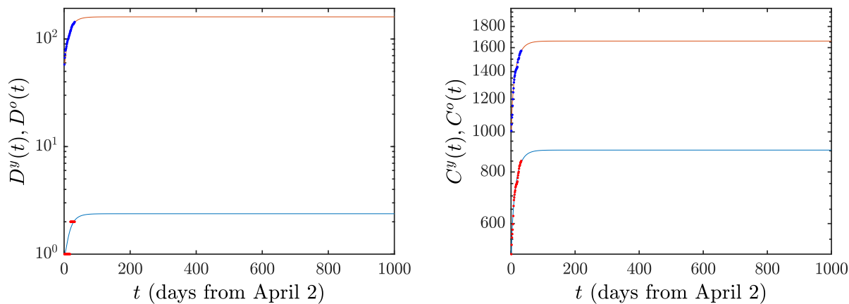
FIG. 2: Evolution of the current situation of deaths D(t) (left) and cumulative infections C(t) (right) in Greece, under the unrealistic assumption of the indefinite continuation of lockdown conditions. In this and all the figures that follow, the blue curve corresponds to the young population, while the red curve to the older population. The data for Greece from the 3rd of April to the 4th of May 2020 are depicted by dots. For the latter, alternate colors have been used (i.e., blue dots for the older population and red for the younger for clearer visualization).
