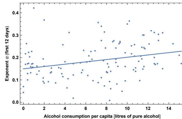
Figure 11: Exponent \alpha for each country vs. alcohol consumption. We show the data points and the best-fit for the linear interpolation.
