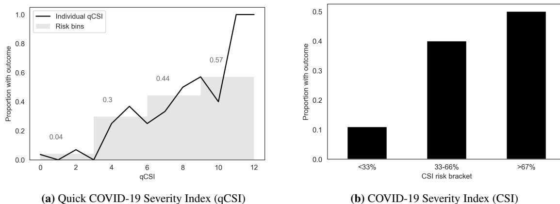
Figure 4: Calibration of qCSI and CSI on external validation dataset. (a) Each patient in the validation cohort was assigned a score by qCSI, and the percentage who had a critical respiratory illness outcome were plotted with a line plot. Patients were then grouped into risk bins by qCSI intervals (0-3, 4-6, 7-9, 10-12) and the percentage of patients in each group with the outcome is indicated in the bar plot. (b) Each patient in the validation cohort was assigned a CSI, a percent risk from 0 to 100% using gradient boosting and isotonic regression. The percent of patients with CSI scores of 0-33%, 33-66%, and 66-100% who experienced critical respiratory illness at 24 hours are shown.
