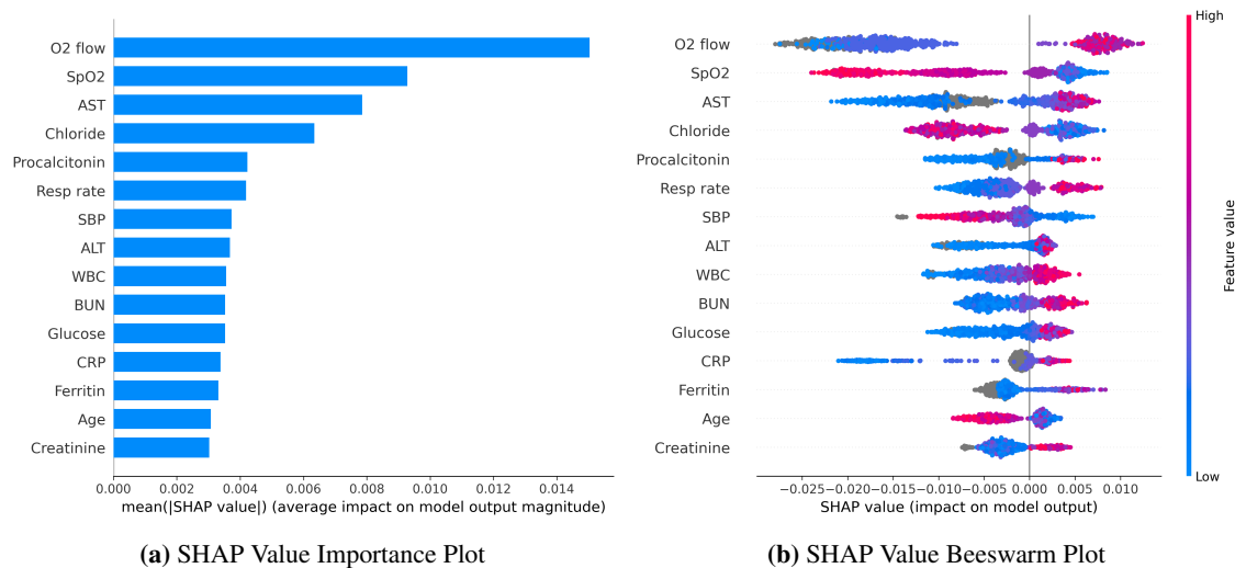
Figure 2: SHAP variable importance and beeswarm plots. (a) Mean absolute SHAP values suggest a rank order for variable importance in the CSI. (b) In the beeswarm plot, each point corresponds to an individual person in the study. The points position on the x-axis shows the impact that feature has on the model's prediction for a given patient. Color corresponds to relative variable value.
