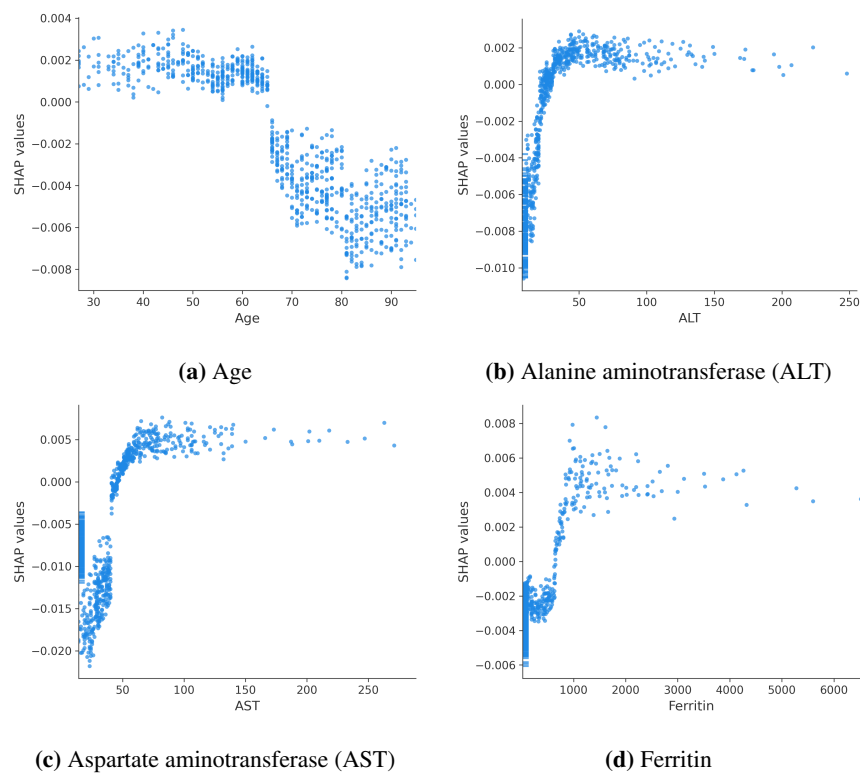
Figure 3: SHAP value plots for (a) age, (b) alanine aminotransferase, and (c) aspartate aminotransferase, and (d) ferritin. Scatter plots show the effects of variable values (x-axis) on the model predictions as captured by SHAP values (y-axis).
