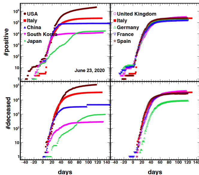
Figure 1. Number of positive (top panels) and deceased (bottom panels) as function of time for different countries indicated in the inset. Time t=0 was suitably chosen to match the exponential growth for the number of positive and it was kept the same for all the other plots, figures 1,3.
