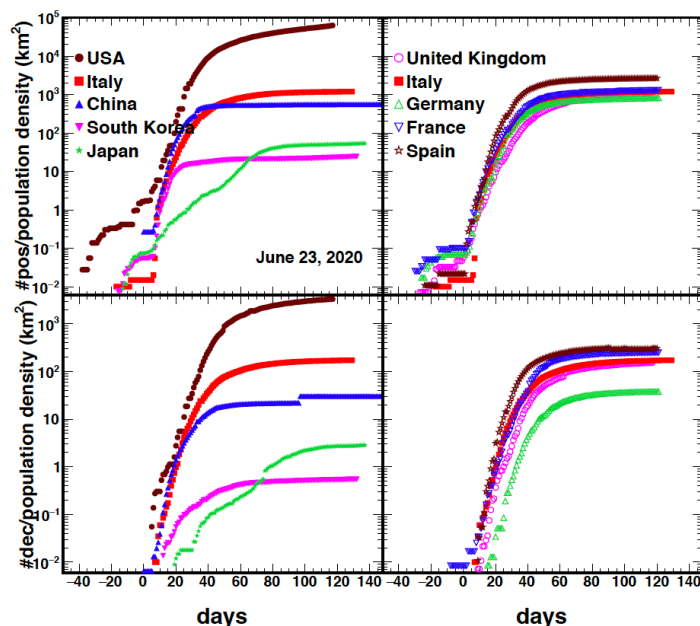
Figure 2. Number of cases divided by the population density of each country vs time, compare to figure 1.
