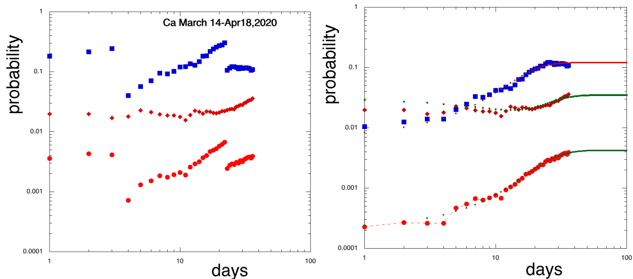
Figure 7. Positive (square symbols) and deceased (circle symbols) probabilities vs time in days. The rhomb symbols represent the ratio deceased/positive independent on the number of tests. The right panel is obtained after renormalization, see text.
