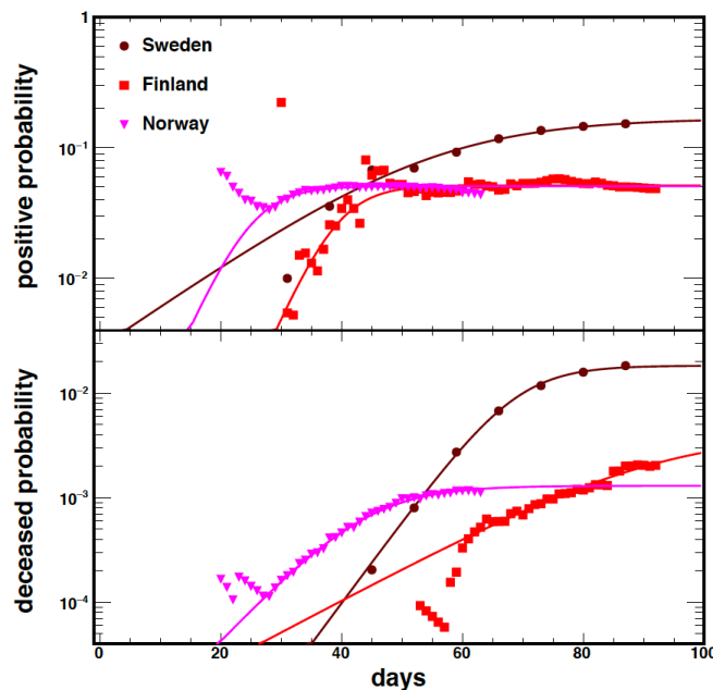
Figure 11. Probabilities as function of time for the countries indicated in the inset. Sweden is adopting the natural selection option resulting in higher probabilities compared to nearby countries. Different starting data depend on which day the complete information needed for the plot was released. Updates are given in figure A5.
