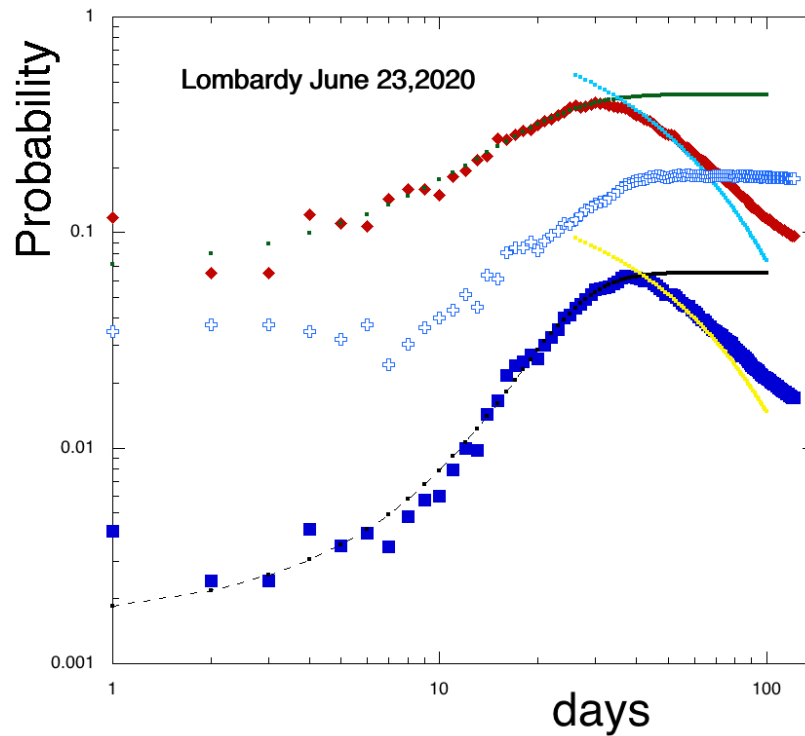
Figure A1. Same as figure 4 for the Lombardy case. The original model predictions are given by the full lines. Notice the data increase respect to the prediction at later times due to the reopening of normal activities: a situation to monitor attentively.
