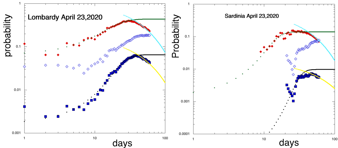
Figure 4. Probability for positive (rhomb symbols) or deceased (square symbols) vs time in days for the Lombardy (left) and Sardinia (right) regions. The open crosses give the ratio positive/deceased and reach almost 20% for Lombardy [8]. The continuous points are obtained from eq.(1) and the exponential decay from eq.(2). Updated data are given in figure A1.
