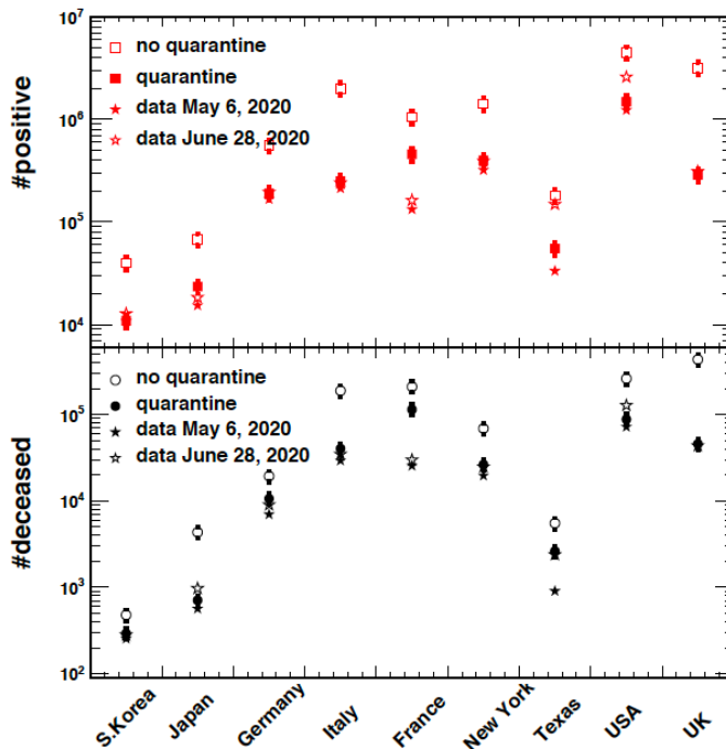
Figure 10. Number of positive (top panel) and deceased (bottom panel) for the countries indicated on the abscissa. Predictions without quarantine measures refer to June 28, 2020. The numerical data are reported in table AI.
