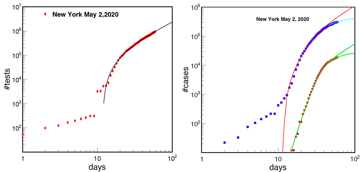
Figure 9. Same as figures 5 and 6 for the state of New York.
