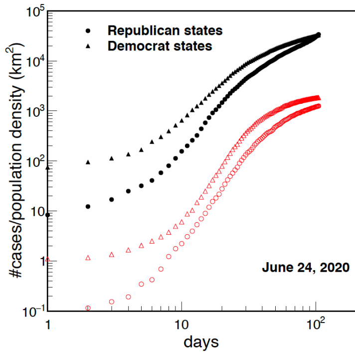
Figure A4. Same as figure A3 but for the number of cases divided the population density, compare to figure 2.
