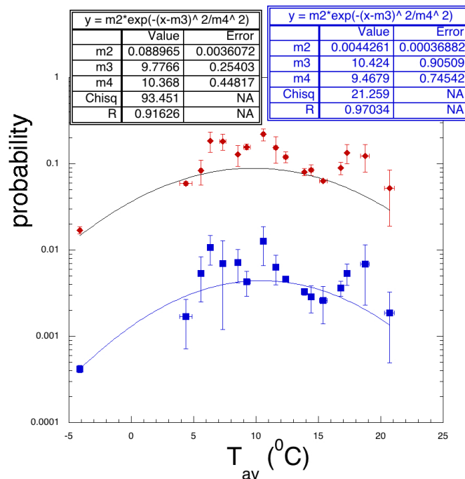
Figure 12. Positive (rhomb symbols) and deceased (square symbols) probabilities vs average temperature of the US states in the spring season. The data to calculate the probabilities were collected on May 3,2020. To get better statistics, averages were performed over states differing about 1 °C. Enforced Gaussian fits are also included and the fit parameters given in the inset.
