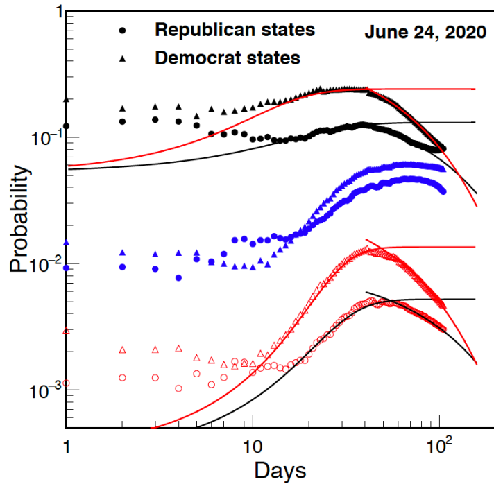
Figure A3. Positive (full symbols) and deceased (open symbols) probabilities for US states with different party governor. The democratic case is dominated by the high population density state of New York, see figure 8. The striking different behavior explains the prediction discussed in fig.10 regarding the USA. Notice an increase at later times for the republican states suggesting a too early reopening. Recall that there is a time delay for the deceased respect to positive.
