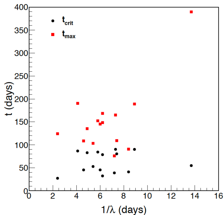
Figure 13. t_{\max} & t_{\text{crit}} vs 1/\lambda for all cases analyzed in this paper. The largest values of t_{\max} & 1/\lambda refer to Sweden while the largest value of t_{\text{crit}} refers to the USA. All the numerical values of this figure are reported in table AIII.
