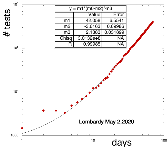
Figure 5. Total number of tests as function of time for Lombardy. The fitting function and its values are displayed in the insets.
