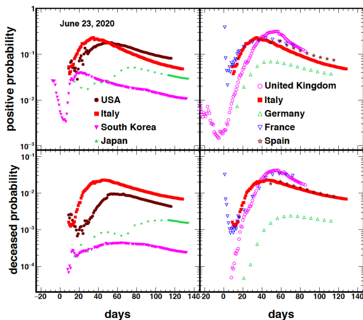
Figure 3. Probabilities vs time for the countries indicated in the inset. Some countries stopped providing the number of tests performed daily (France on May 5 th and the UK on May 22 nd ), other countries are providing this information periodically (Spain, Germany).
