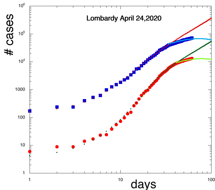
Figure 6. Predicted cases with and without quarantine as function of time, see text. Data for positive and deceased are given by the square and circle symbols respectively.
