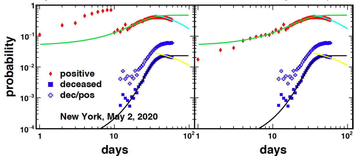
Figure 8. Same as figure 7 for the state of New York. See figure A2 for an update.
