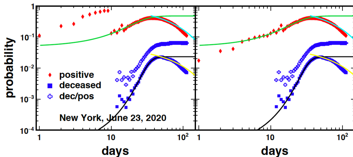
Figure A2. Same as figure 8 updated to June 23, 2020. A small decrease respect to the prediction from eq.(1) and (2) is observed at later times.
