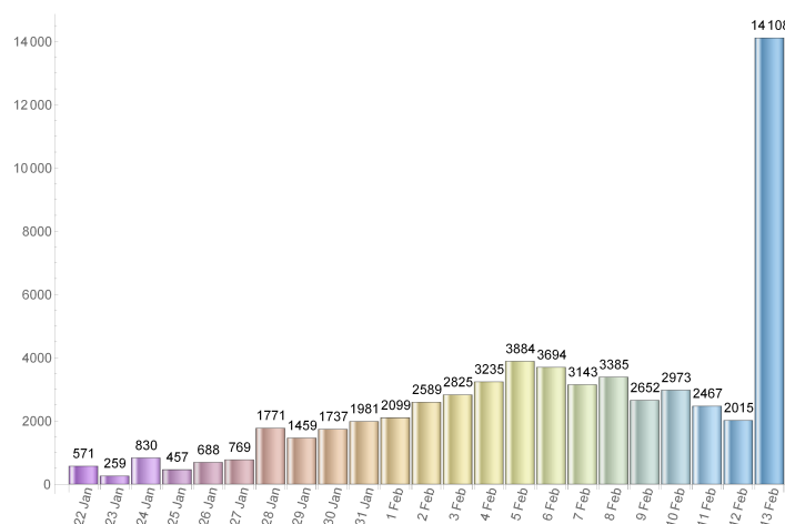
FIGURE 3. Number of new cases in China between Jan 22 nd and Feb 13 th .
