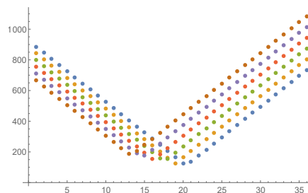
FIGURE 6. The values of the norms of the difference I_{sp} - I_w for several values of \mu \in (0.08, 0.085) and of K \in (5, 100, 6, 500) .
