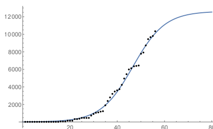
FIGURE 4. Total number of infected individuals fitting the data for São Paulo (updated to April 21 st ).
