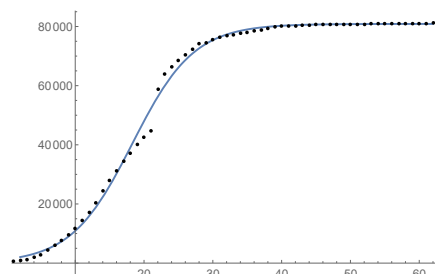
FIGURE 2. The function of the total number of infected individuals in Wuhan, fitting the data updated to April 21 st .
