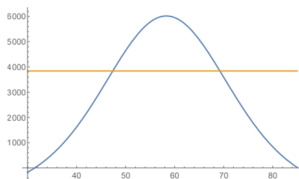
(fig3) FIGURE 5. The number of simultaneously infected individuals in a period of 15 days (disregarded the casualties).
