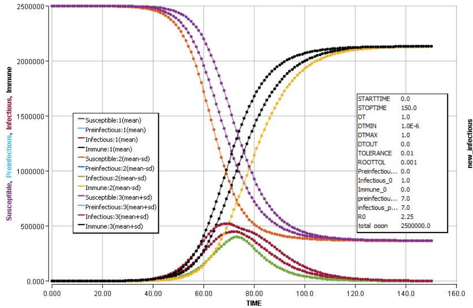
Figure 7. Simulation for SIR model
