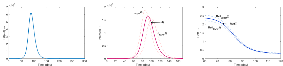
Figure 10. SEIR with E and I infectious
