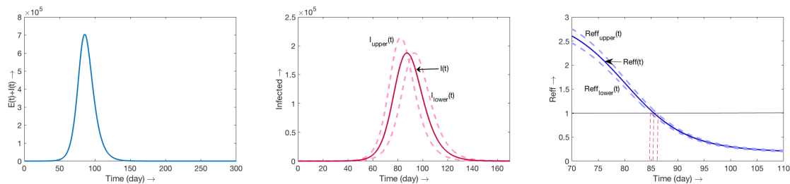
Figure 9. SEIR with only I infectious
