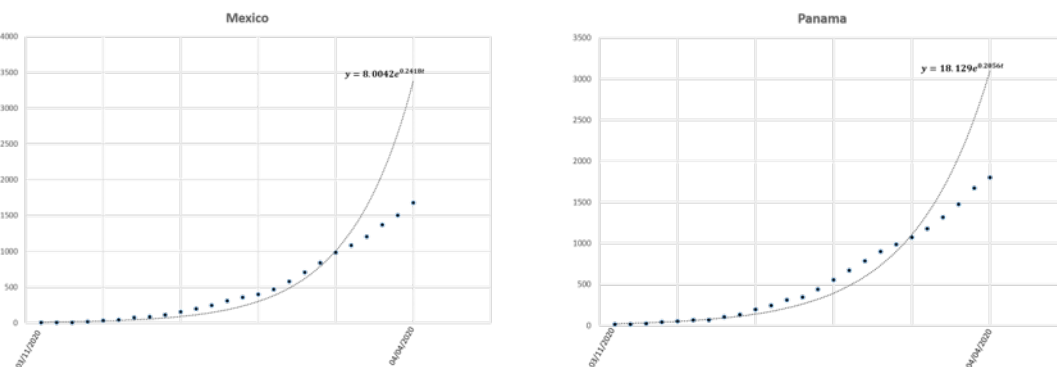
Figure 12. Exponential fitting for data from Mexico and Panama
