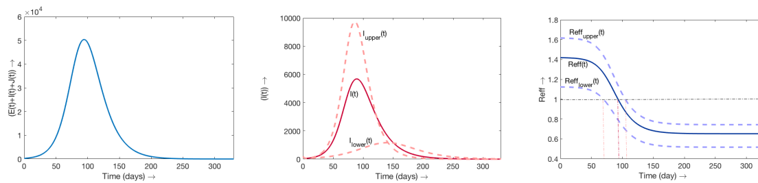
Figure 5. SEIR-J.
