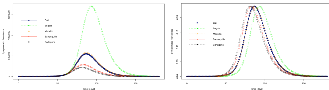
Figure 6. Comparison of outbreaks in 6 major cities of Colombia using SEIR_Q1Q2Q3 model
