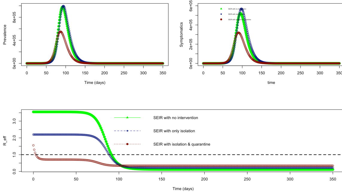
Figure 4. SEIR-Q1Q2Q3 Model results. Showing total cases and effective reproduction number
