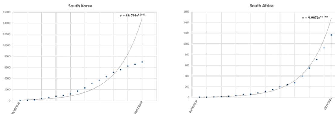
Figure 11. Exponential fitting for data from South Korea and South Africa
