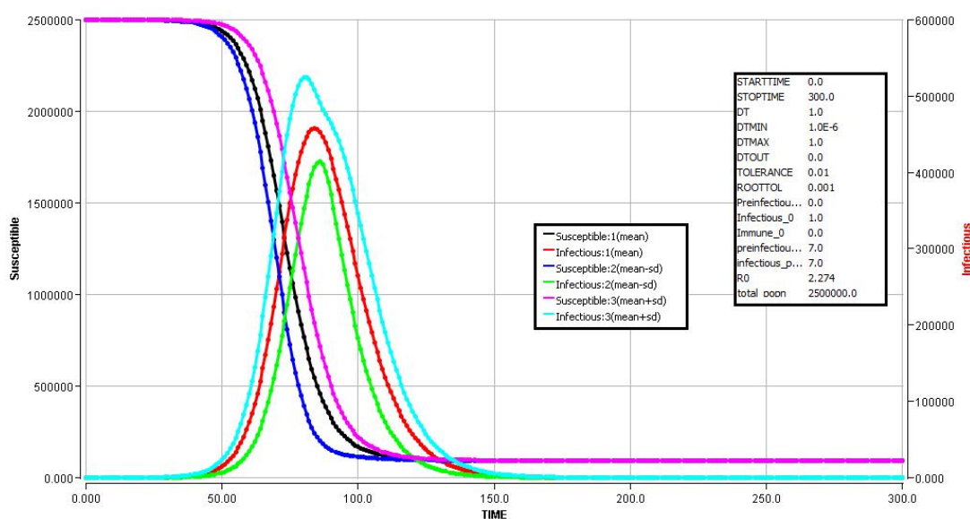
Figure 3. Simulation for SEIR model with E and I both infectious
