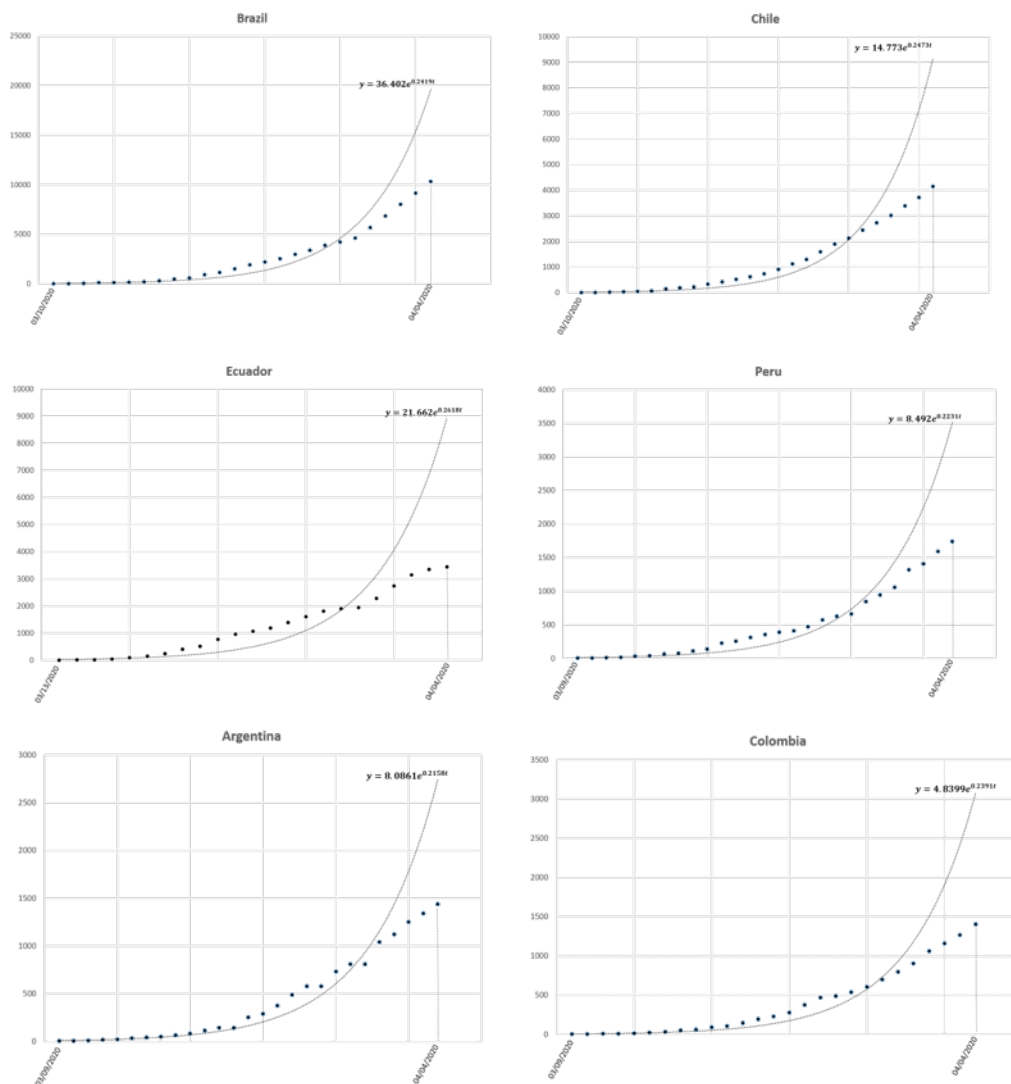
Figure 13. Exponential fitting for data from six South America countries
