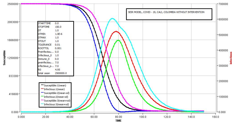
Figure 8. Simulation for SEIR model with only I infectious
