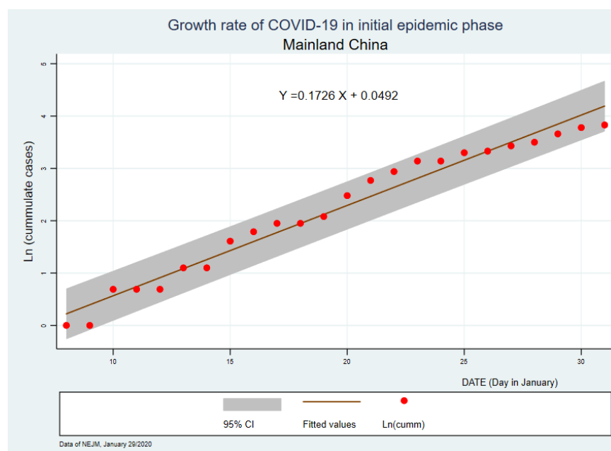
Figure 2. Growth rate of Covid-19 in initial epidemic phase
