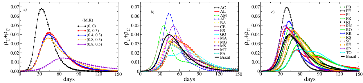
FIG. 4. a) Evolution of the epidemic prevalence in the total population for different mitigation measures controlled by parameters (M, K) . b,c) Epidemic prevalences for the 26 federative states of Brazil under a moderate mitigation approach with (M, K) = (0.4, 0.3) . Day 0 corresponds to March 31, 2020.
