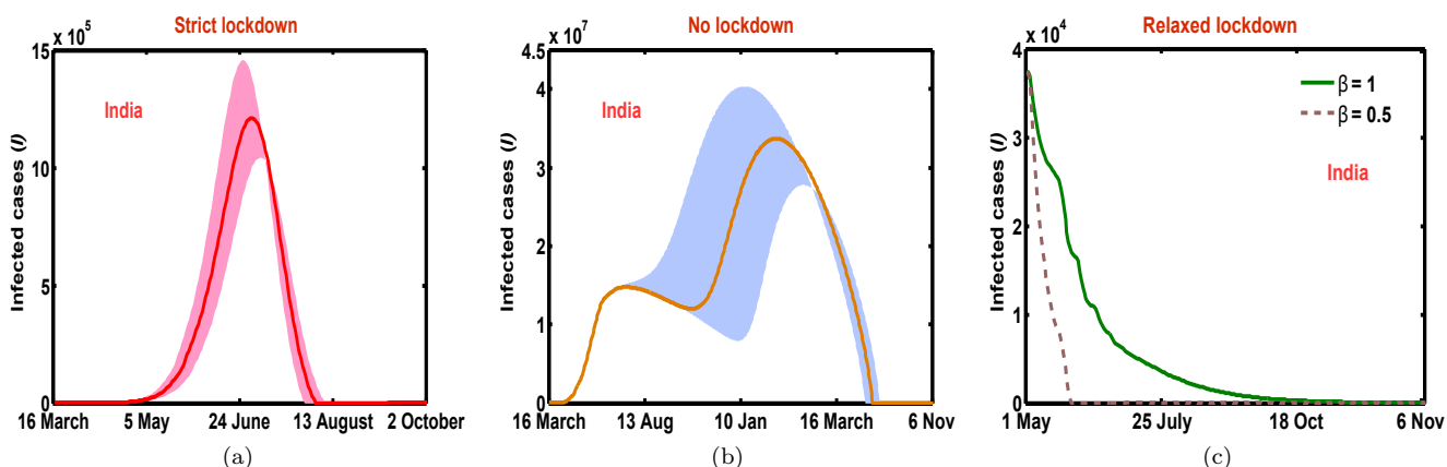
Figure 4: (Color online) Infectious cases ( I ) with respect to time (in days) in different cases (a) strict lockdown (b) no lockdown (c) relaxed lockdown. The parameters are (intrastate population migration factor, interstate population migration factor, \beta ) = (0.34, 0, 3.319), (0.8, 0.6, 9), (0.34, 0.10, 0.5, 1) in (a-c) with common parameters \tau = 8.8 , \mu = 0.0412 , \delta = 0.22 , \sigma = 1/7 , \epsilon = 0.85 , and \gamma = 0.034 . The shaded region in (a-b) is the bound for the fitted model with respect to \tau \in [6, 12] . In (b) the dates 10 Jan, 16 March, 6 Nov belong to year 2021 while remaining dates are from current year 2020.
