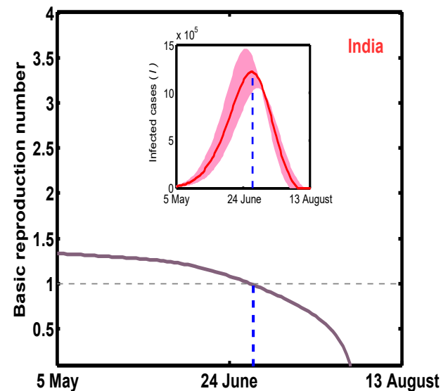
Figure 5: (Color Online) Basic reproduction number with respect to time in presence of strict lockdown for intrastate population migration factor = 0.34, interstate population migration factor = 0, \beta = 3.319 , \tau = 8.8 , \mu = 0.0412 , \delta = 0.22 , \sigma = 1/7 , \epsilon = 0.85 , and \gamma = 0.034 . The inset figure shows infectious cases as in Fig. 4(a) with time for same parameters.
