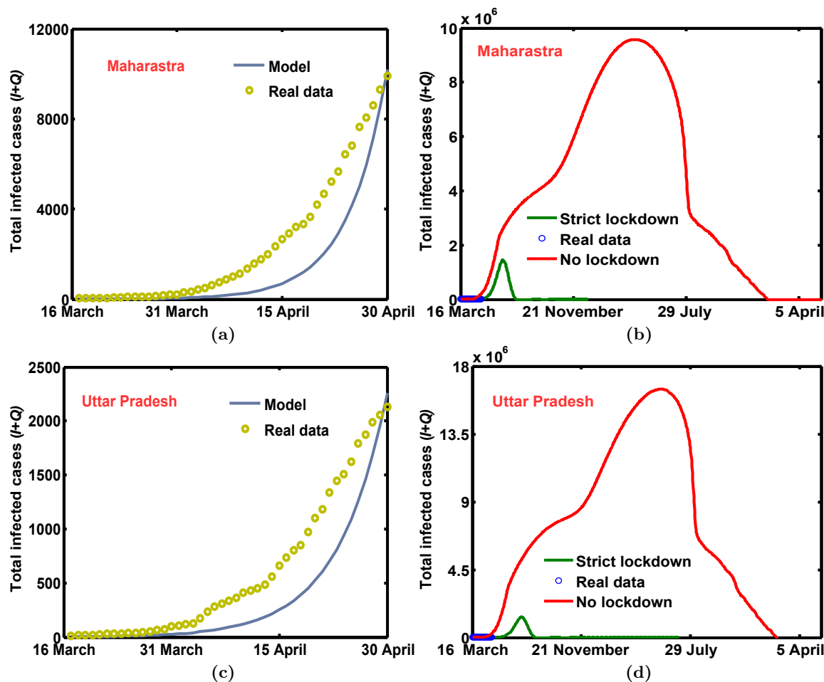
Figure 6: (Color Online) Panels (a) and (c) show fitting of the actual available total COVID-19 infected cases (yellow marker) ( I + Q ) for Maharashtra and Uttar Pradesh, respectively from 16 March to 30 April, 2020 by the proposed model results (blue). Panels (b) and (d) show total infected cases ( I + Q ) in Maharashtra, and Uttar Pradesh, respectively with respect to time (in days) in case of strict (green) and no lockdown (red). Blue marker represents the real data. The parameters for (a) and green curve in (b) are: (intrastate population migration factor, interstate population migration factor, \beta, \tau ) = (0.41, 0, 3.4, 7) while in case of no lockdown (red) the chosen values are (0.8, 0.6, 9, 7). In (c) and green curve in (d) these values are (0.393, 0, 3, 8.2) while in case of no lockdown (red) the chosen values are (0.8, 0.6, 9, 8.2). \mu = 0.0412 , \delta = 0.22 , \sigma = 1/7 , \epsilon = 0.85 , and \gamma = 0.034 are same in (a-d). In (b) and (d), 29 July, and 5 April belong to 2021, and 2022, respectively.
