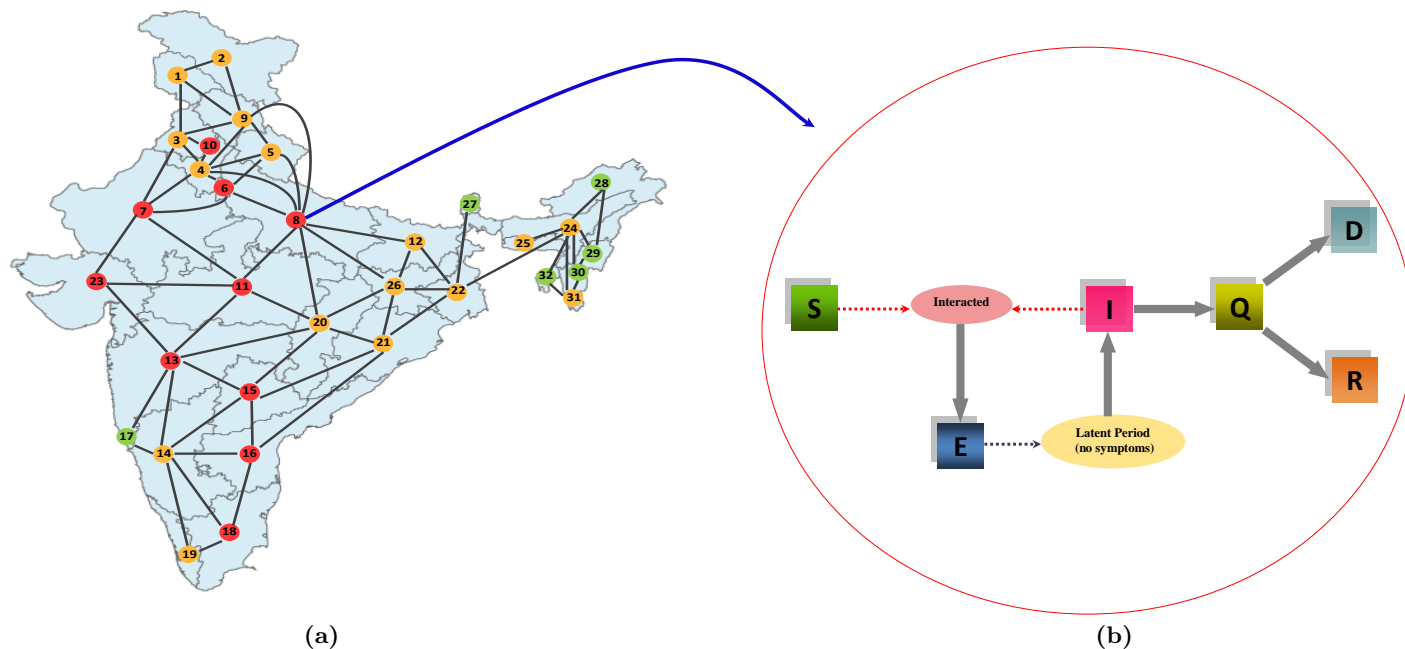
Figure 1: (a) The map of India along with different states (represented by filled dots, numbered from 1 to 32*). The solid lines shows the connections of a state with its neighboring states resulting in inter state movements. The states with more/less than 2000 cases as on April 30, 2020 are shown by red/orange color. COVID-19 free states are represented by green color. The complete dataset reflecting state wise population distribution is provided in Appendix (C) in Table II. *Note that in the study we have not considered a few Indian states and Union Territories including Lakshadweep, Dadra and Nagar Haveli, Daman and Diu, Andaman and Nicobar Islands and Puducherry on account of their comparatively low population density. (b) Within a state, Schematic of SEIQRD Model with time delay.
