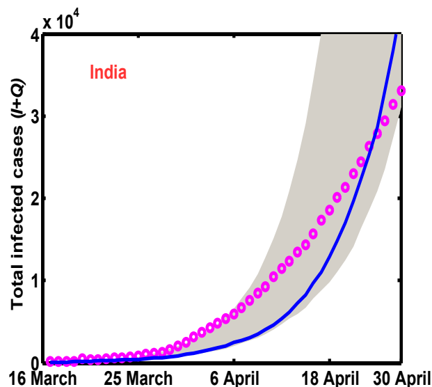
Figure 2: (Color Online) Fitting of the actual available total COVID-19 infected cases ( I + Q ) shown in pink colored markers for India from 16 March to 30 April, 2020. Solid blue line represents the fitted curve with parameters: intrastate population migration factor = 0.34, interstate population migration factor = 0, \beta = 3.319 , \tau = 8.8 , \mu = 0.0412 , \delta = 0.22 , \sigma = 1/7 , \epsilon = 0.85 , and \gamma = 0.034 . The shaded region is the bound for the fitted model with respect to \tau \in [6, 12] .
