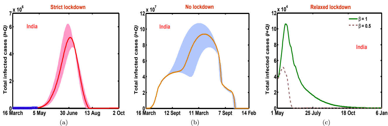
Figure 3: (Color online) Total infected cases ( I + Q ) with respect to time (in days) in different scenarios (a) strict lockdown (b) no lockdown (c) relaxed lockdown. In (a) blue line represents real data from 16 March to 30 April, 2020. The parameters are (intrastate population migration factor, interstate population migration factor, \beta ) = (0.34, 0, 3.319), (0.8, 0.6, 9), (0.34, 0.10, 0.5, 1) in (a-c) with common parameters \tau = 8.8 , \mu = 0.0412 , \delta = 0.22 , \sigma = 1/7 , \epsilon = 0.85 , and \gamma = 0.034 . The shaded region in (a-b) is the bound for the fitted model with respect to \tau \in [6, 12] . In (b) the dates 11 March, 7 Sept are for year 2021, 14 Feb for 2022; in (c) 6 Jan belong to year 2021; while remaining dates are from 2020.
