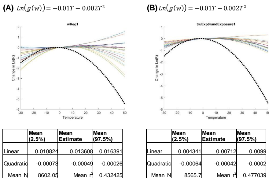
Figure S10: Impact of using weighted regression (A) vs. unweighted (B)
