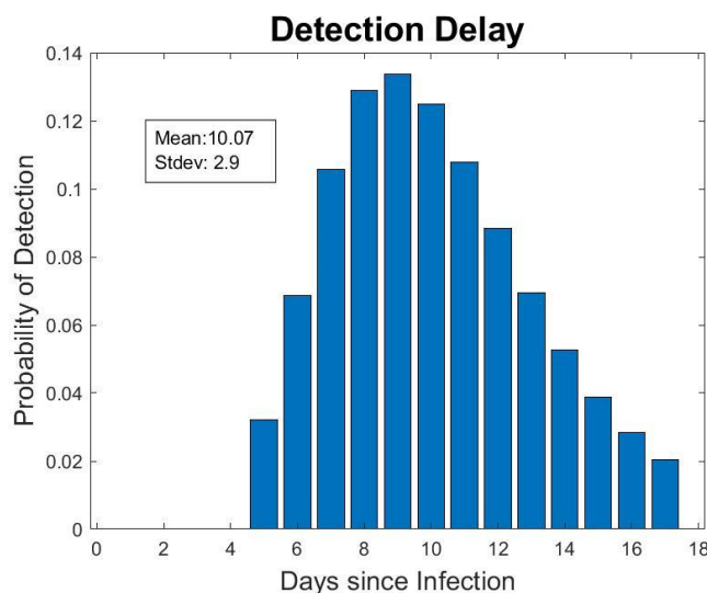
Figure S4: Distribution of Detection Delay
