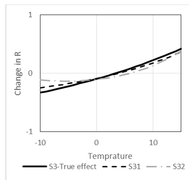
S31 - With fixed-effect
