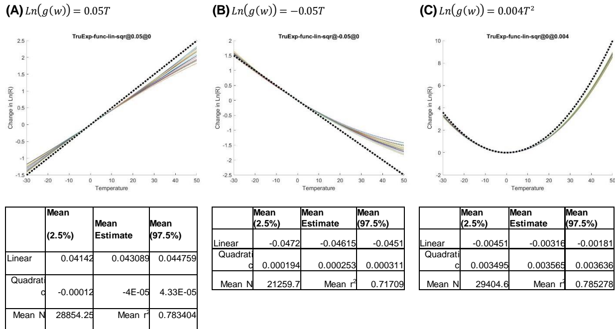
Figure S6: Performance of estimation method, provided with true infections, in identifying different functional relationships between weather and reproduction.
