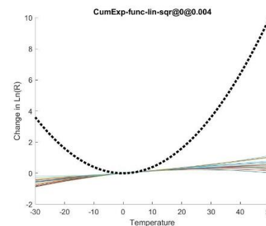
(C) \text{Ln}(g(w)) = 0.004T^2
