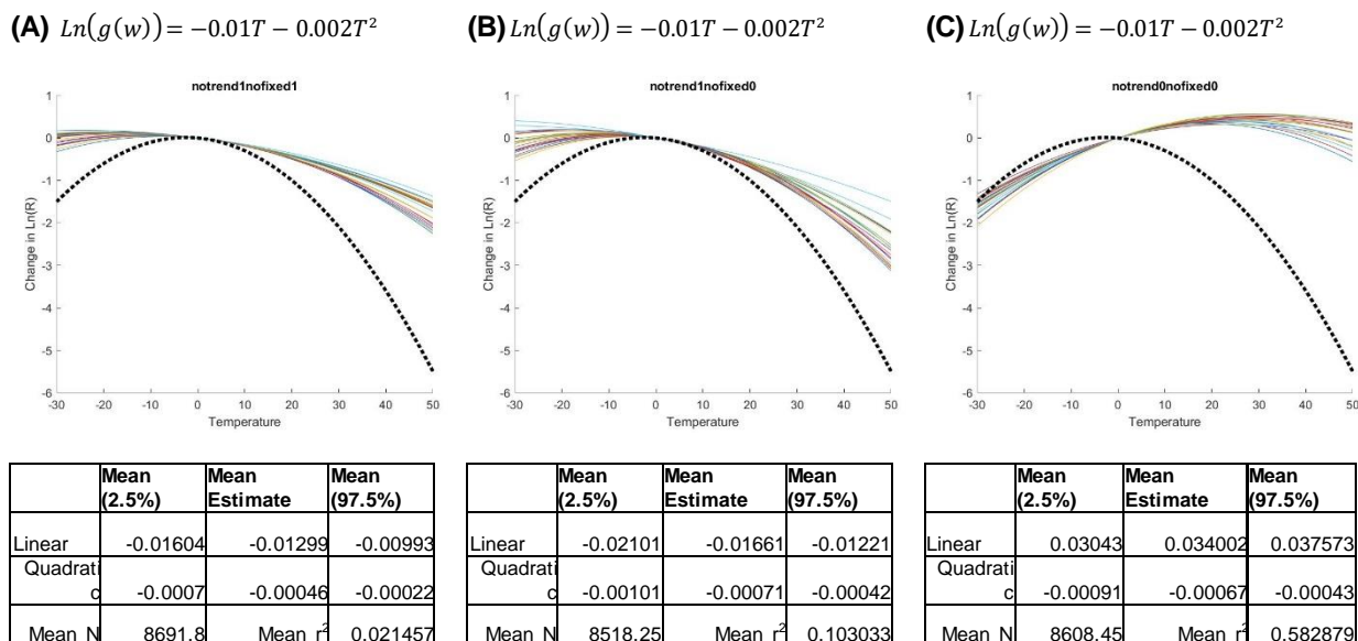
Figure S9: Comparing the use of no fixed or trend effects (A), only fixed effects without trends (B), and both location specific fixed and trend effects.
