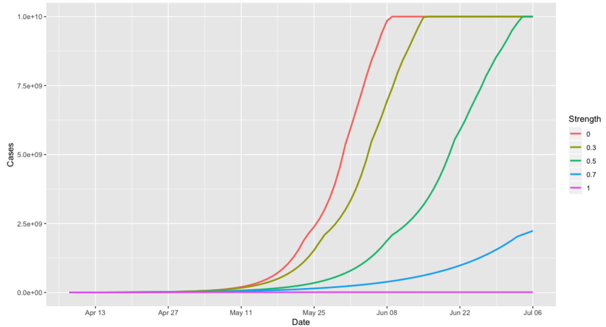
Figures S1. Counterfactual numbers of cases of Covid-19 over time worldwide to respond the interventions with values 0.3, 0.5, 0.7 and 1.
