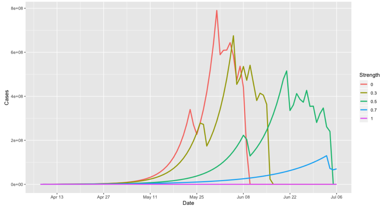
Figure S2. Time-case plot of Covid-19 worldwide under four invention scenarios
