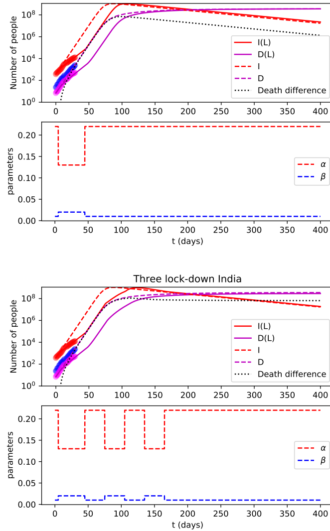
Figure 6: Top most panel shows the effect of a single 40 days long lock-down according to the SIR model simulation (different lines). The second top-most panel shows the temporal variation of \alpha and \beta adjusted according to the lock-down duration to best match the observed data (shown by circles). The bottom two figures show the same thing but for three lock-down scenario (see text for details).
