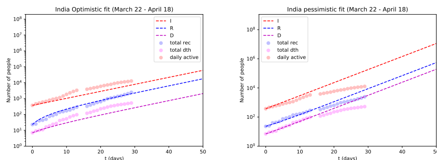
Figure 2: Comparison of SIR(D) model simulation (various lines) to the measured data (circles) for India during the period 22 March - April 18. The left panel corresponds the optimistic fit with \alpha = 0.135 , \beta = 0.03 , and \gamma = 0.0035 and the right panel corresponds the pessimistic fit with \alpha = 0.22 , \beta = 0.01 , and \gamma = 0.0035 .
