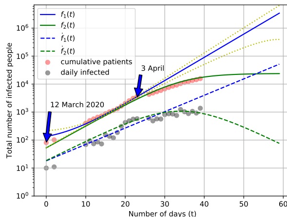
Figure 1: Functional fit to the measured data for the total infected people as a function of time (days). The best fit for f_1(t) and its derivative was obtained by using python libraries. Two yellow dotted lines show the two sigma deviation from the best fitted values. The fit for f_2(t) is done by eye estimation.
