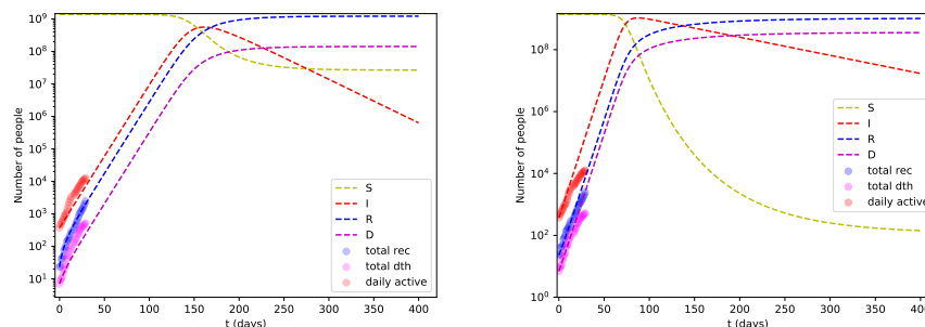
Figure 3: Prediction for India from the SIR(D) model simulation for two different scenarios and assuming no lock-down imposed. The left plot corresponds to the optimistic case whereas the right panel corresponds to the pessimistic case (see text for details).
