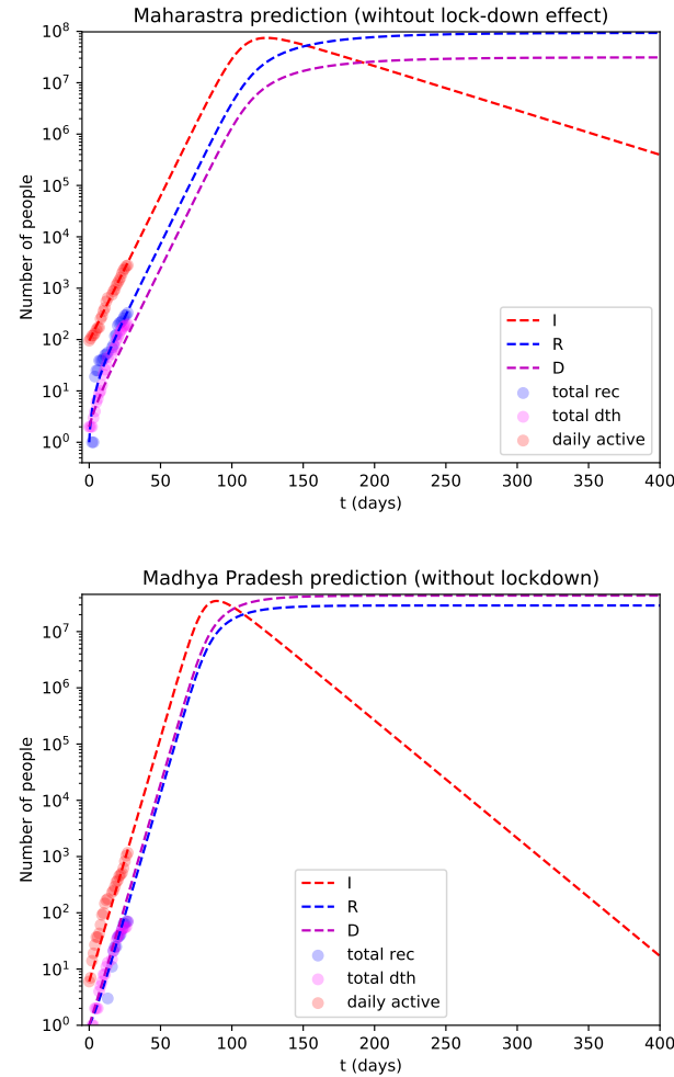
Figure 4: Predictions from the SIR(D) model simulation (mostly pessimistic prediction) for Maharashtra (top panel) and Madhya Pradesh (bottom panel). The values of the constants taken are \alpha = 0.15 , \beta = 0.015 \gamma = 0.005 for Maharashtra and \alpha = 0.25 , \beta = 0.02 \gamma = 0.03 for Madhya Pradesh.
