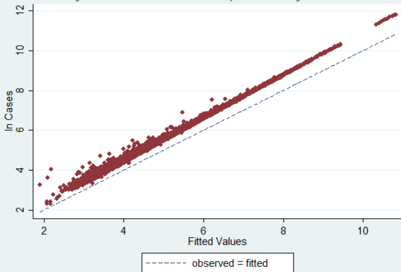
Figure 2 - Observed and Fitted Values of Dynamic Panel Regression of Cases
