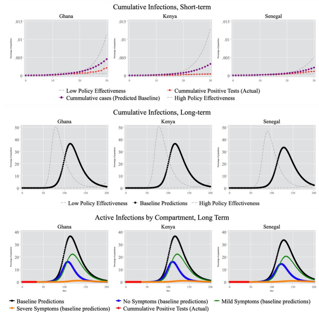
Figure 3: Projection of Active Infections
