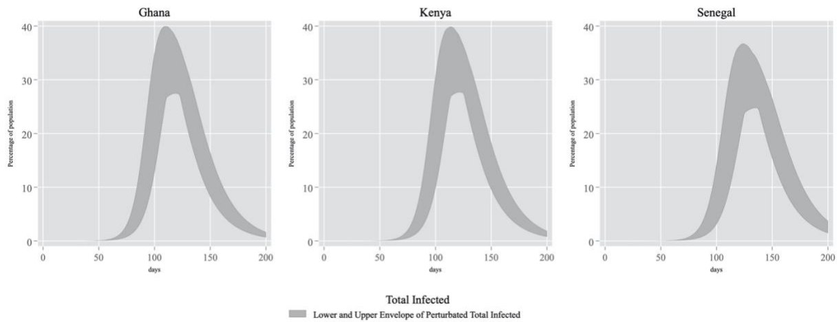
Figure 2: Sensitivity of Active Cases to Perturbations of R_t
