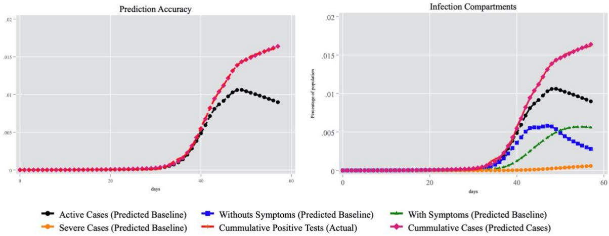
Figure 1: Benchmark, South Korea
