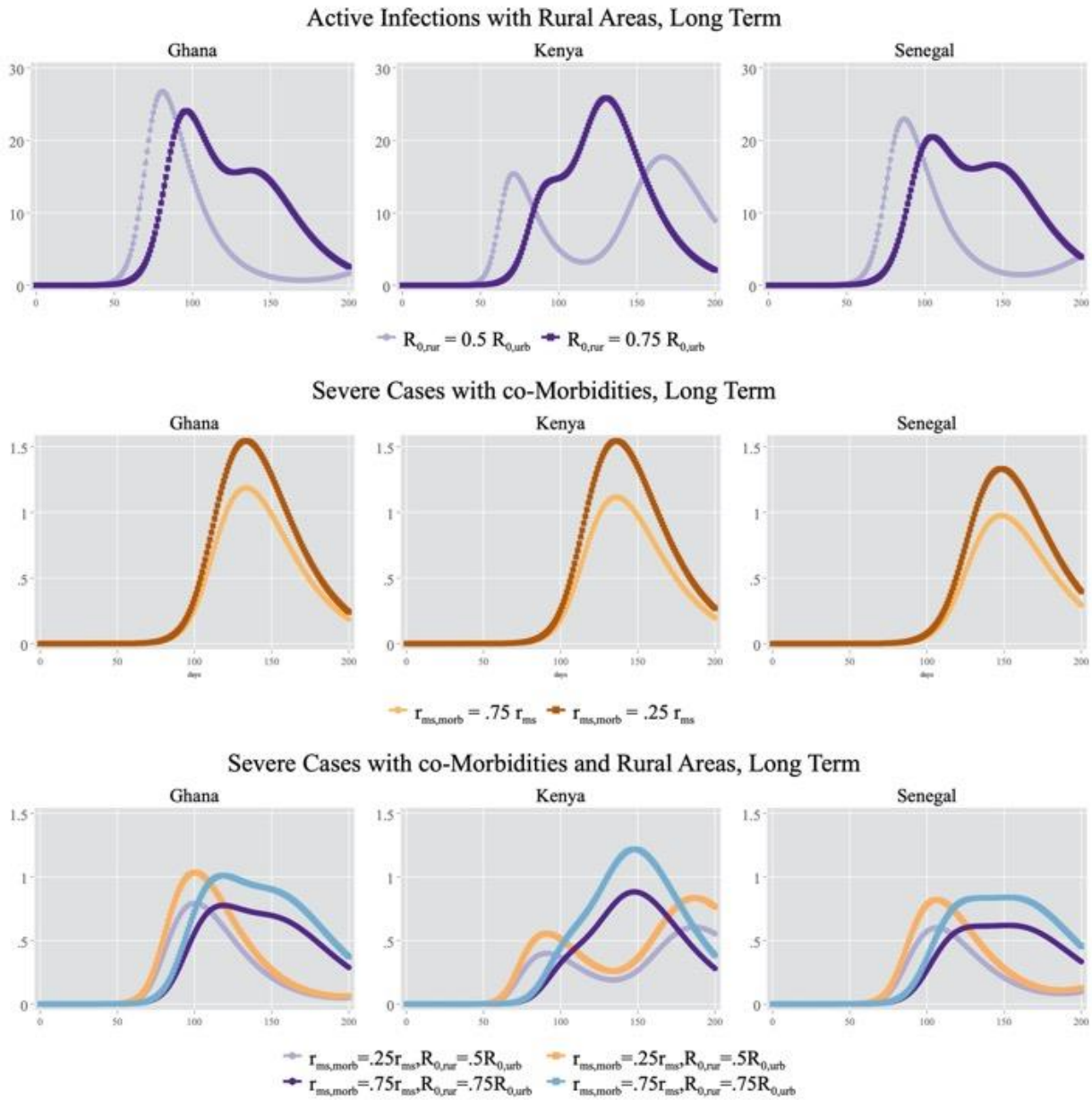
Figure 4: Projected Active Infections Accounting for Underlying Conditions and Rural Areas
