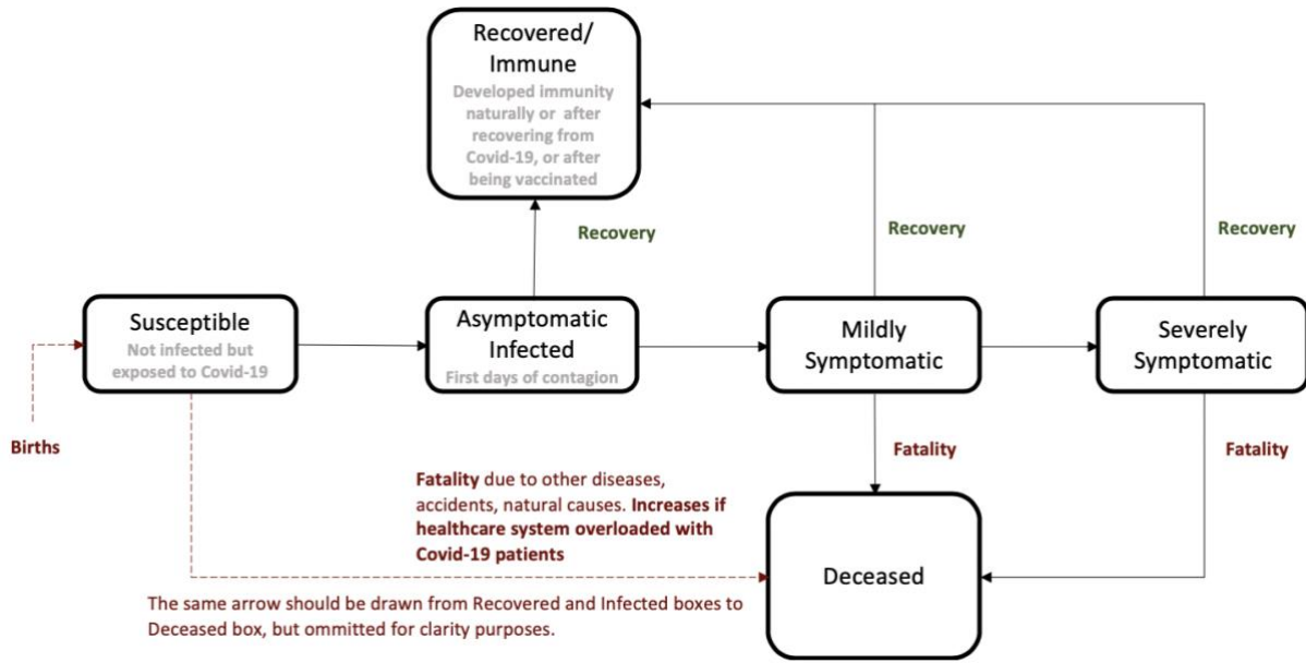
Figure 1: Visual representation of the model
