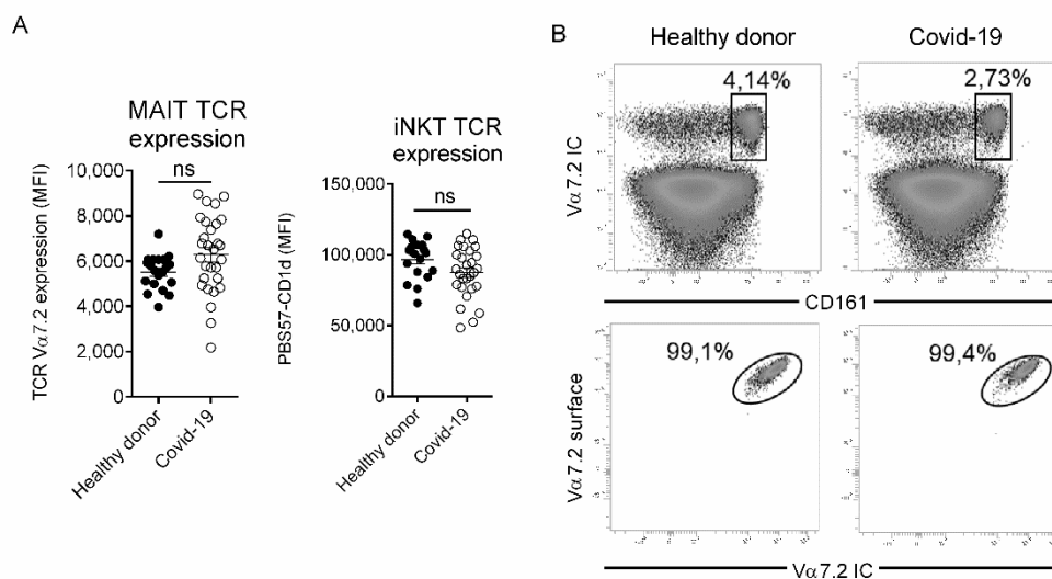
451 Supplemental Figure 2: Evaluation of TCR internalization in MAIT and iNKT cells. A, 452 Mean intensity fluorescence of TCR expression on MAIT and iNKT cells from control (n = 20) 453 or Covid-19 patients (n = 30) based on TCR Vα7.2 and PBS57-CD1d tetramer staining 454 respectively. Individuals and means ± SEM are shown. B, Flow cytometry analysis of TCR 455 Vα7.2 expression using surface vs intracellular staining. Representative dot plots of 4 control 456 and 4 Covid-19 patients are shown. ns, not significant; ***, p<0.001.
