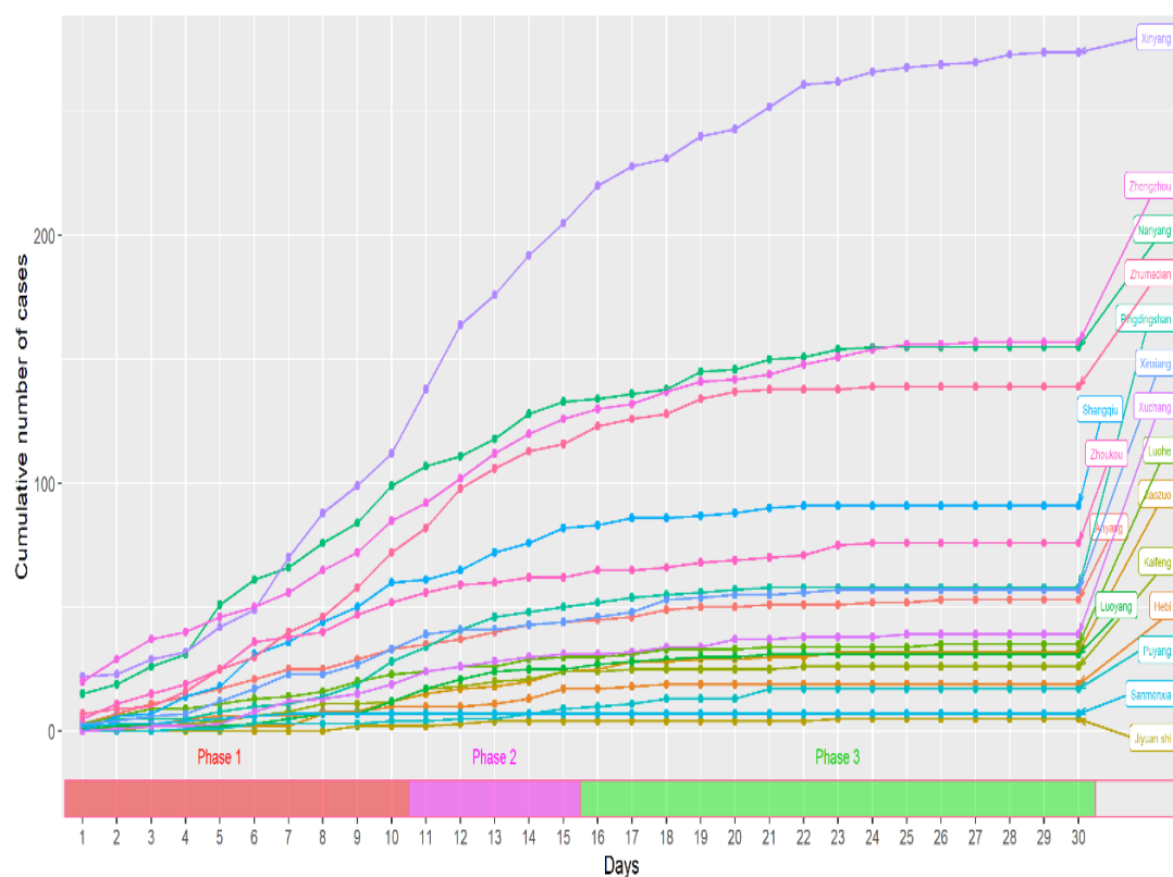
Figure 4(a). Cumulative number of cases for 30 days.
