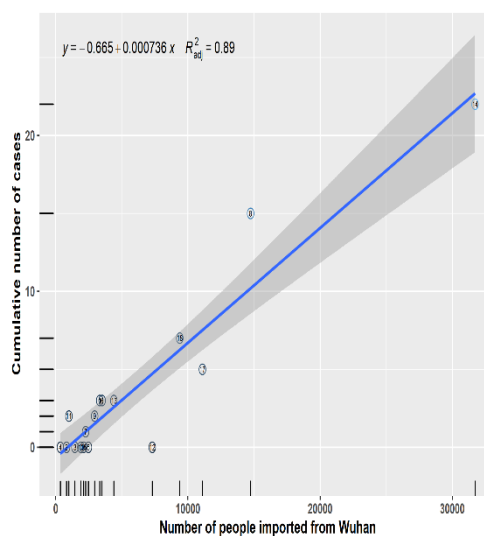
Figure 1(b). 17 cities scatter plot
