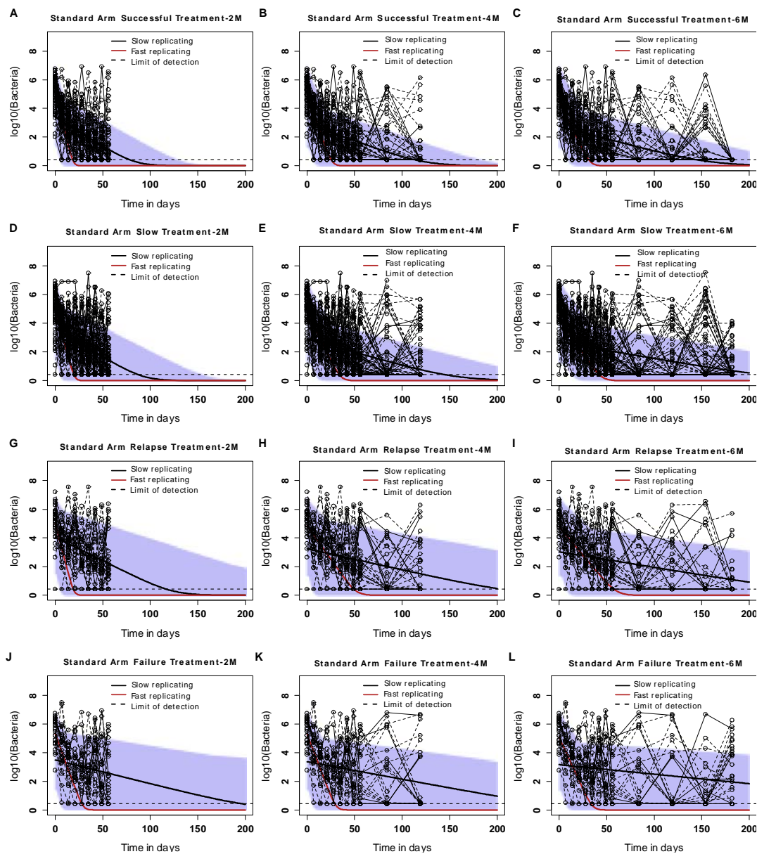
Figure S2. Model fitting to accrued data at 8-weeks, 4-months and 6-months time points. Shown are model fitting to the accrued cure data cluster at 8-weeks/2M (A), 4M (B) and 6M (C), respectively. Model fitting to the slow successful cure cluster data are shown in D (at 2M), E (at 4M) and F (at 6M). Relapsing disease data patterns are given in G, H, and I and while treatment failure are shown in J, K and L at 2M, 4M and 6M,
