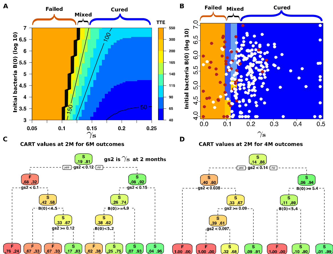
Figure S4. Biomarker characterization in indeterminate data zones. Thresholds for
