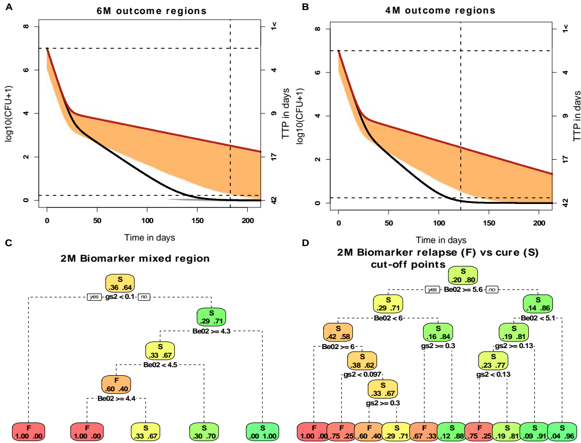
Figure S5. Thresholds for regions with mixed outcomes. \gamma_2 values greater than 0.125 cure patients with initial bacteria burden between 4-6 \log_{10}\text{CFU}/\text{mL} and values below 0.125 will result in failure using simulations. (B) illustrates the overlap between the initial bacteria and the slopes for the 4-month outcomes. In A and B regions of failure are shaded orange and the cure region has the grey shading). (C) CART derived cut-off values for 6 months outcomes. (D) CART derived predictor (initial burden and \gamma_2 -slope) cut-off to delineate relapses from cure.
