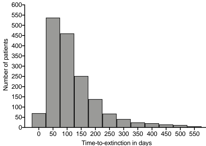
Fig 2. Distribution of time-to-extinction for all 1,924 patients. Shown is the data for all the 1,646 patients who achieved bacillary population extinction; bacilli in the remainder of patients did not reach extinction, so the time is at infinity. The mean time to extinction and 95% confidence intervals were 122.4 [117.9 to 126.9] days.
