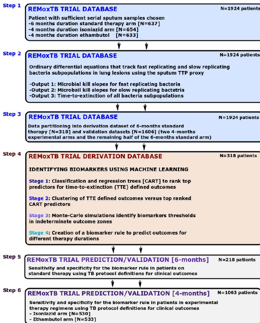
Figure 1. Biomarker Development Steps. Step 1: Patients without sufficient data points to derive bacterial kill slopes were removed. Step 2: The weekly sputum time-to-positivity data was then converted to colony forming units and modeled using ordinary differential equations. Step 3: Data partitioning of 50% of patients in standard of care six-months therapy as derivation data-set and the other 50% into validation dataset. All patients in experimental arm, administered over 4 months were assigned to validation datasets. Step 4: Four mathematical modeling and machine learning types of analysis in derivation dataset to [1] identify predictors of time-to-extinction [TTE] and [2] threshold values delimiting different TTE, and [3] design a diagnostic rule for different therapy durations. Step 5: Accuracy of diagnostic rule/biomarker for six-months therapy duration in standard of care validation dataset using clinical definitions of outcome [relapse, cure]. Step 6: Accuracy of diagnostic rule/biomarker for four-months therapy duration in two experimental arms in validation dataset using clinical definitions of relapse and cure.
