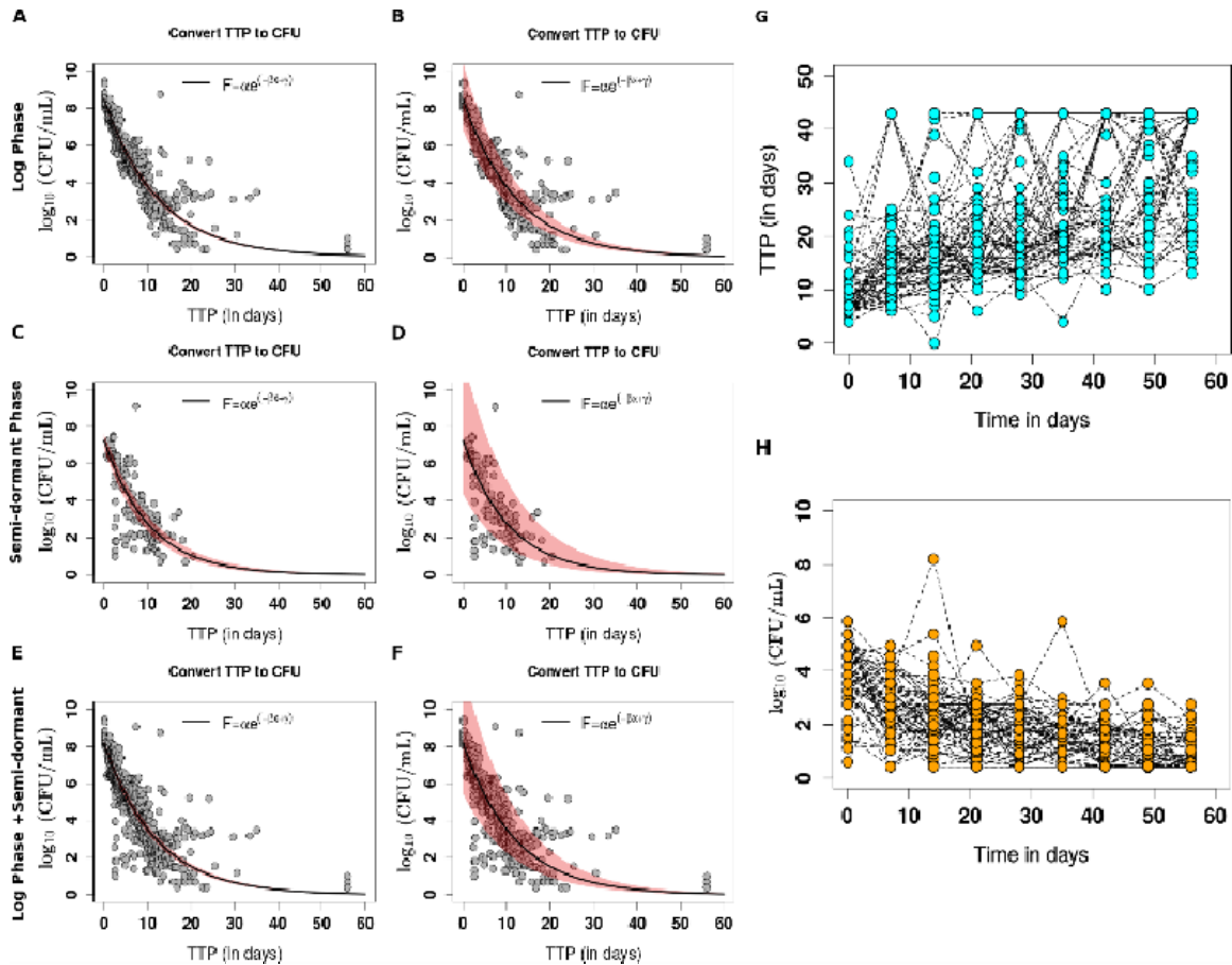
Figure S1. Converting TTP to CFU and vice-versa. Illustrating conversion of serial TTP values from patients to corresponding CFU values. Panels A showing model function correlating TTP to CFU, here the model has two parameters to the estimated, in B the model with three parameters has wider uncertainty. While conversion for bacteria in log phase is shown in A and B , conversion for slow (non replicating) replicating bacteria is shown in C and D , then in panels E and F , combined subpopulations are shown. Panel G shows TTP patient clinical data and the corresponding converted CFU are shown in H at start of therapy [Day 0] and every 7 days till day 56.
