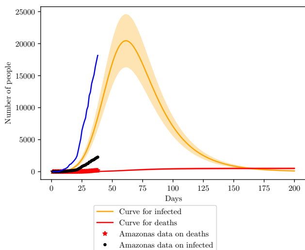
Fig. 18: Simulation of the COVID-19 pandemic crisis on Amazonas.
