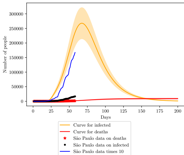
Fig. 15: Simulation of the COVID-19 pandemic crisis on Sao Paulo. The blue curve was shown to represent the 90% loss of data on Sao Paulo considering a constant testing rate.
