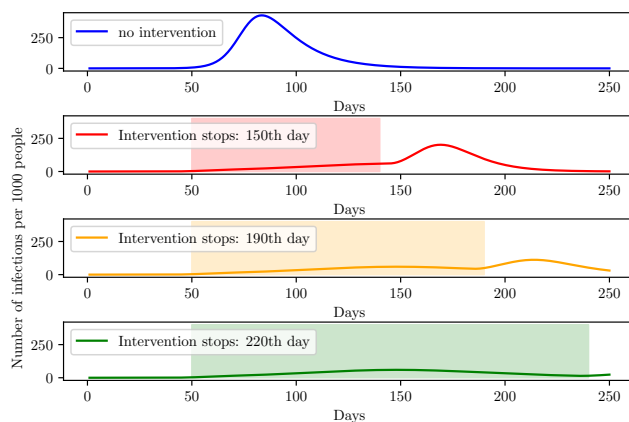
Fig. 20: Height of the second peak for different times on social isolation.
