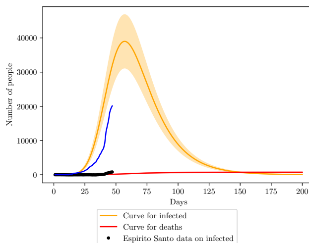
Fig. 11: Simulation of the COVID-19 pandemic crisis on Espirito Santo.
