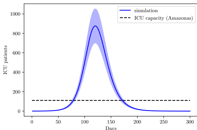
Fig. 19: Simulation of the ICU demand on the state of Amazonas.
