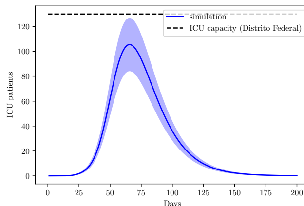
Fig. 14: ICU demand on Distrito Federal due to COVID-19.
