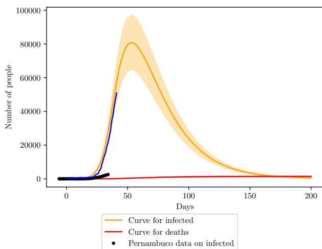
Fig. 9: Simulation of the COVID-19 pandemic crisis on Pernambuco. The blue curve shows the behavior of the data considering 90% loss of infections.
