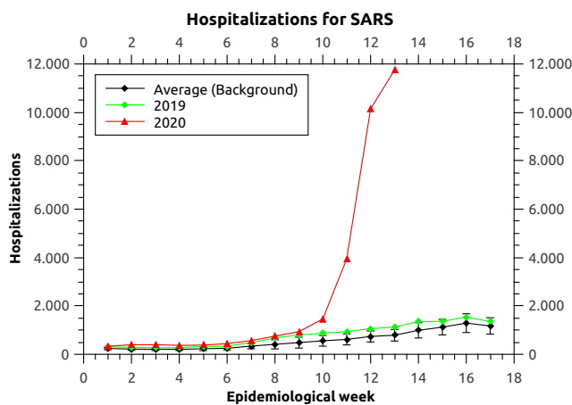
Fig. 3: Number of hospitalizations by SARS on Brazil on the year of 2020, 2019 and the background average.
