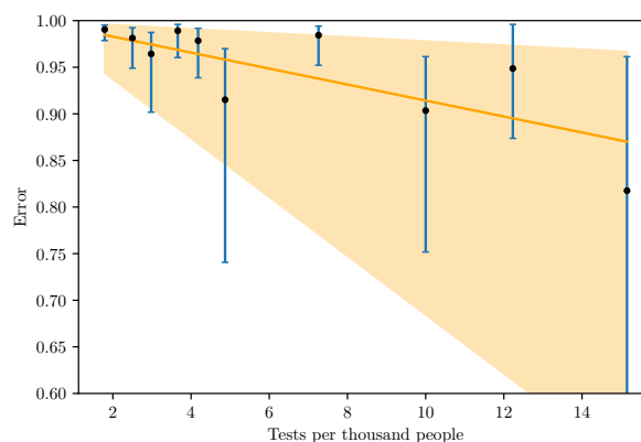
Fig. 5: Relation between the number of tests performed on total per 1000 habitants and the fraction of lost cases.
