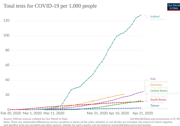
Fig. 7: Total number of tests per 1000 habitants. Graph taken from [19].
