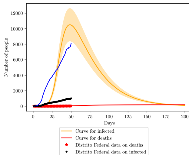
Fig. 13: COVID-19 scenario for Distrito Federal. Blue curve represents the behavior of data considering 86% loss of infections.
