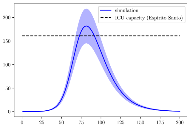
Fig. 12: Simulation of the ICU population on Espirito Santo due to COVID-19. Blue curve represents data following the 88% of undocumented infections.
