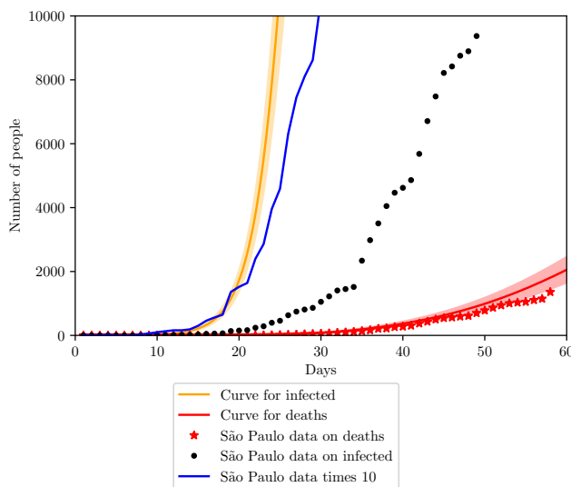
Fig. 16: Simulation of the COVID-19 pandemic crisis on Sao Paulo on most recent days.
