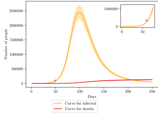
Fig. 8: Simulation of the COVID-19 pandemic crisis on Brazil.
