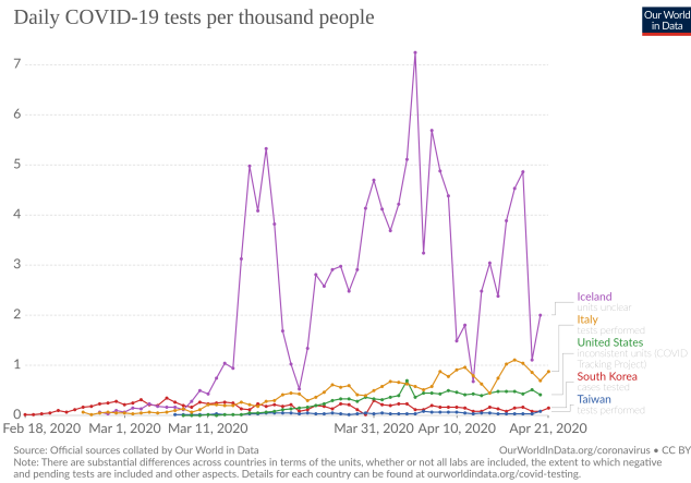
Fig. 6: Tests Per Day Per 1000 habitants. Taken from [19].
