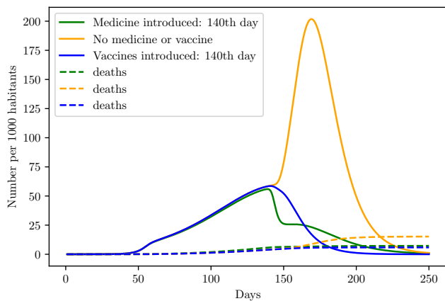
Fig. 22: Behavior of the infection curve if the vaccination/medication occurs 10 days before time of intervention stopping.
