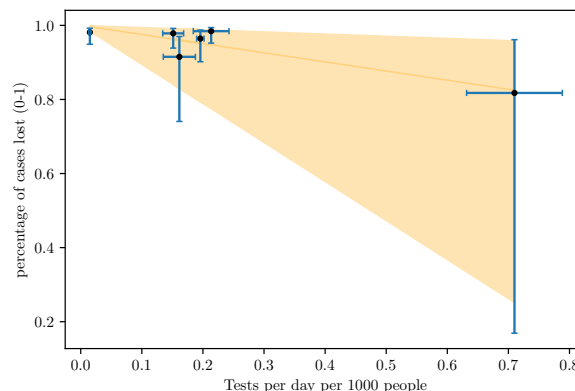
Fig. 4: Relation between the number of tests performed per day per 1000 habitants and the fraction of lost cases.
