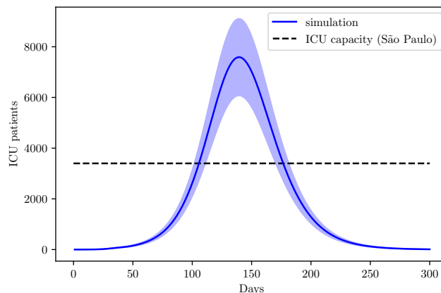
Fig. 17: Simulation of the ICU demand on the state of Sao Paulo.
