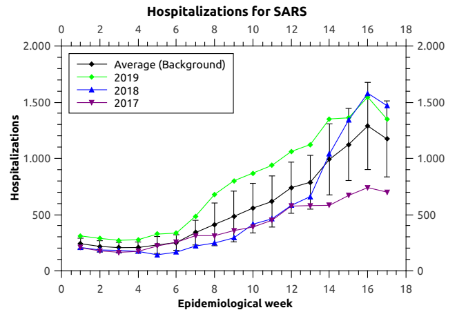
Fig. 2: Hospitalizations by SARS on Brazil on the years of 2017, 2018 and 2019.
