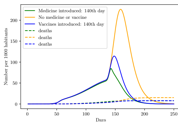
Fig. 21: Behave of the infection curve if the vaccination/medication occurs at the same time of intervention stopping.
