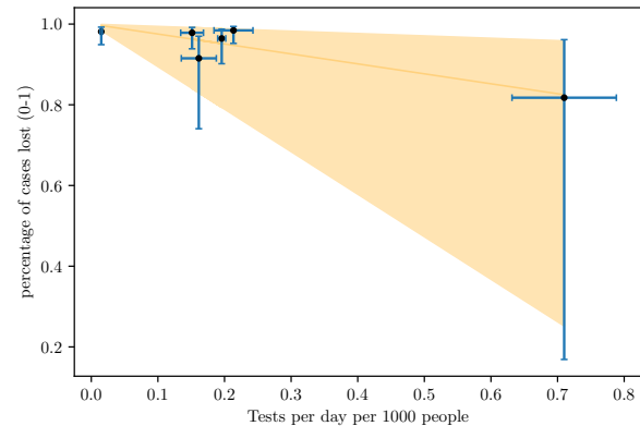
Fig. 4: Relation between the number of tests performed per day per 1000 habitants and the percentage of lost cases.
