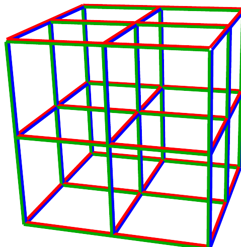
Figure 1: Illustration of sample pooling in the hypercube algorithm, for D = L = 3 and N = 27 . Each lattice point represents an individual. The hypercube is sliced into L slices, in each of the D principal directions, and samples from N/L individuals are pooled into a sample for each slice. For this example, the 3 sets of slices are shown in blue, red and green. If one infected individual is present, tests on each set of slices identify their coordinate in that direction. Hence only 9 tests would uniquely identify them. As the viral prevalence falls, the optimal group size N and dimension D grow, and the efficiency gain rises.
