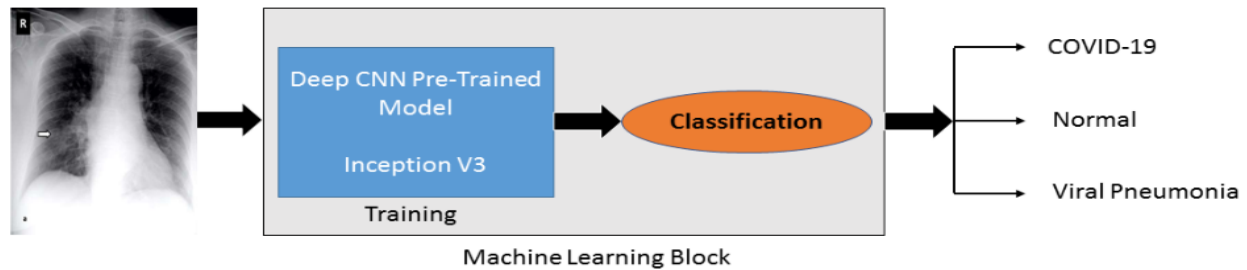
Fig. 4. Schematic representation of pre-trained model for the prediction of COVID-19 patients, normal and viral pneumonia.
