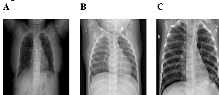
Fig. 1. Example chest radiography images of: (A) COVID-19 Viral Infection (B) Non COVID-19 infection (C) Viral Pneumonia
