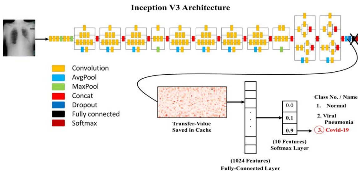
Fig. 2. Transfer learning on the Inception-v3 model
